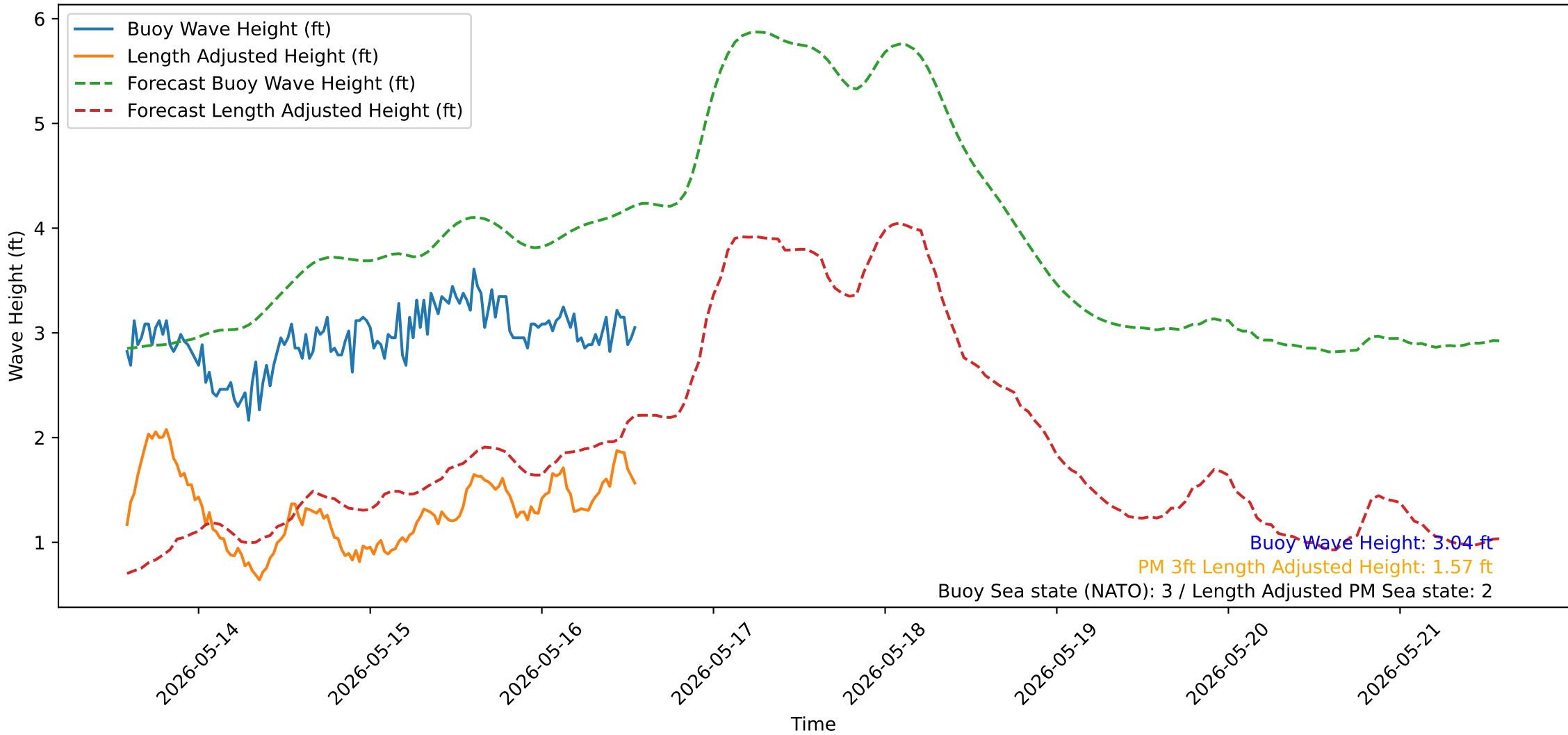
Wave Heights over Time for Oceanside Harbor at 2026-05-16 13:50:32
