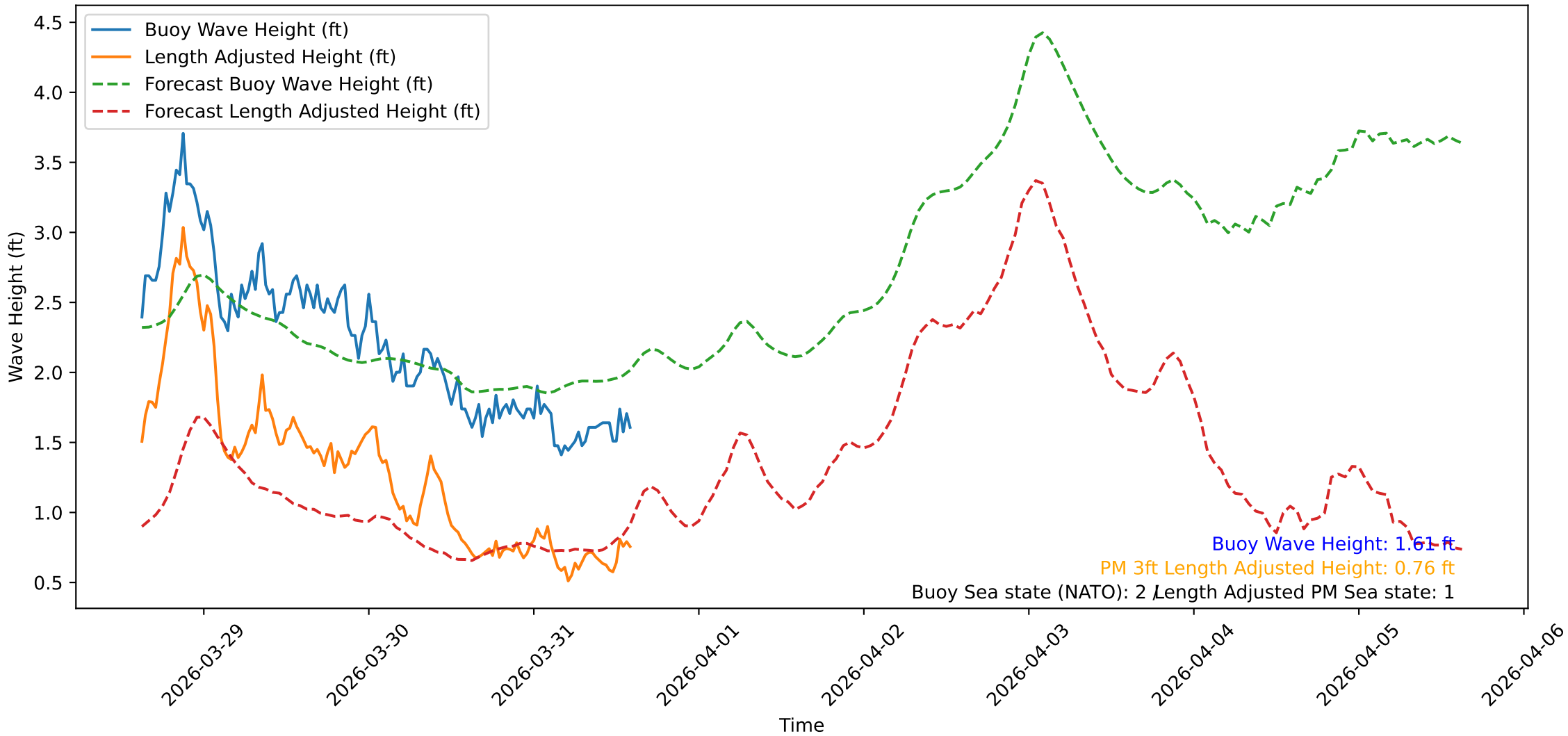
Wave Heights over Time for Green Beach at 2026-03-31 15:01:10
