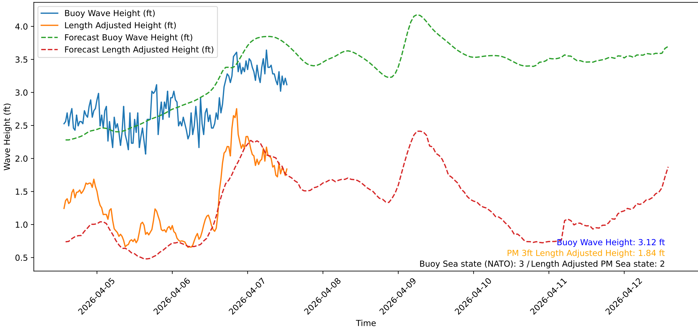
Wave Heights over Time for Oceanside Harbor at 2026-04-07 13:40:32
