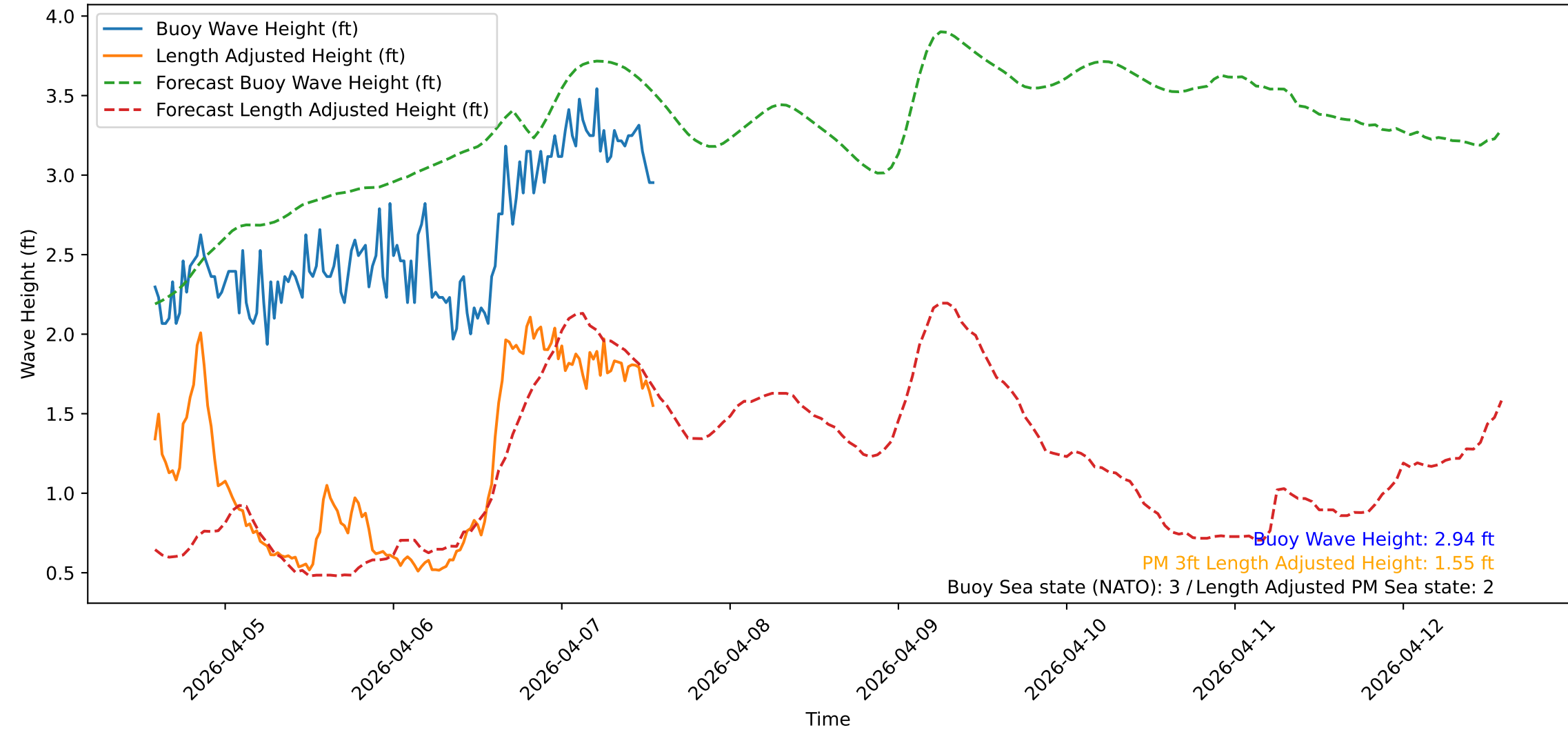
Wave Heights over Time for Red Beach at 2026-04-07 13:40:48
