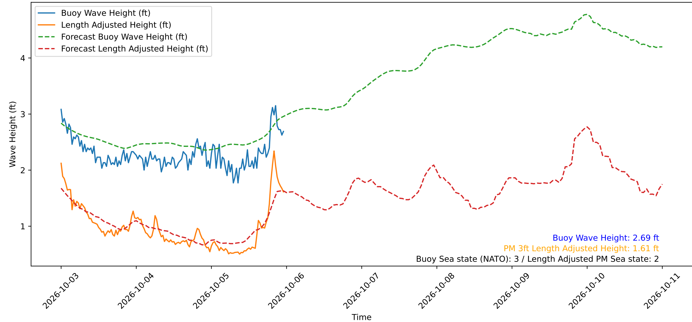
Wave Heights over Time for Green Beach at 2026-10-05 23:41:12
