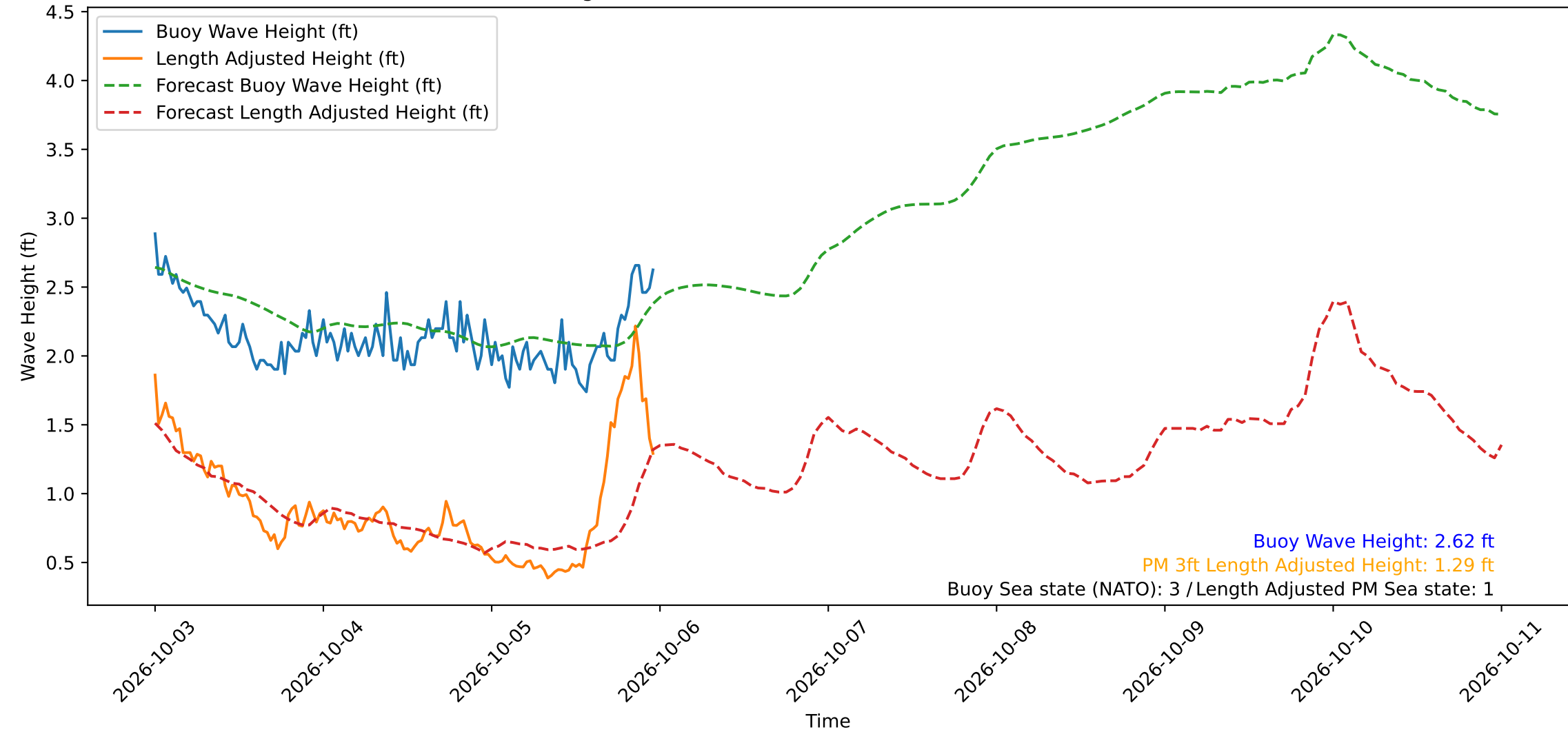
Wave Heights over Time for Red Beach at 2026-10-05 23:40:49
