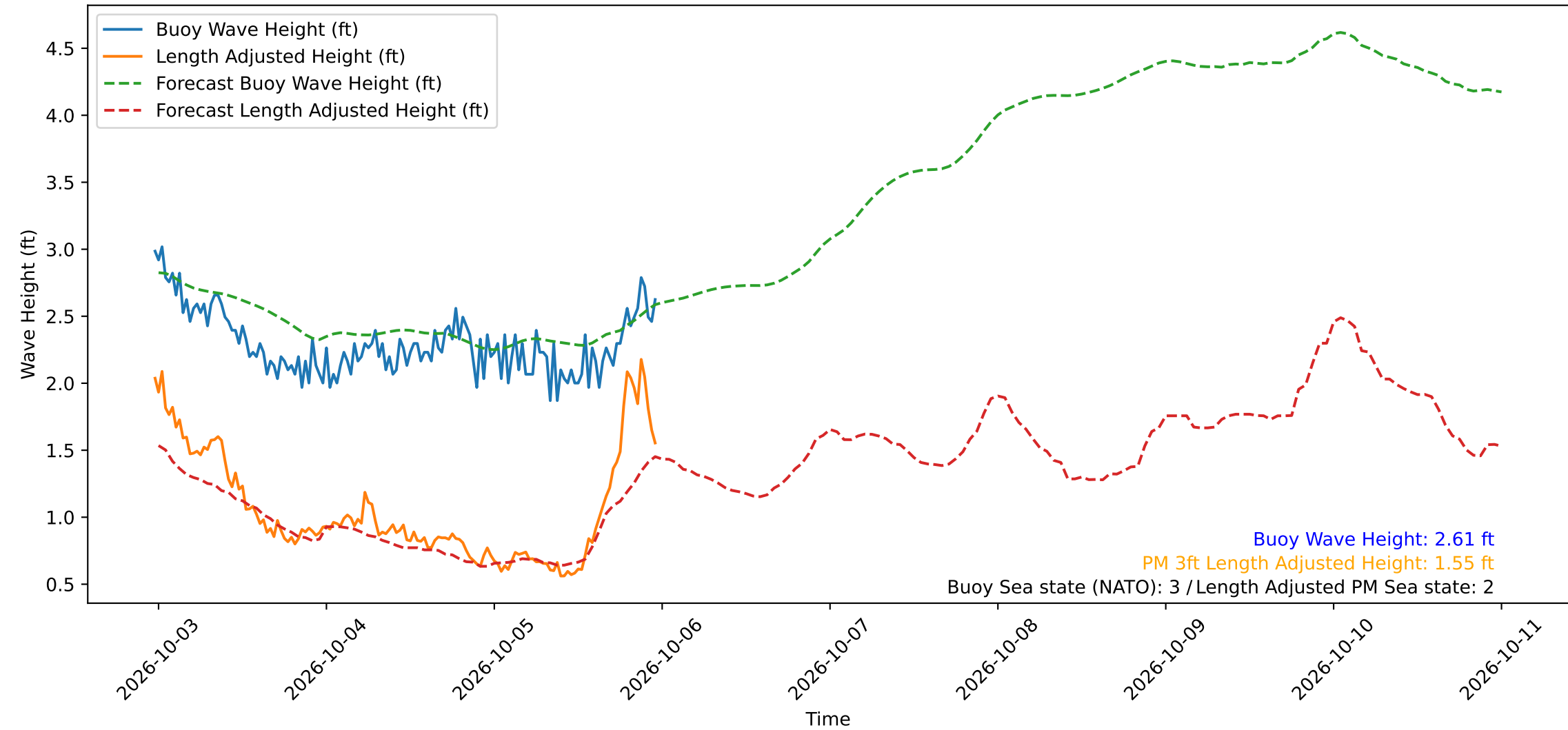
Wave Heights over Time for Oceanside Harbor at 2026-10-05 23:40:30
