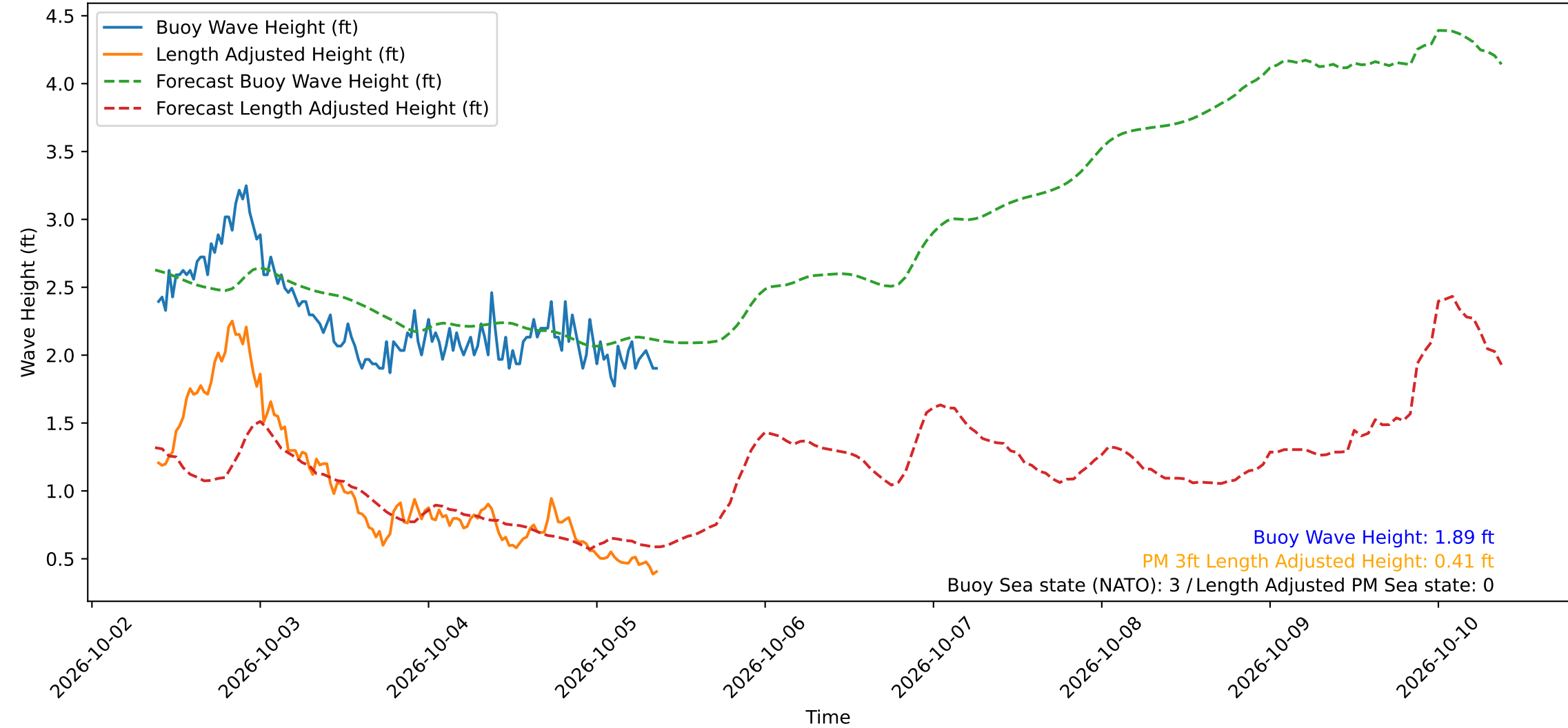
Wave Heights over Time for Red Beach at 2026-10-05 09:10:49
