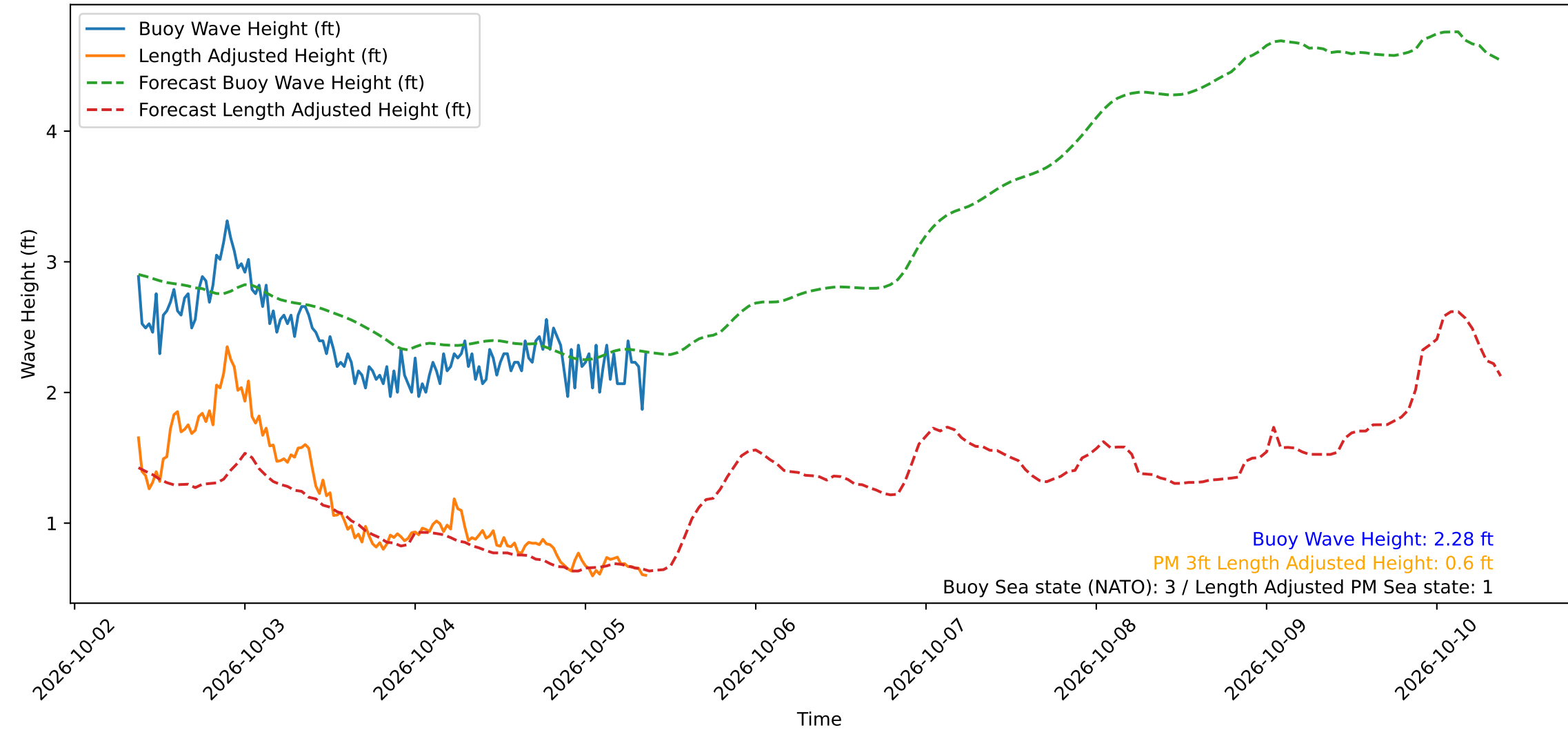
Wave Heights over Time for Oceanside Harbor at 2026-10-05 09:10:29
