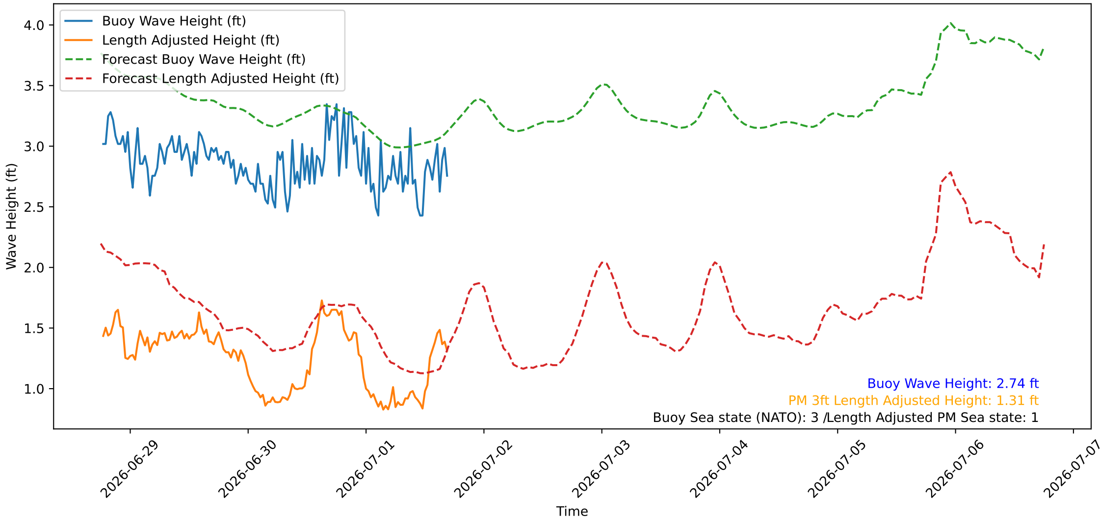
Wave Heights over Time for Red Beach at 2026-07-01 18:00:44
