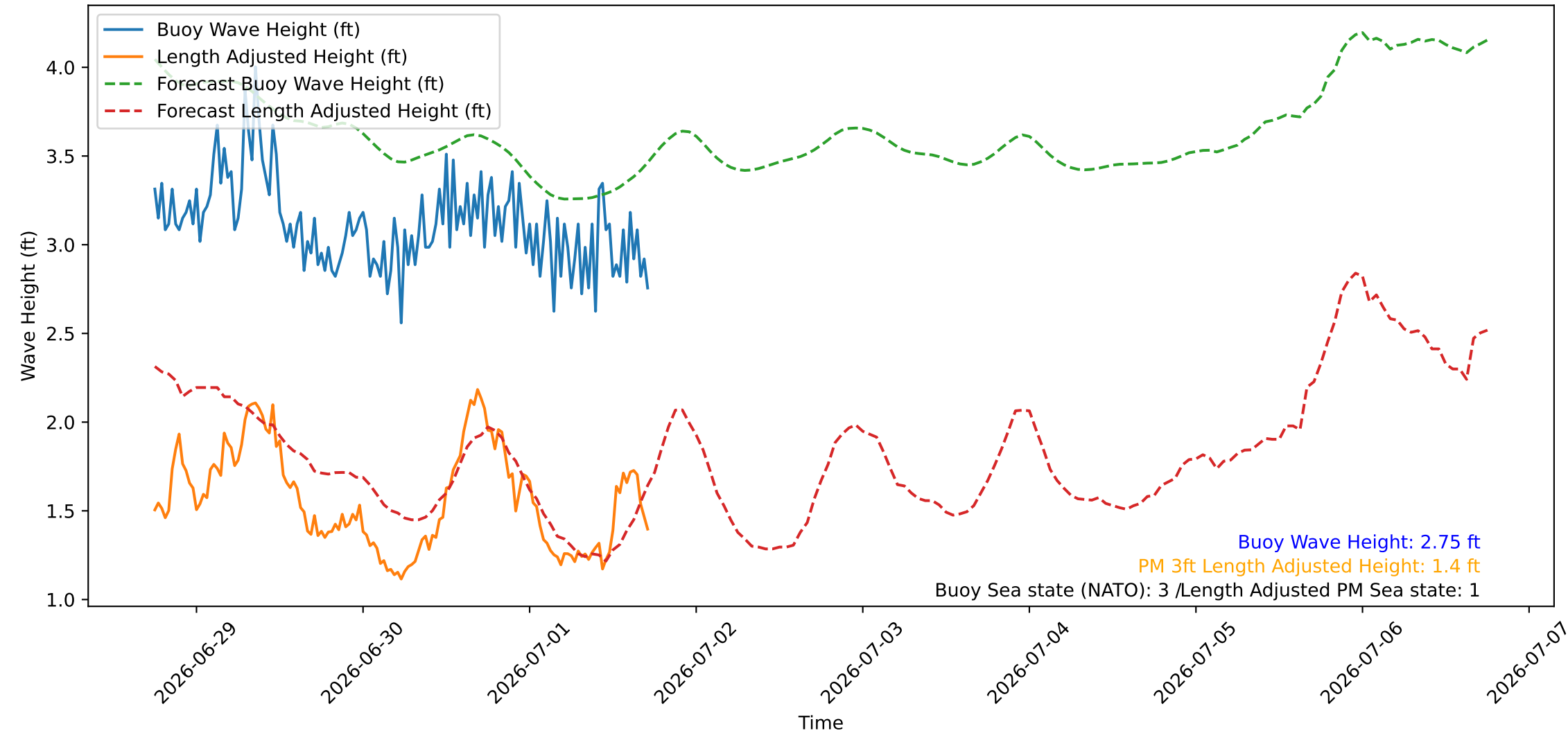
Wave Heights over Time for Oceanside Harbor at 2026-07-01 18:00:25
