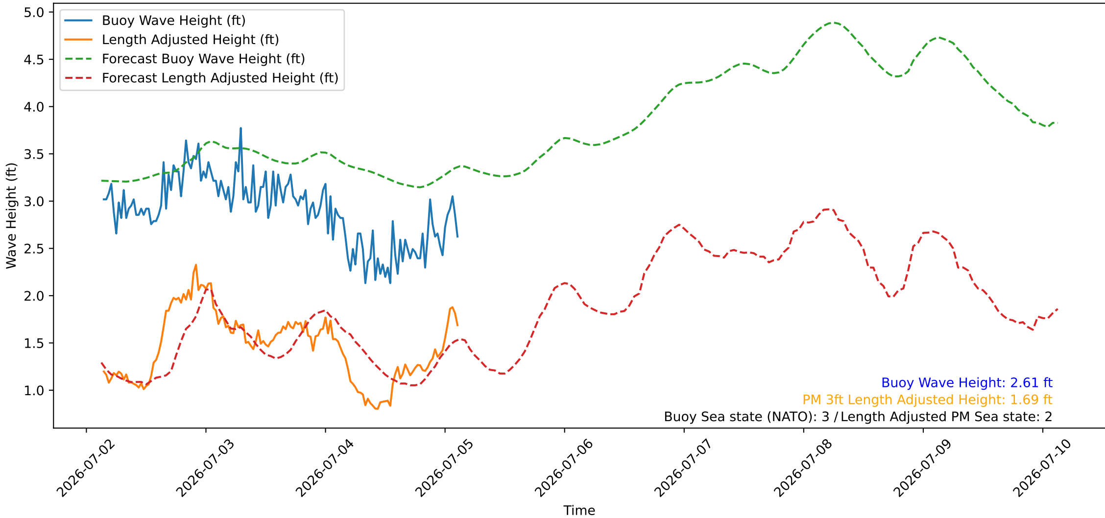
Wave Heights over Time for Oceanside Harbor at 2026-07-05 03:20:27
