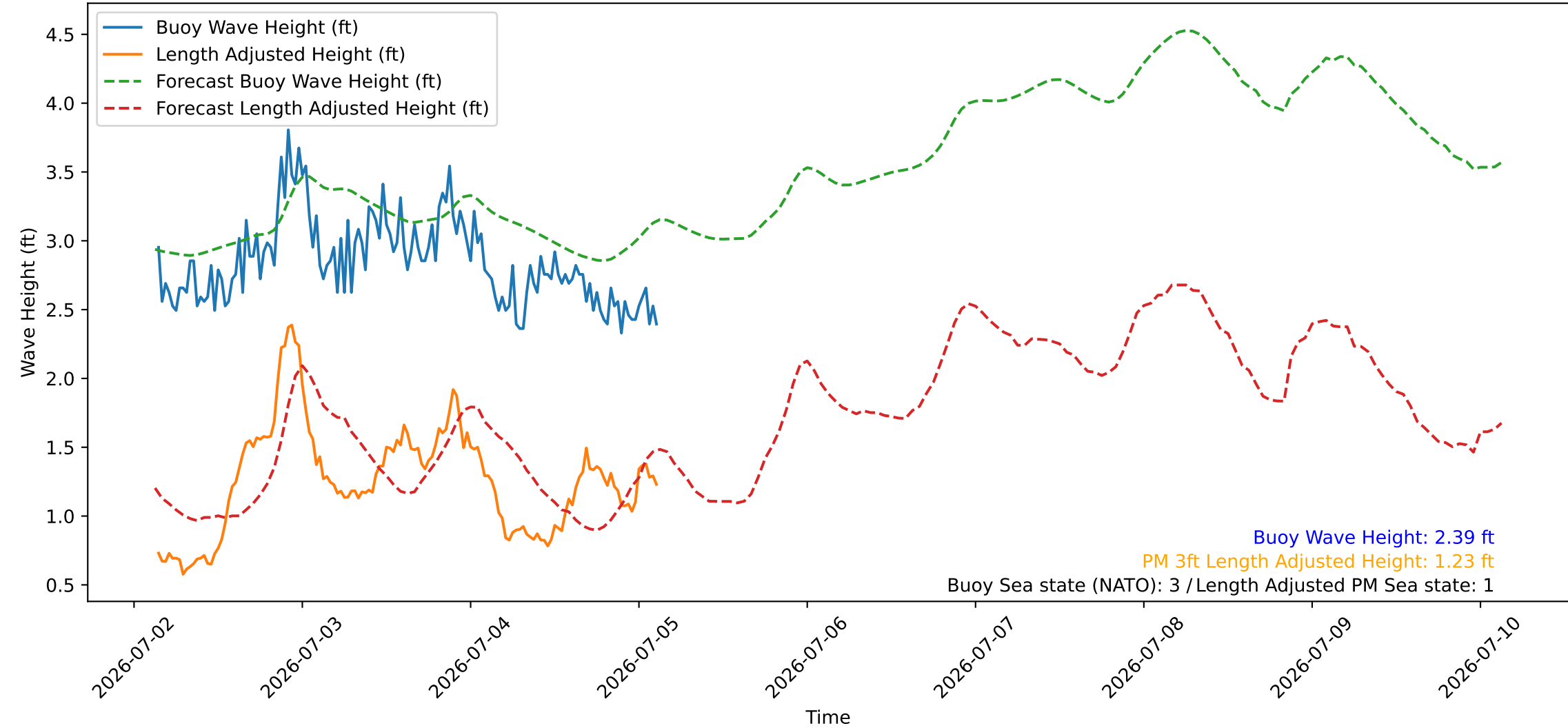
Wave Heights over Time for Red Beach at 2026-07-05 03:20:47
