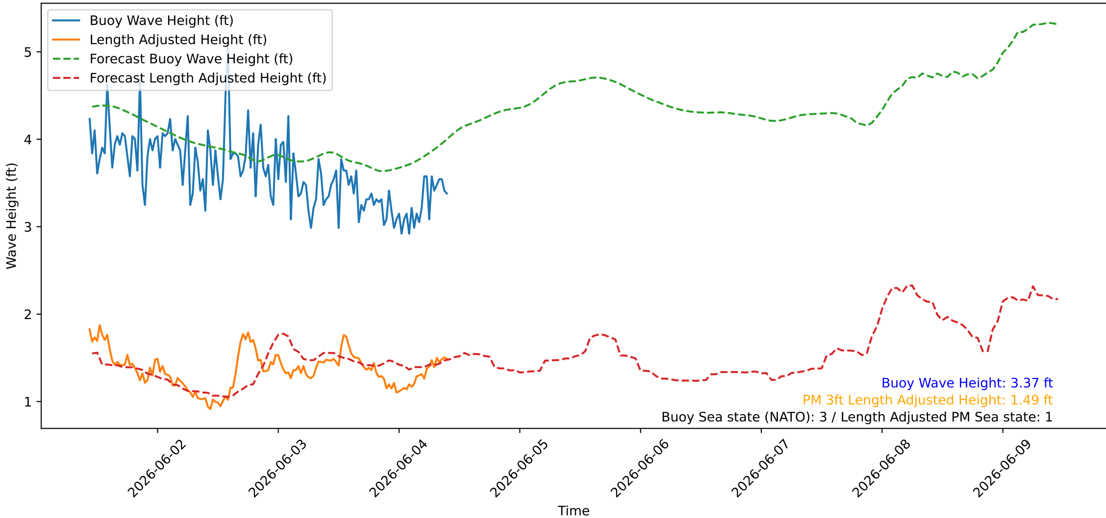
Wave Heights over Time for Oceanside Harbor at 2026-06-04 10:40:25
