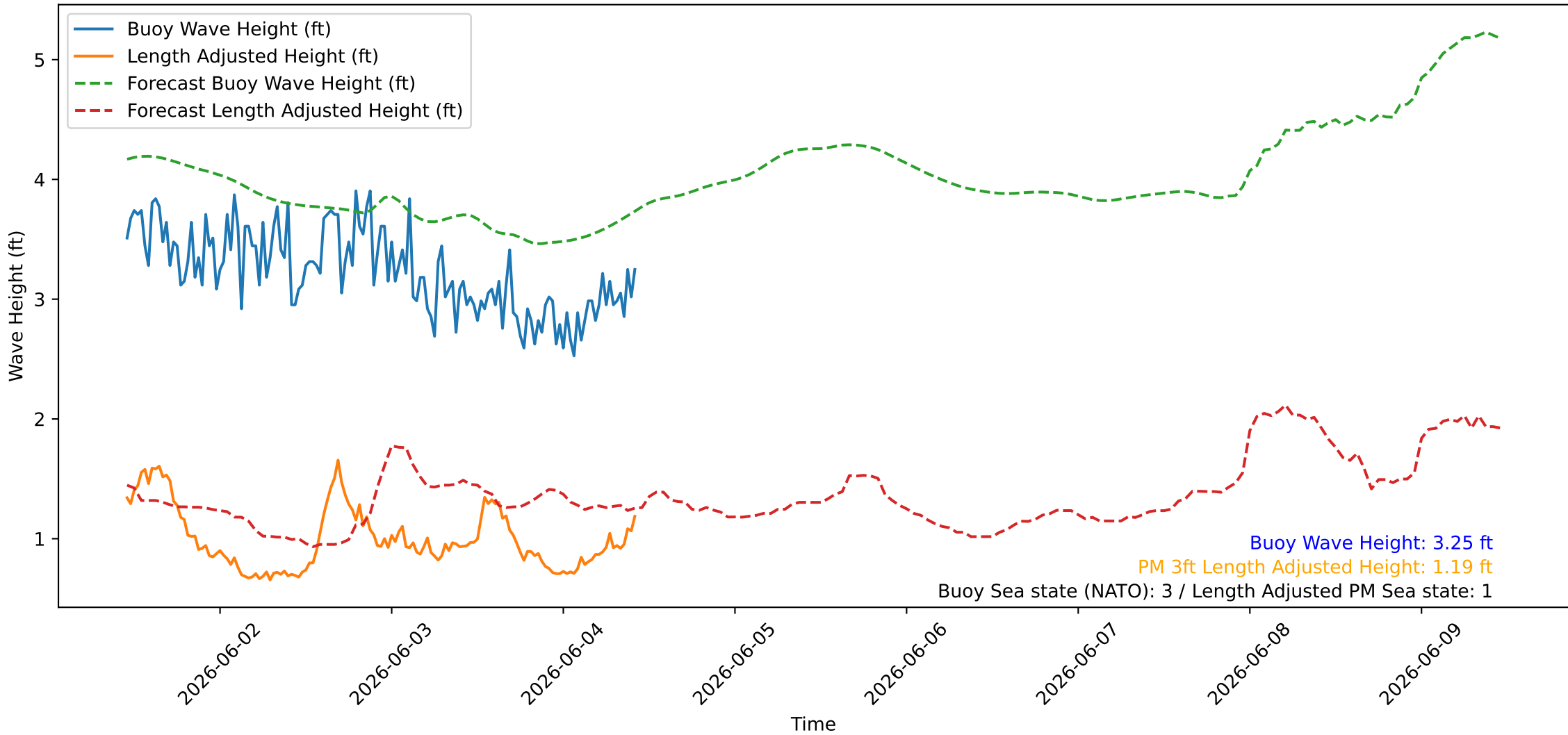
Wave Heights over Time for Red Beach at 2026-06-04 10:40:45
