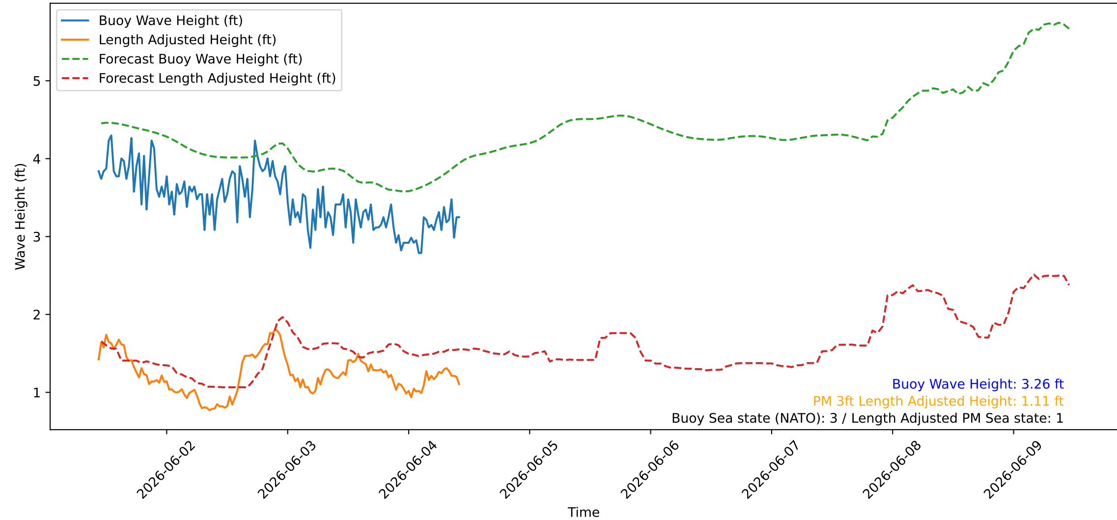
Wave Heights over Time for Green Beach at 2026-06-04 10:41:07
