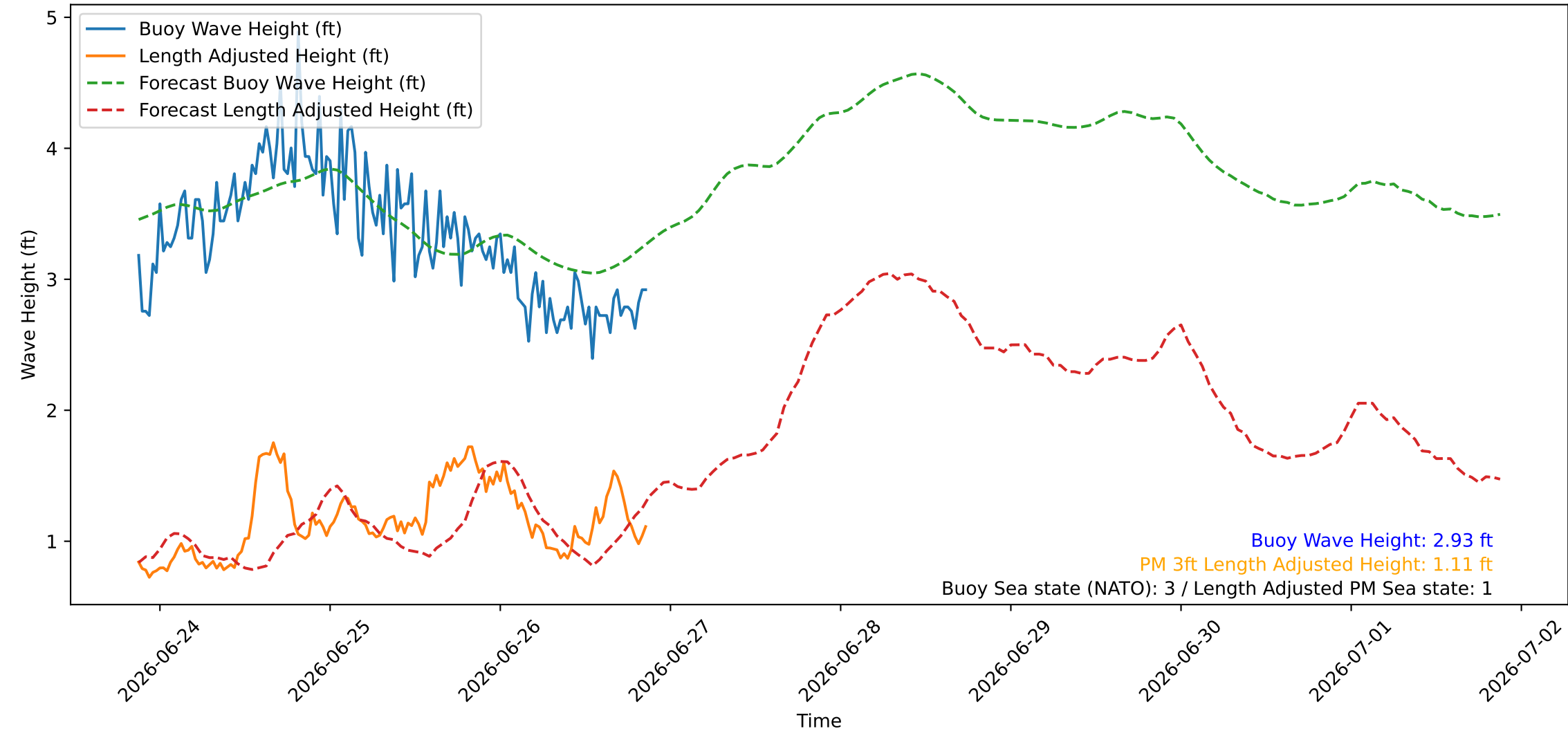
Wave Heights over Time for Oceanside Harbor at 2026-06-26 21:10:26
