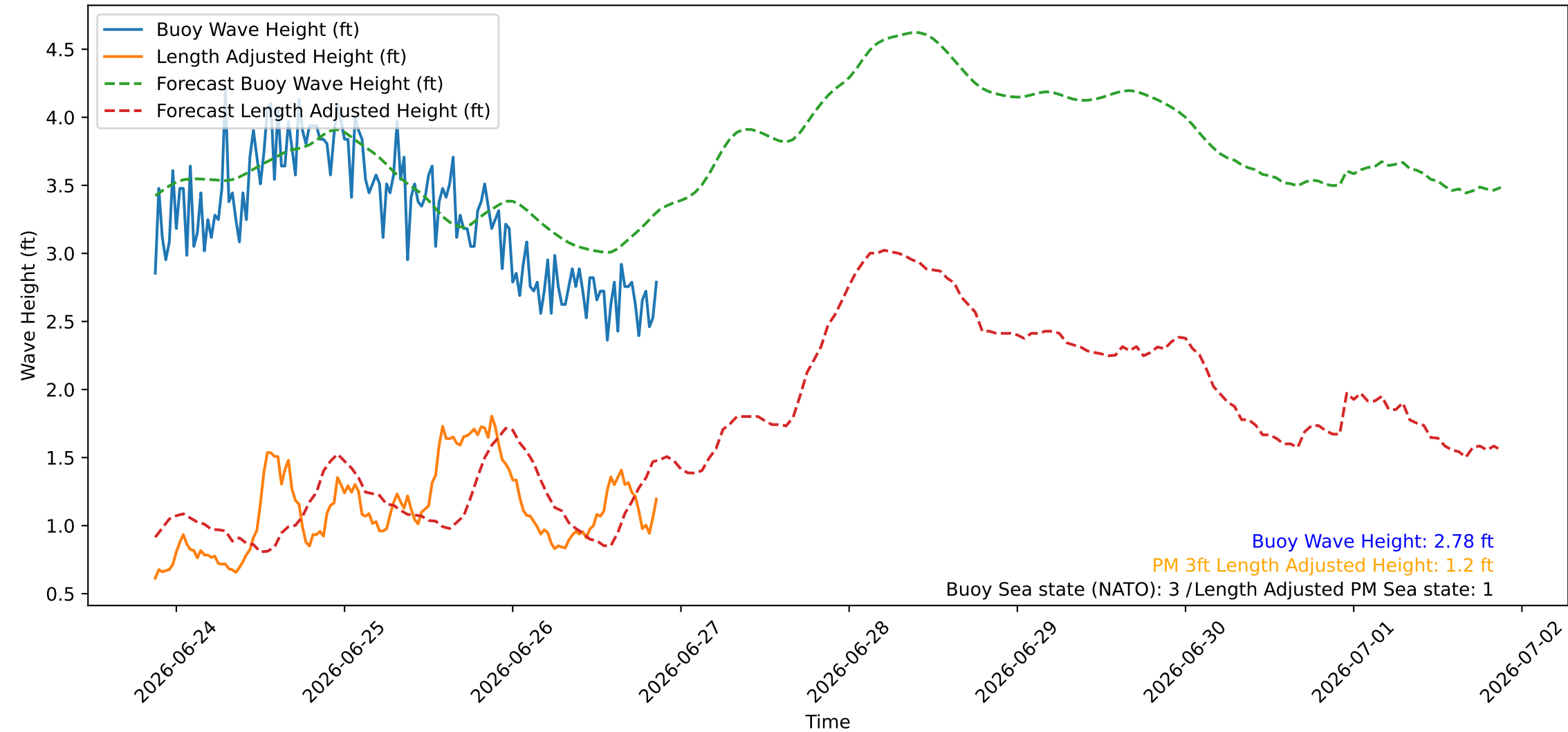
Wave Heights over Time for Green Beach at 2026-06-26 21:11:08
