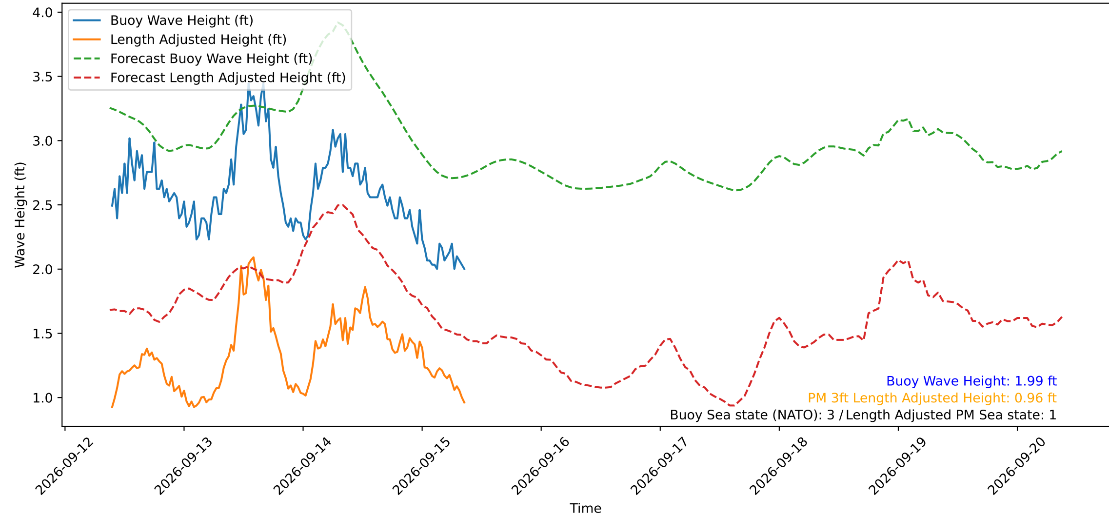
Wave Heights over Time for Red Beach at 2026-09-15 09:20:51
