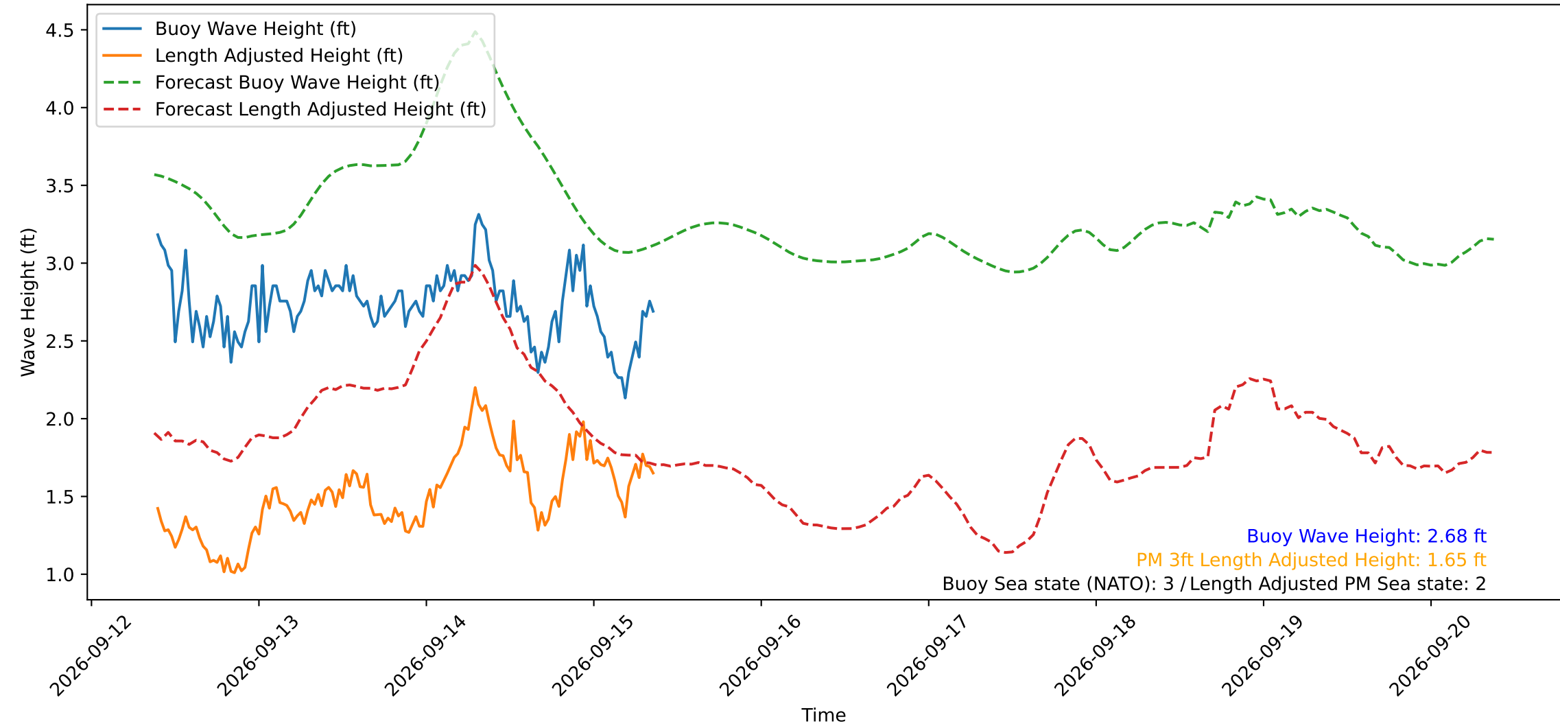
Wave Heights over Time for Green Beach at 2026-09-15 09:21:15
