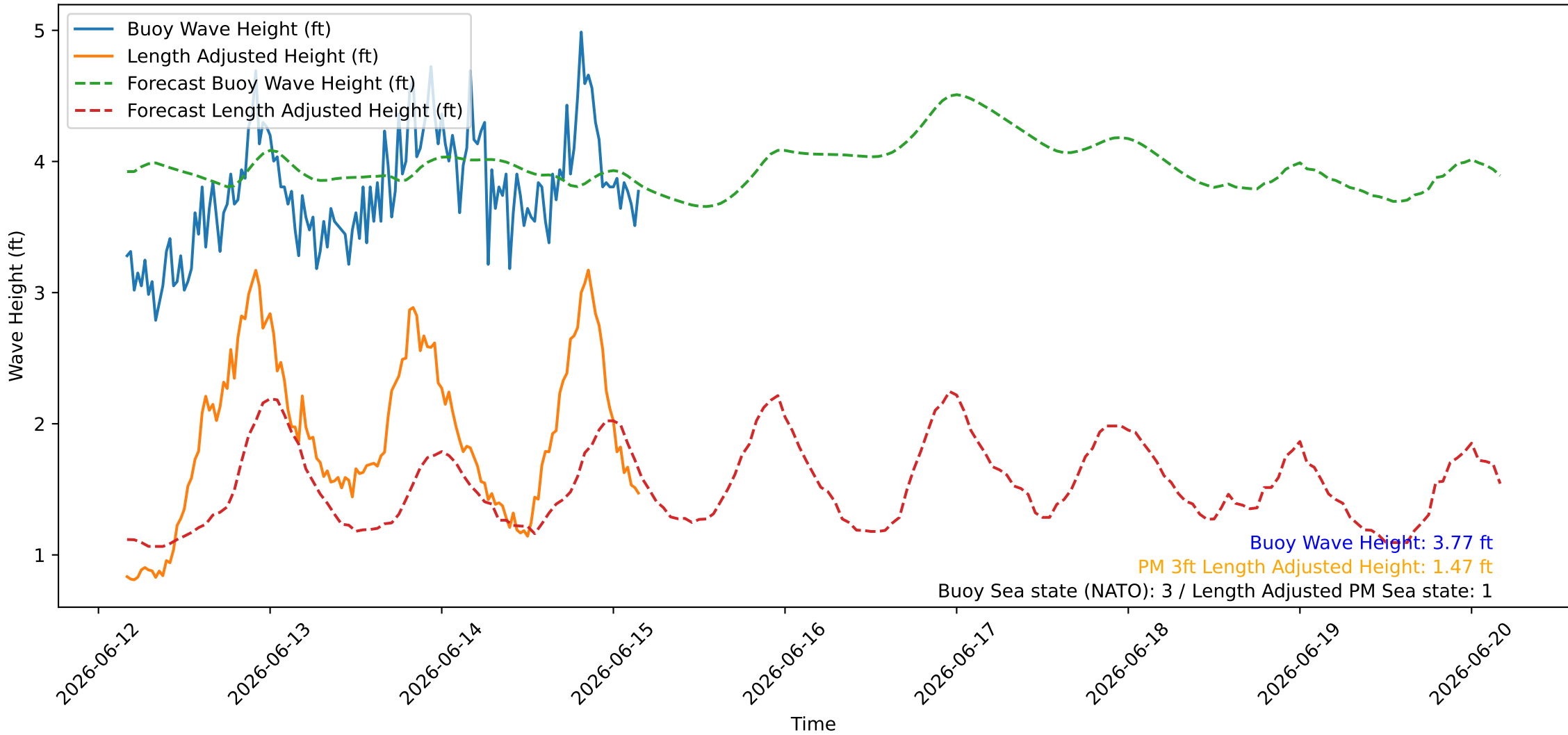
Wave Heights over Time for Oceanside Harbor at 2026-06-15 04:10:25
