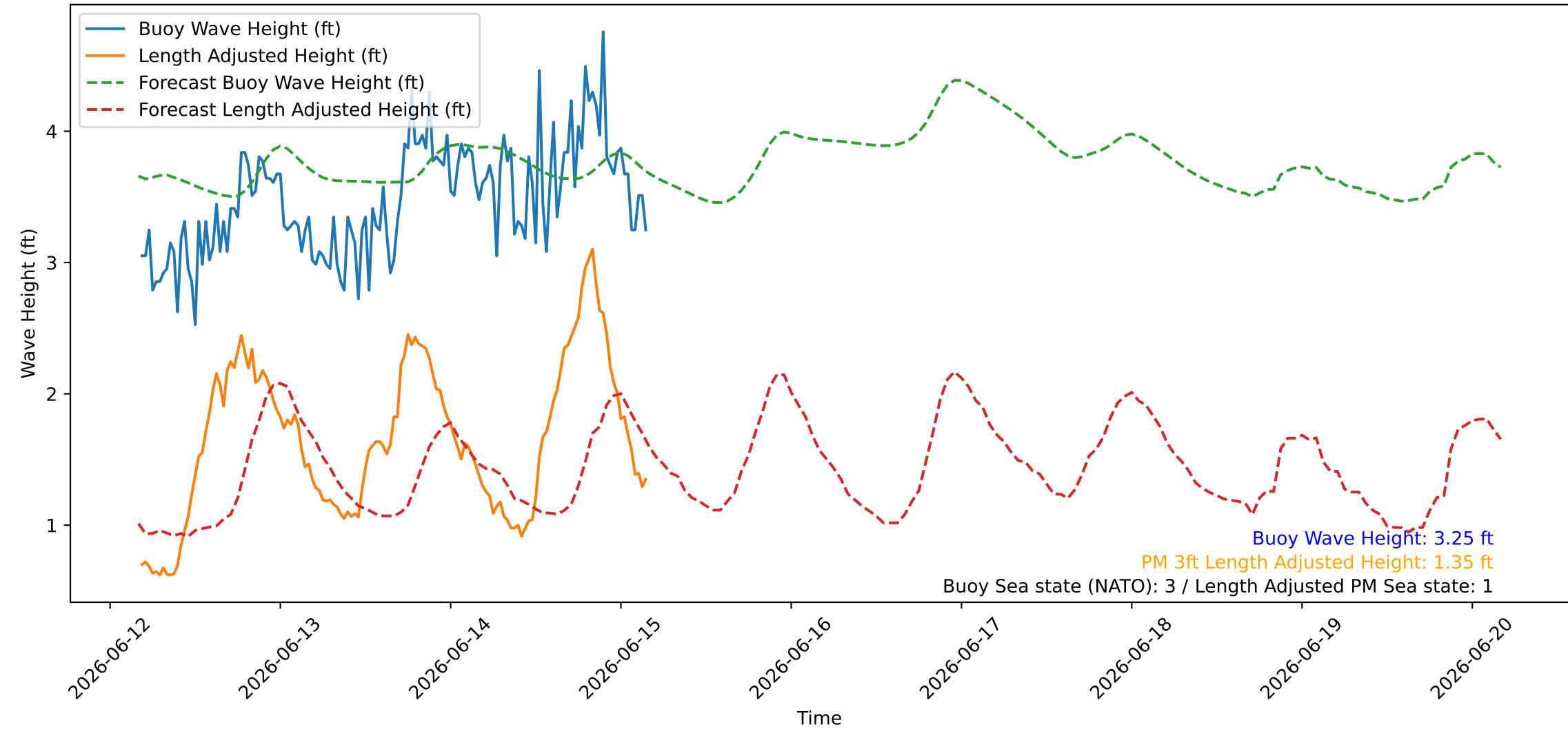
Wave Heights over Time for Red Beach at 2026-06-15 04:10:45
