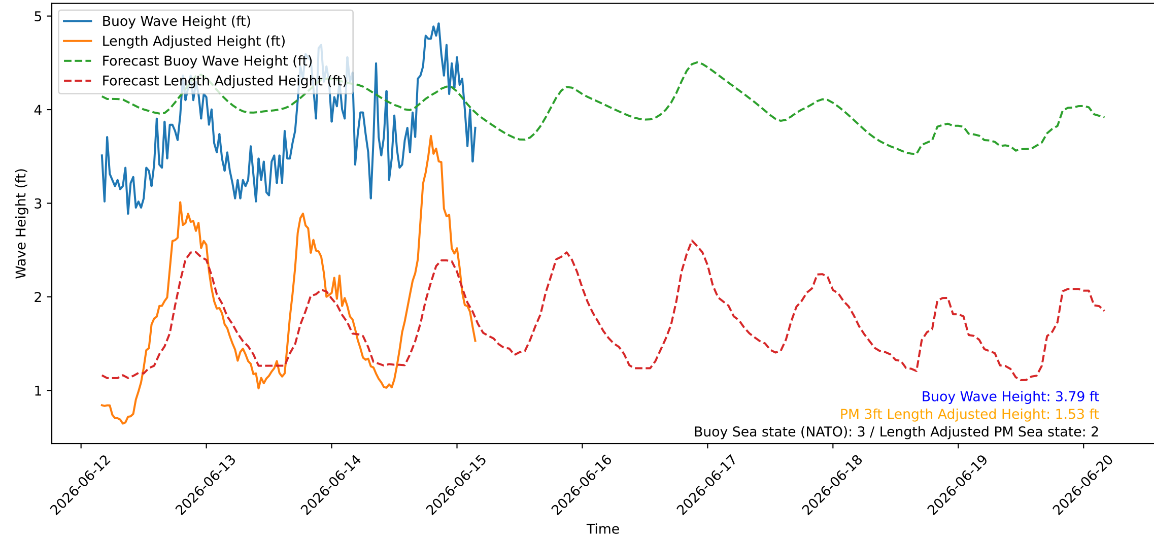
Wave Heights over Time for Green Beach at 2026-06-15 04:11:07
