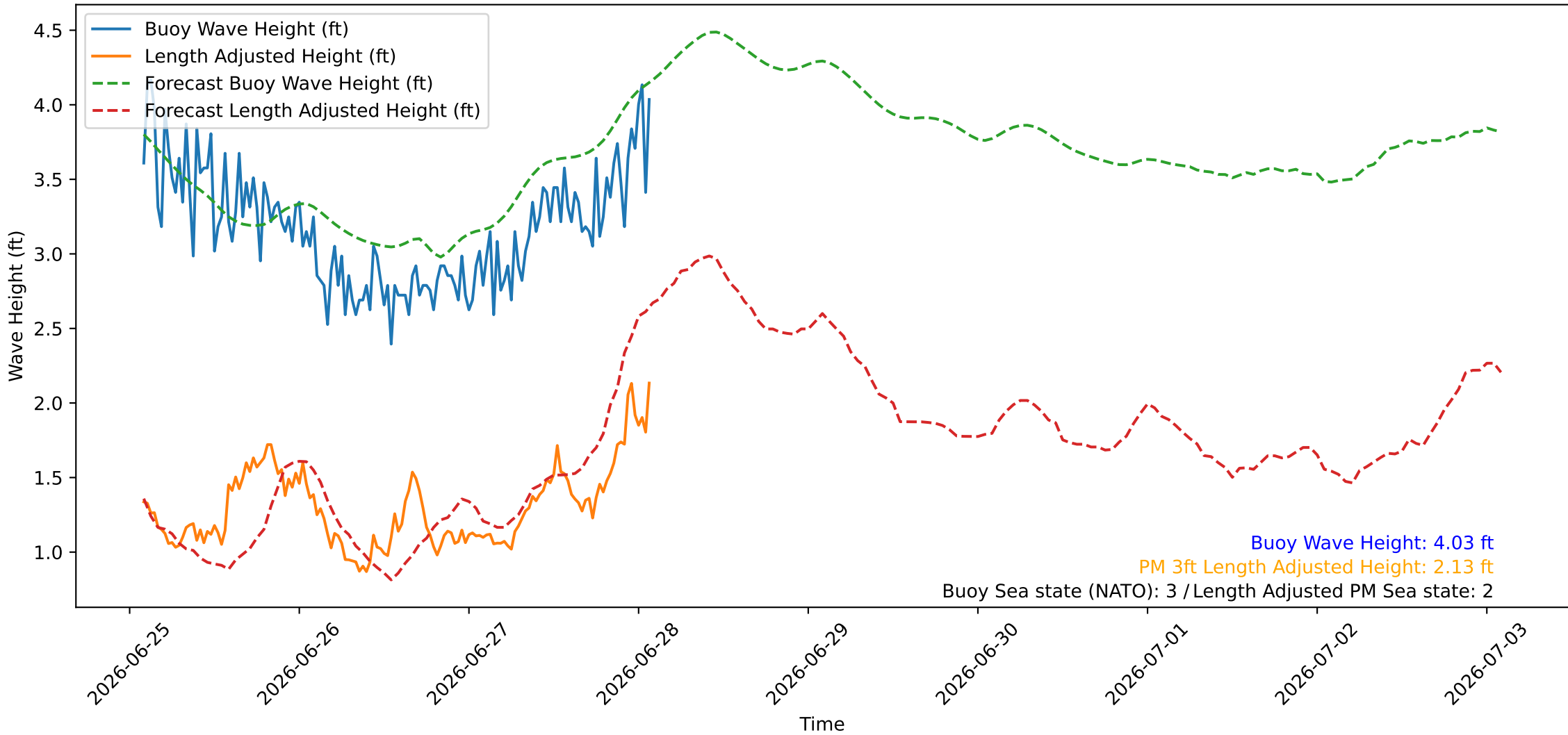
Wave Heights over Time for Oceanside Harbor at 2026-06-28 02:10:26
