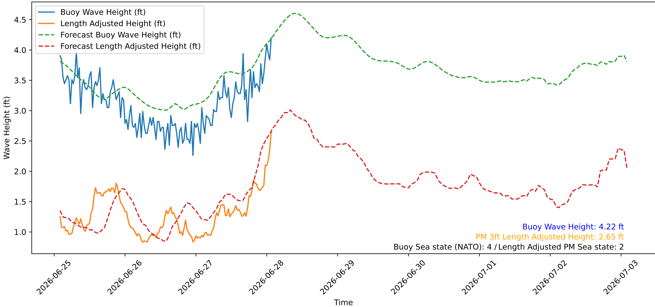
Wave Heights over Time for Green Beach at 2026-06-28 02:11:07
