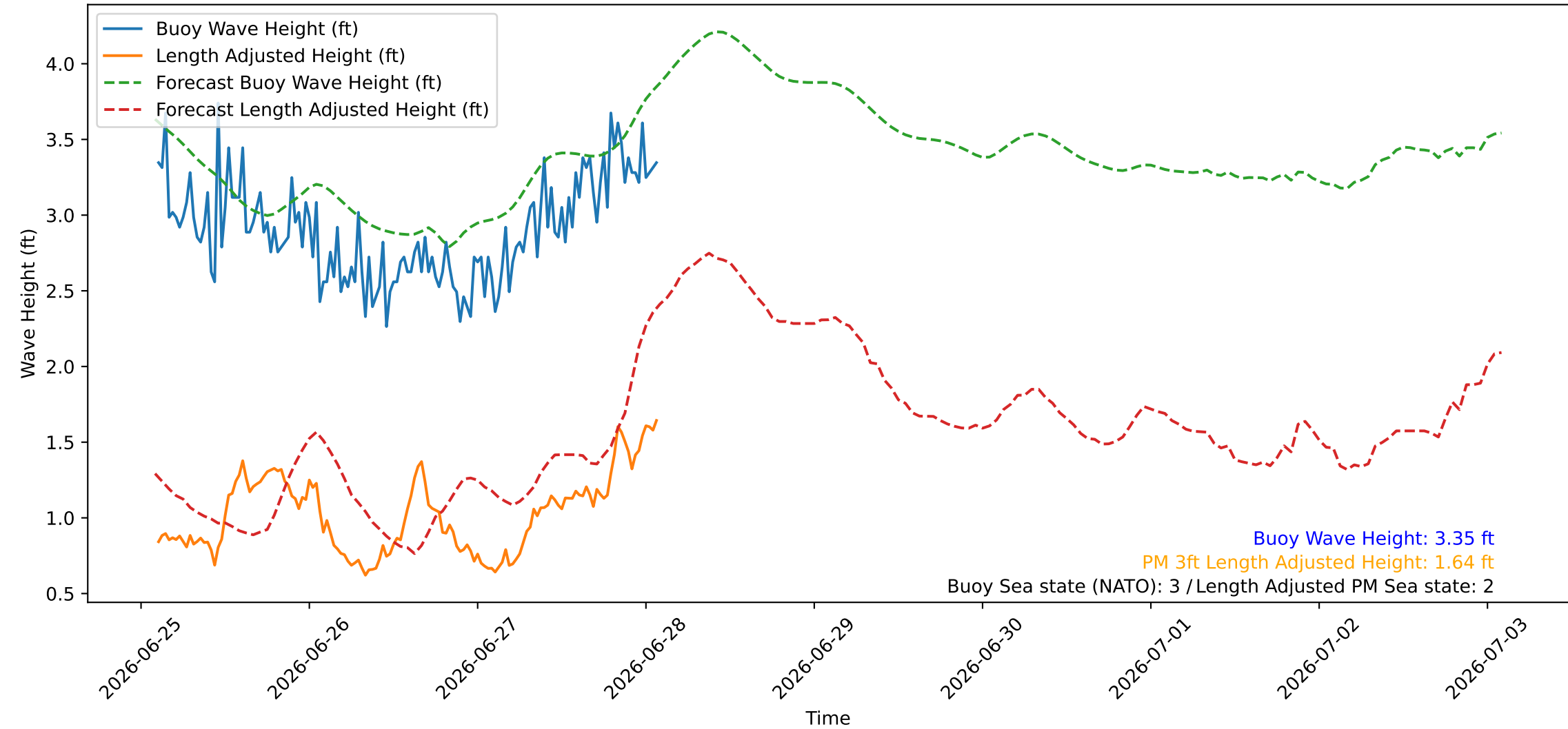
Wave Heights over Time for Red Beach at 2026-06-28 02:10:45
