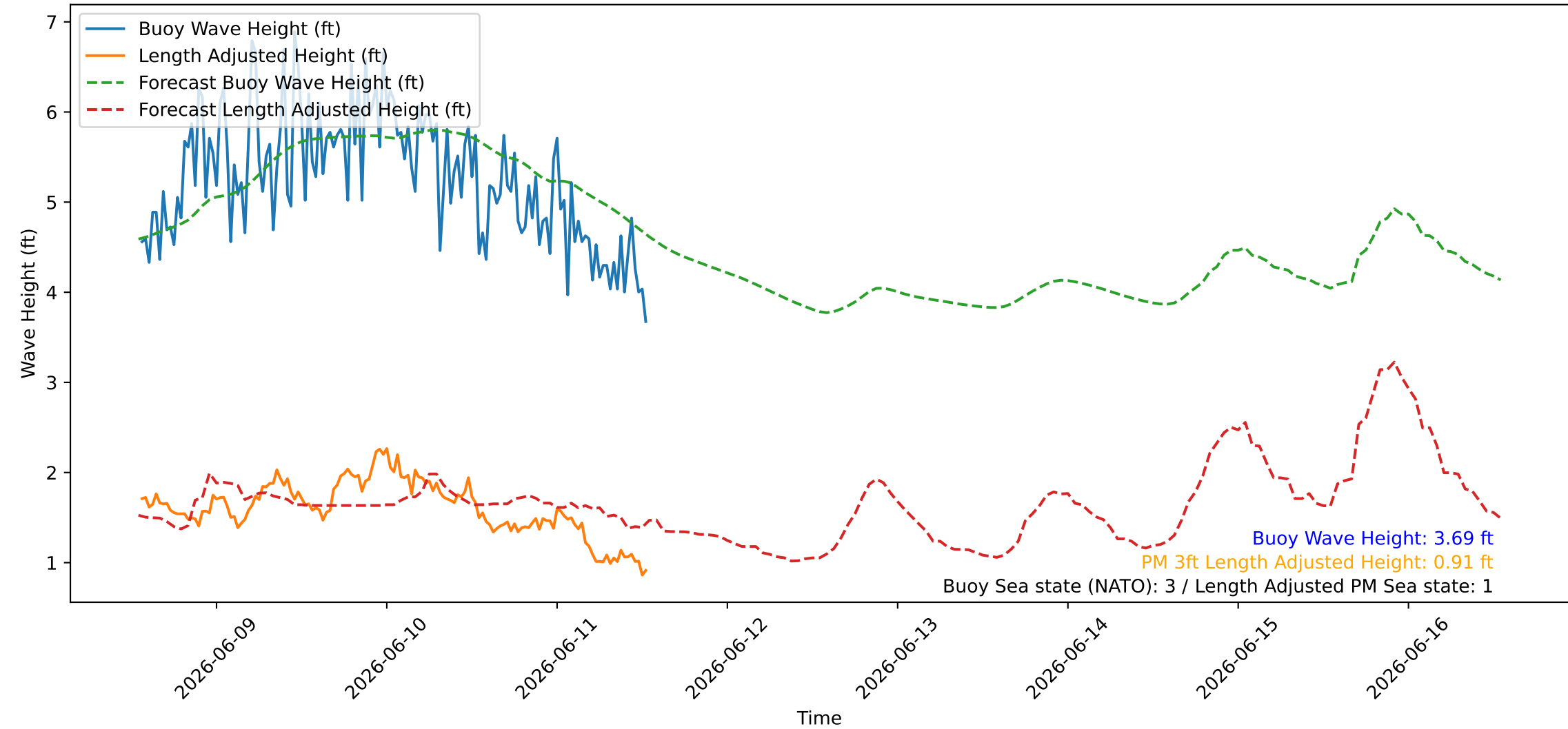
Wave Heights over Time for Green Beach at 2026-06-11 13:21:10
