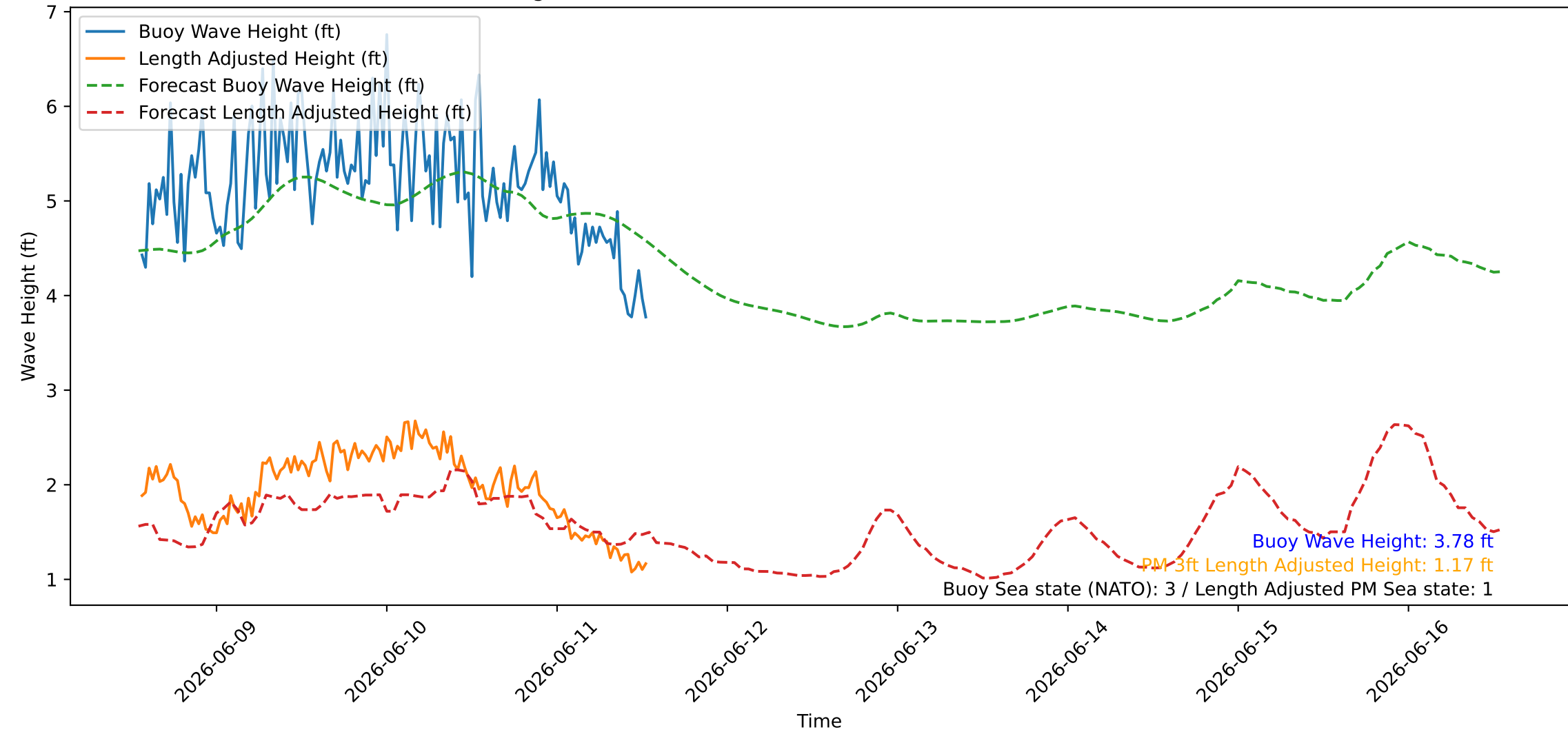
Wave Heights over Time for Oceanside Harbor at 2026-06-11 13:20:26
