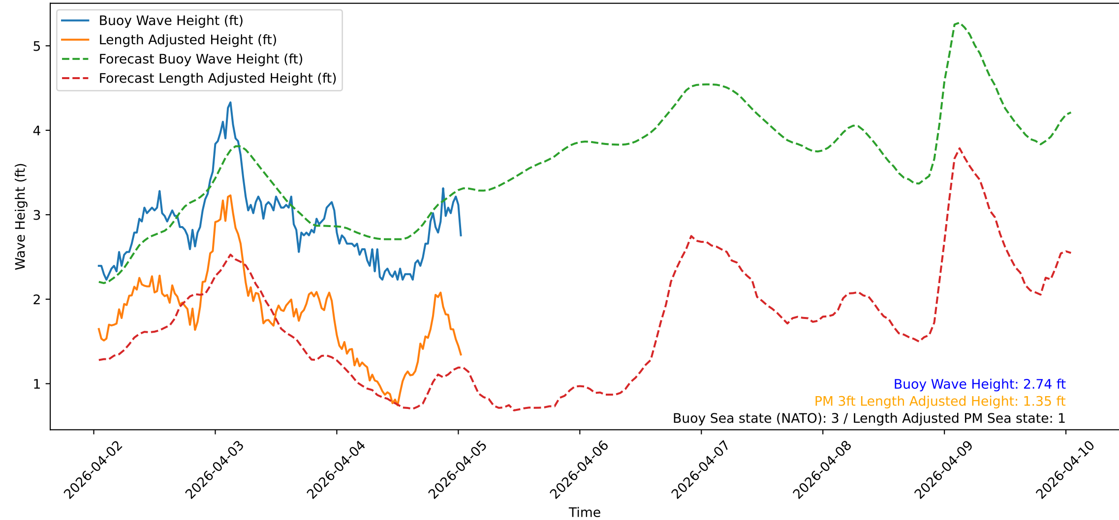
Wave Heights over Time for Green Beach at 2026-04-05 01:11:10
