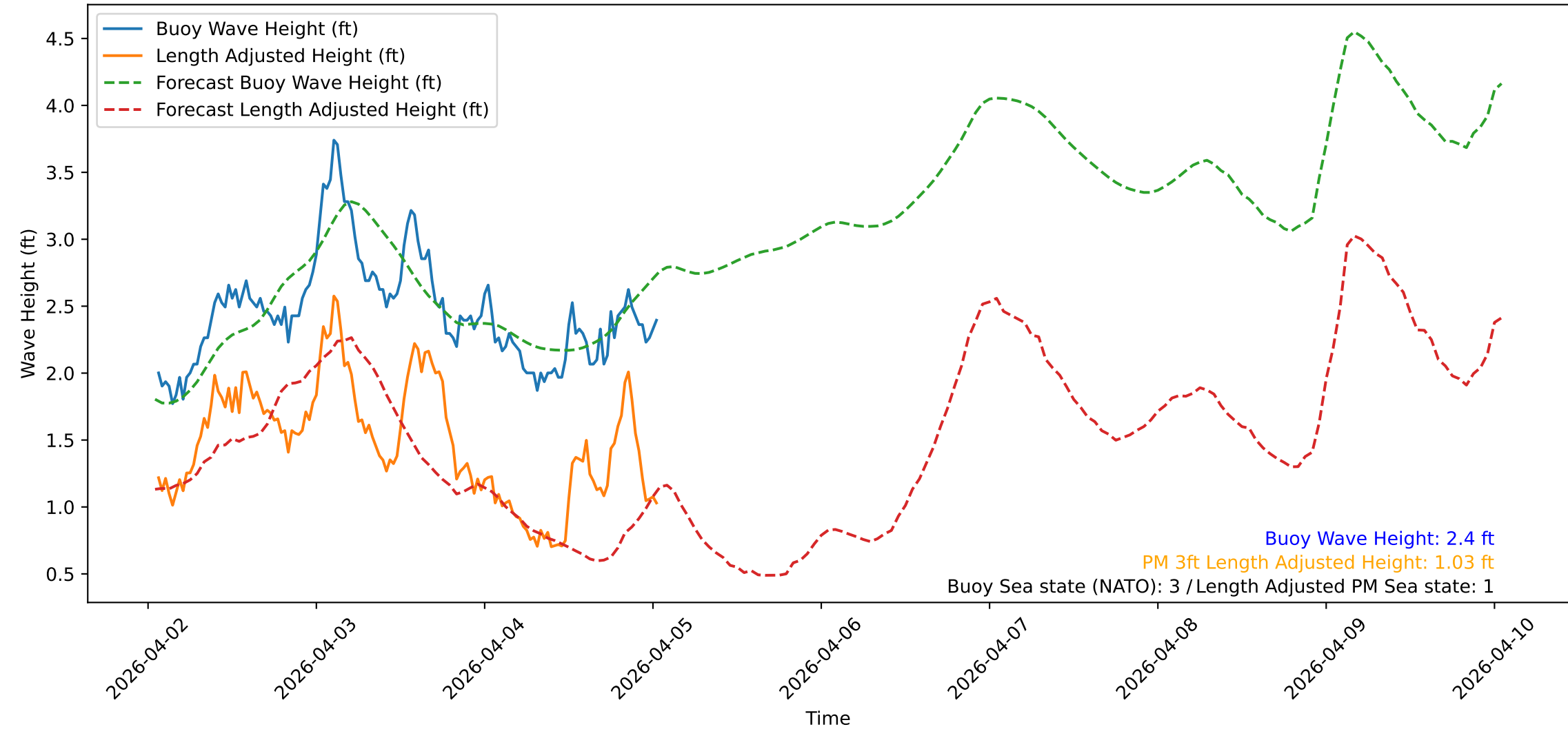
Wave Heights over Time for Red Beach at 2026-04-05 01:10:47
