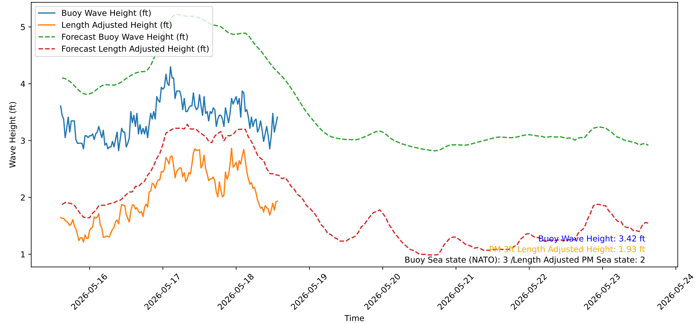
Wave Heights over Time for Oceanside Harbor at 2026-05-18 14:30:32
