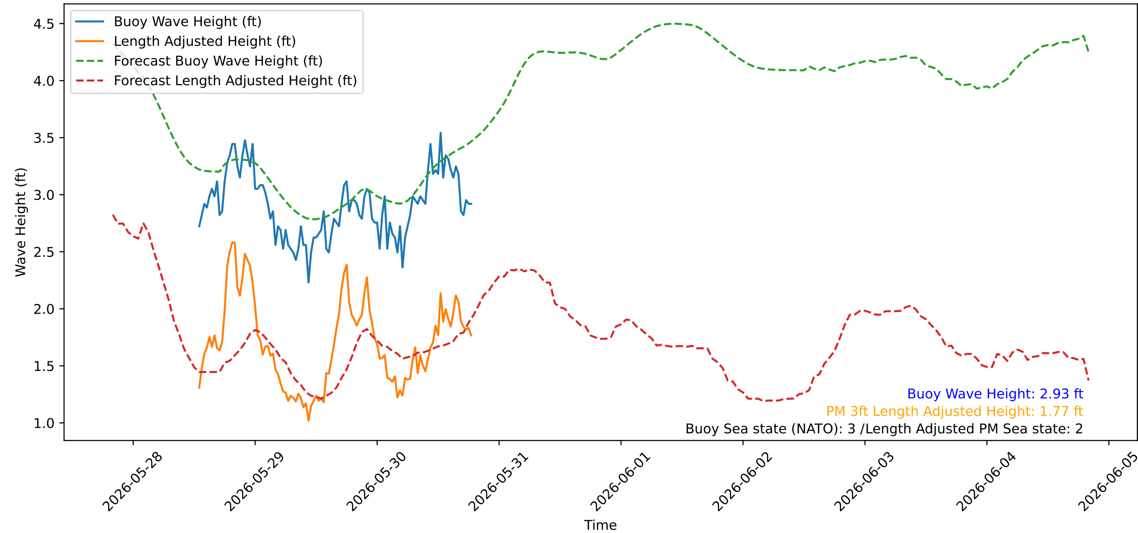
Wave Heights over Time for Oceanside Harbor at 2026-05-30 19:30:24
