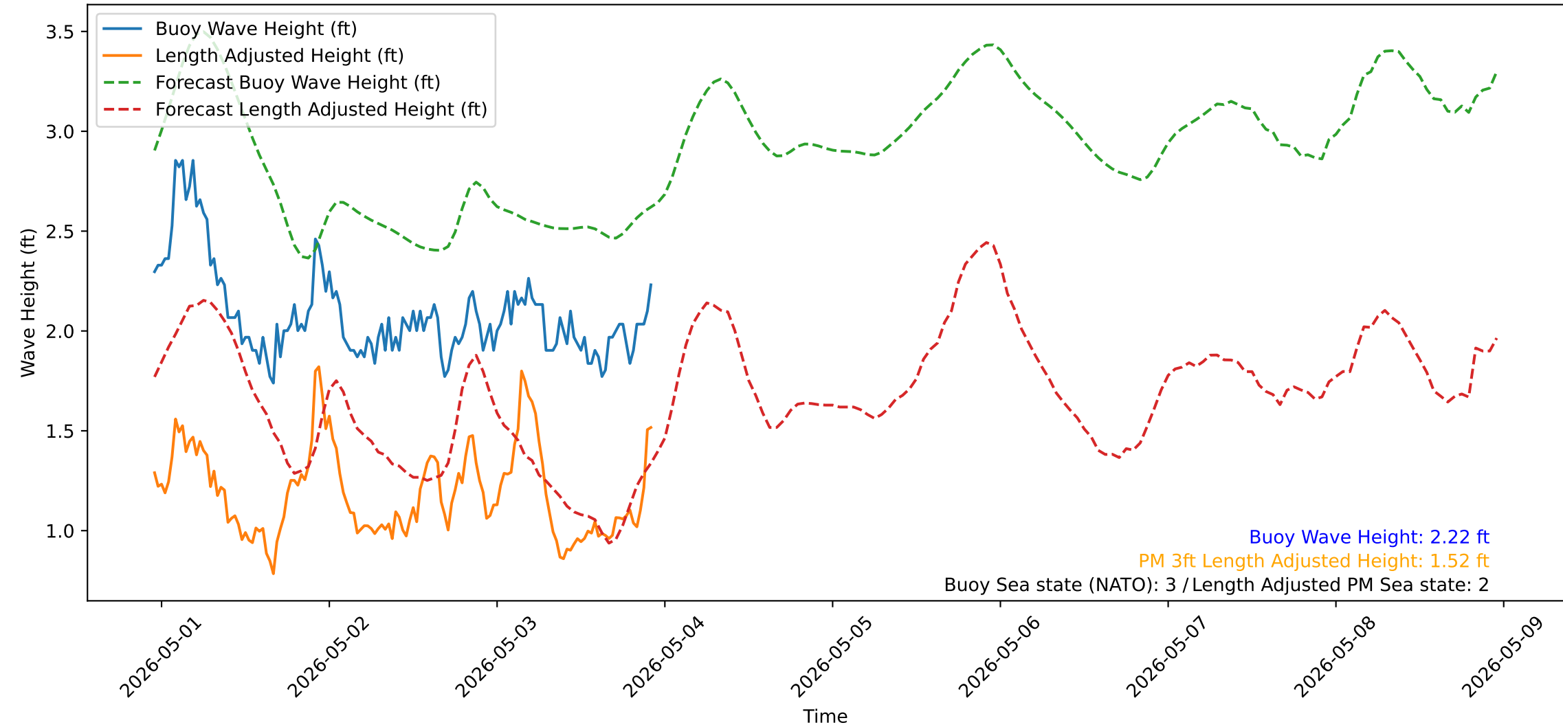
Wave Heights over Time for Green Beach at 2026-05-03 22:51:14
