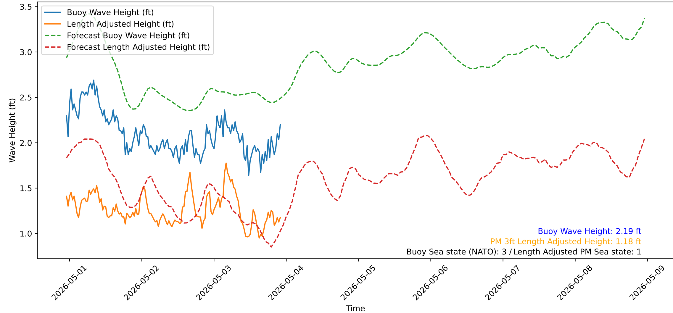
Wave Heights over Time for Oceanside Harbor at 2026-05-03 22:50:31
