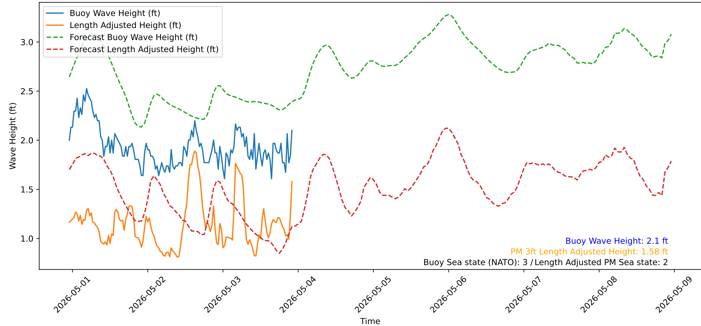
Wave Heights over Time for Red Beach at 2026-05-03 22:50:52
