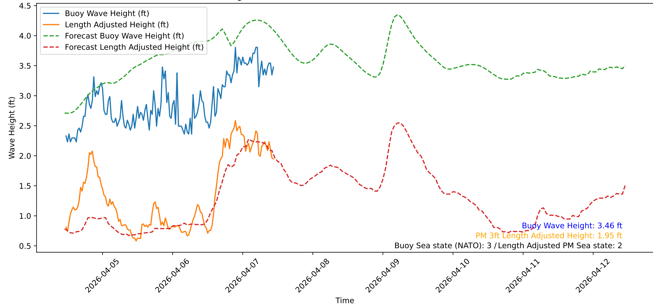
Wave Heights over Time for Green Beach at 2026-04-07 11:21:12
