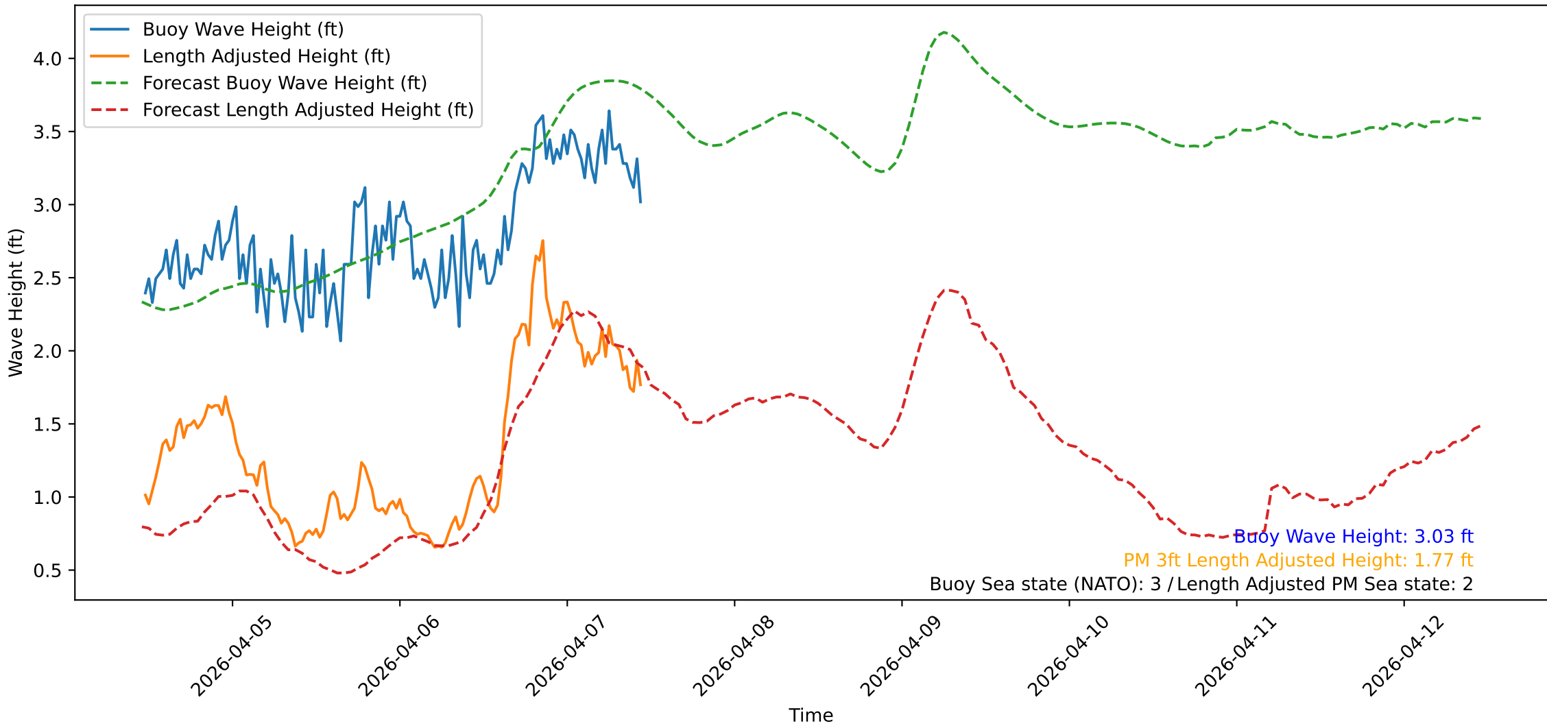
Wave Heights over Time for Oceanside Harbor at 2026-04-07 11:20:35
