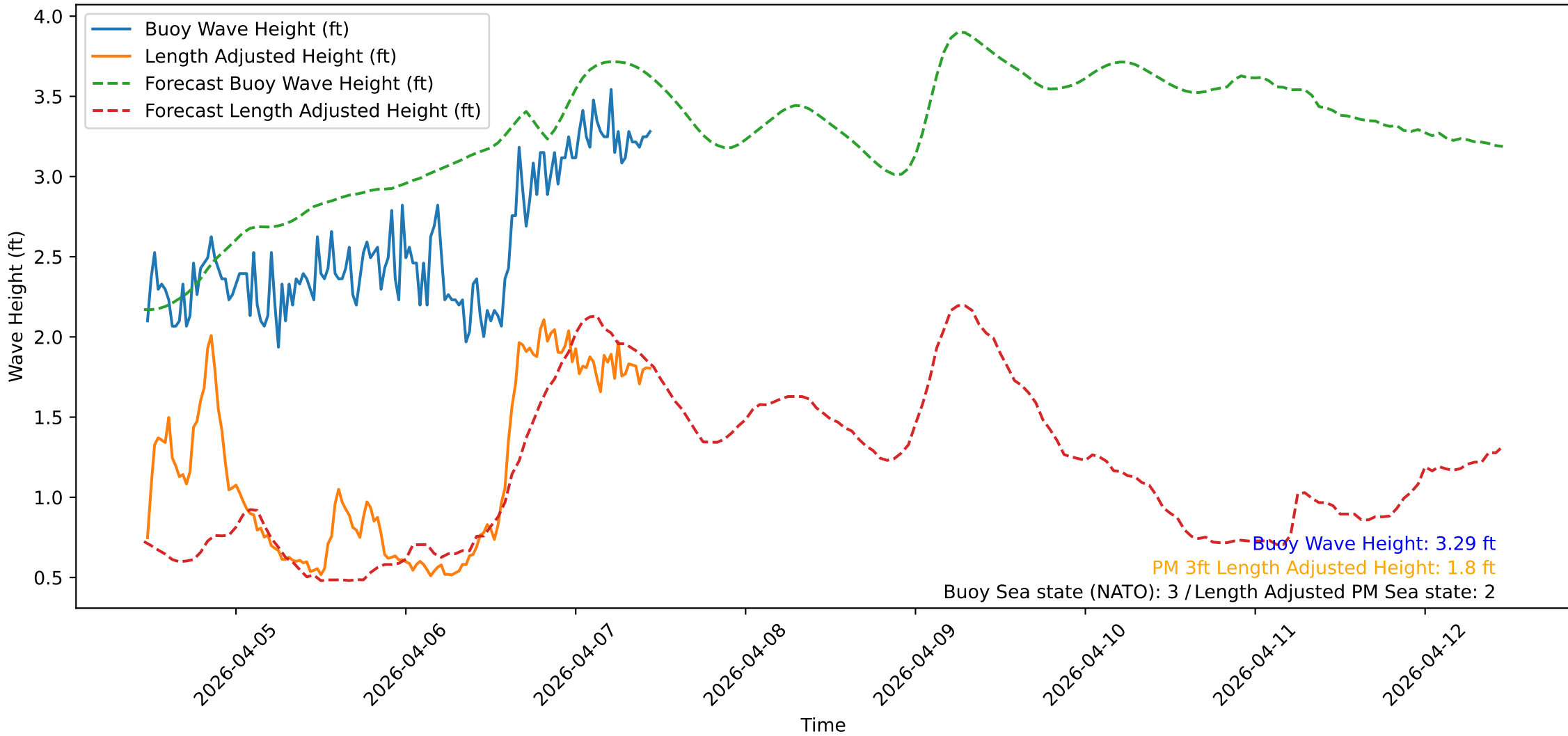
Wave Heights over Time for Red Beach at 2026-04-07 11:20:51
