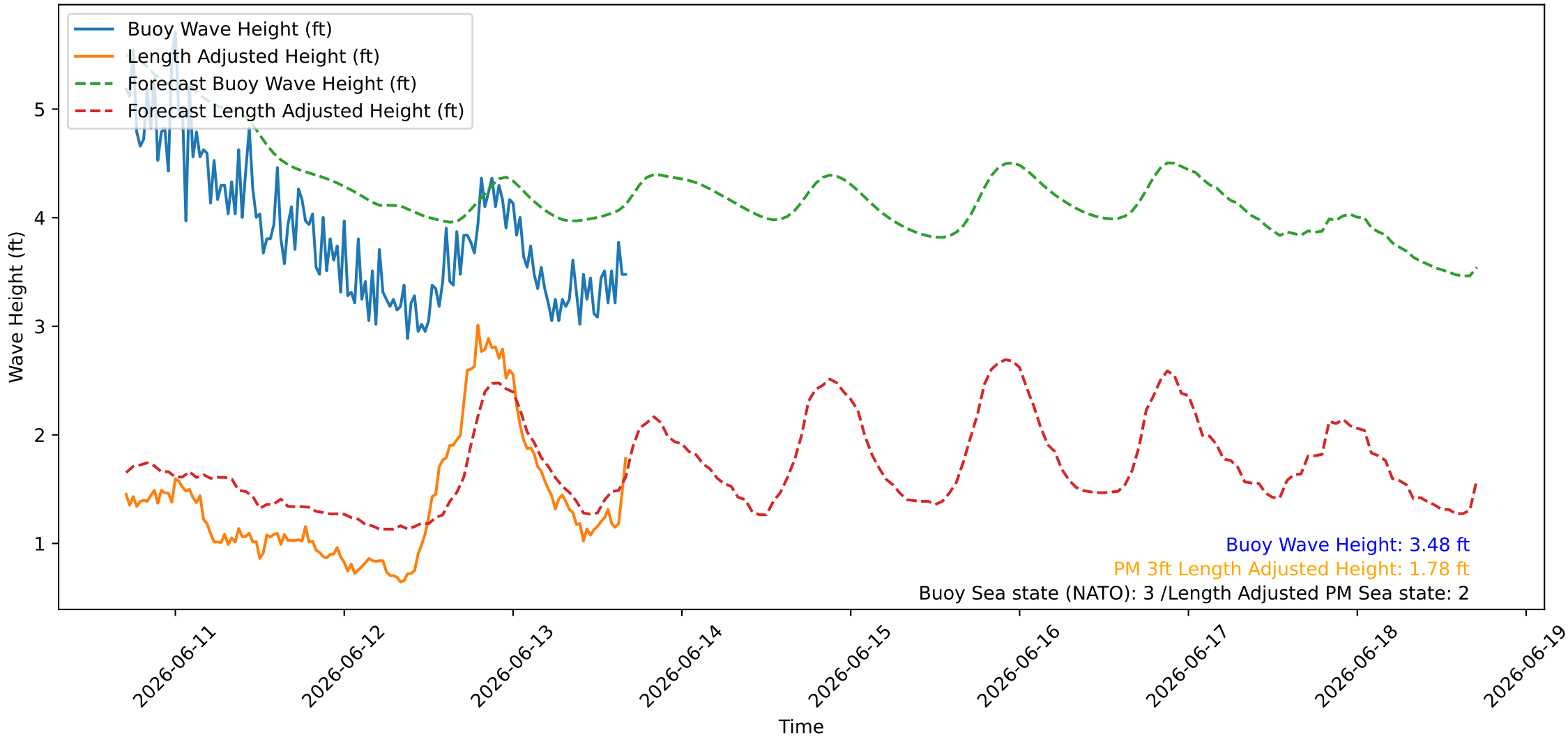
Wave Heights over Time for Green Beach at 2026-06-13 16:51:09
