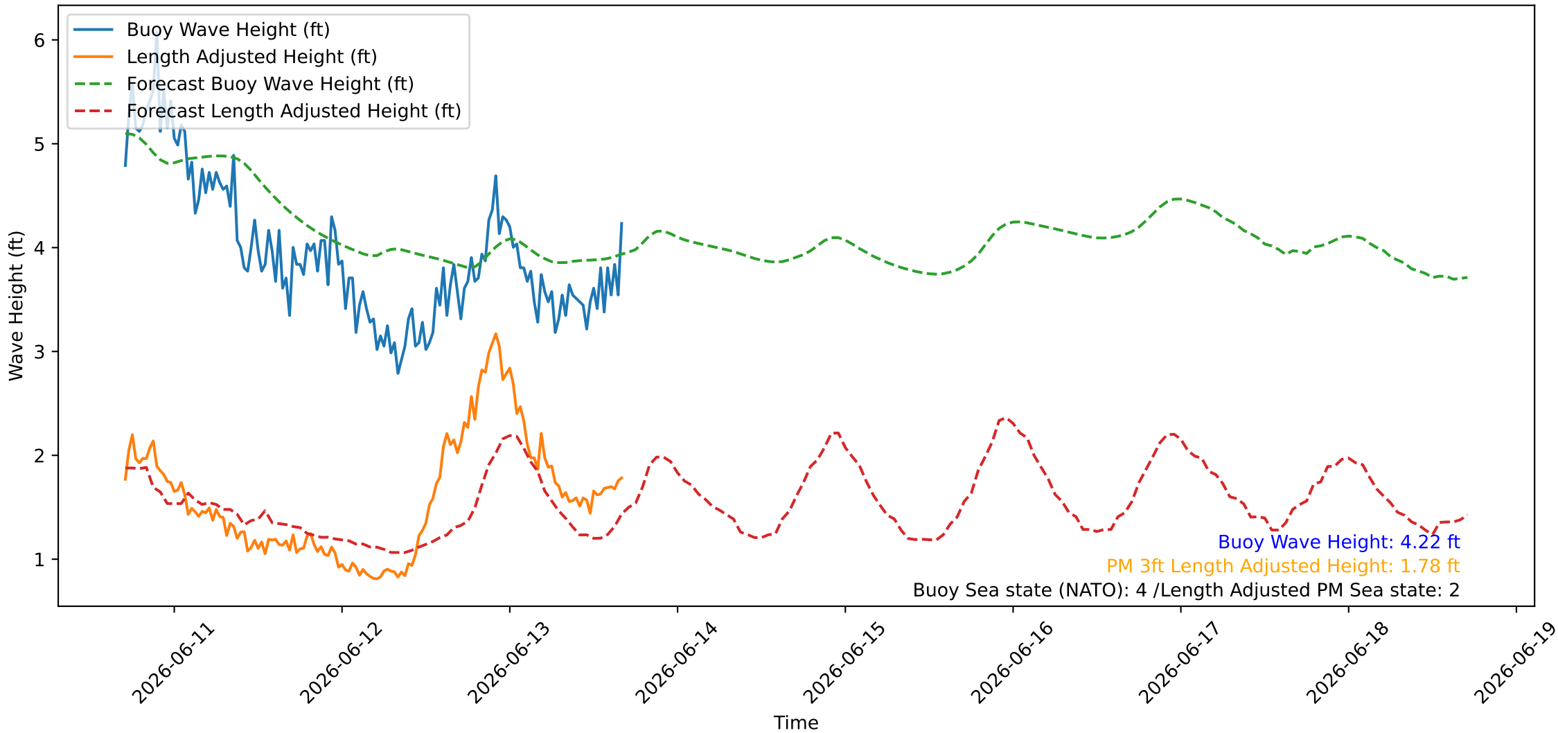
Wave Heights over Time for Oceanside Harbor at 2026-06-13 16:50:26
