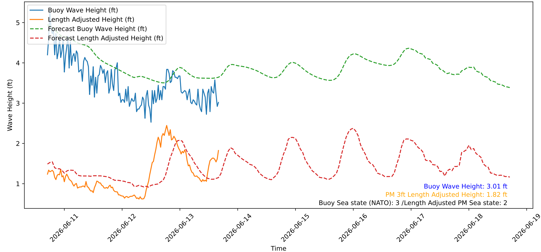
Wave Heights over Time for Red Beach at 2026-06-13 16:50:47
