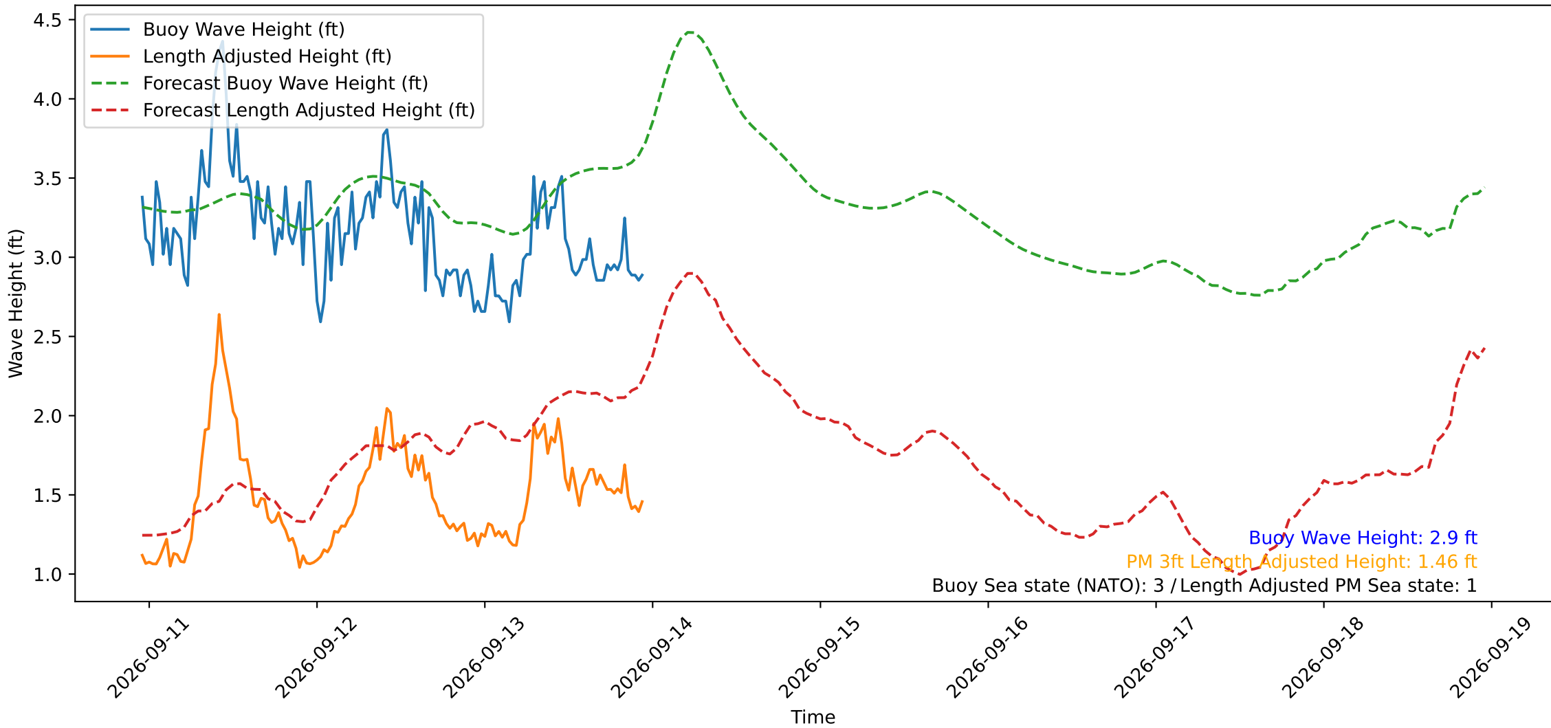
Wave Heights over Time for Oceanside Harbor at 2026-09-13 23:00:29
