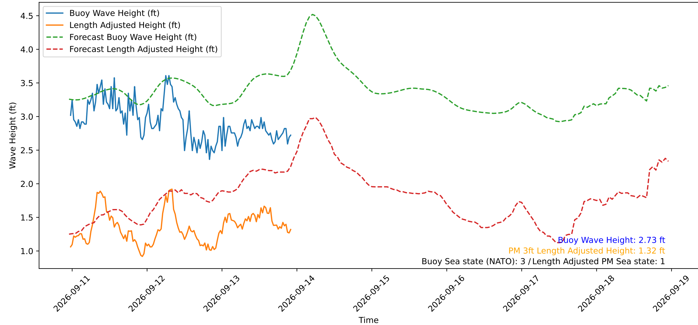
Wave Heights over Time for Green Beach at 2026-09-13 23:01:11
