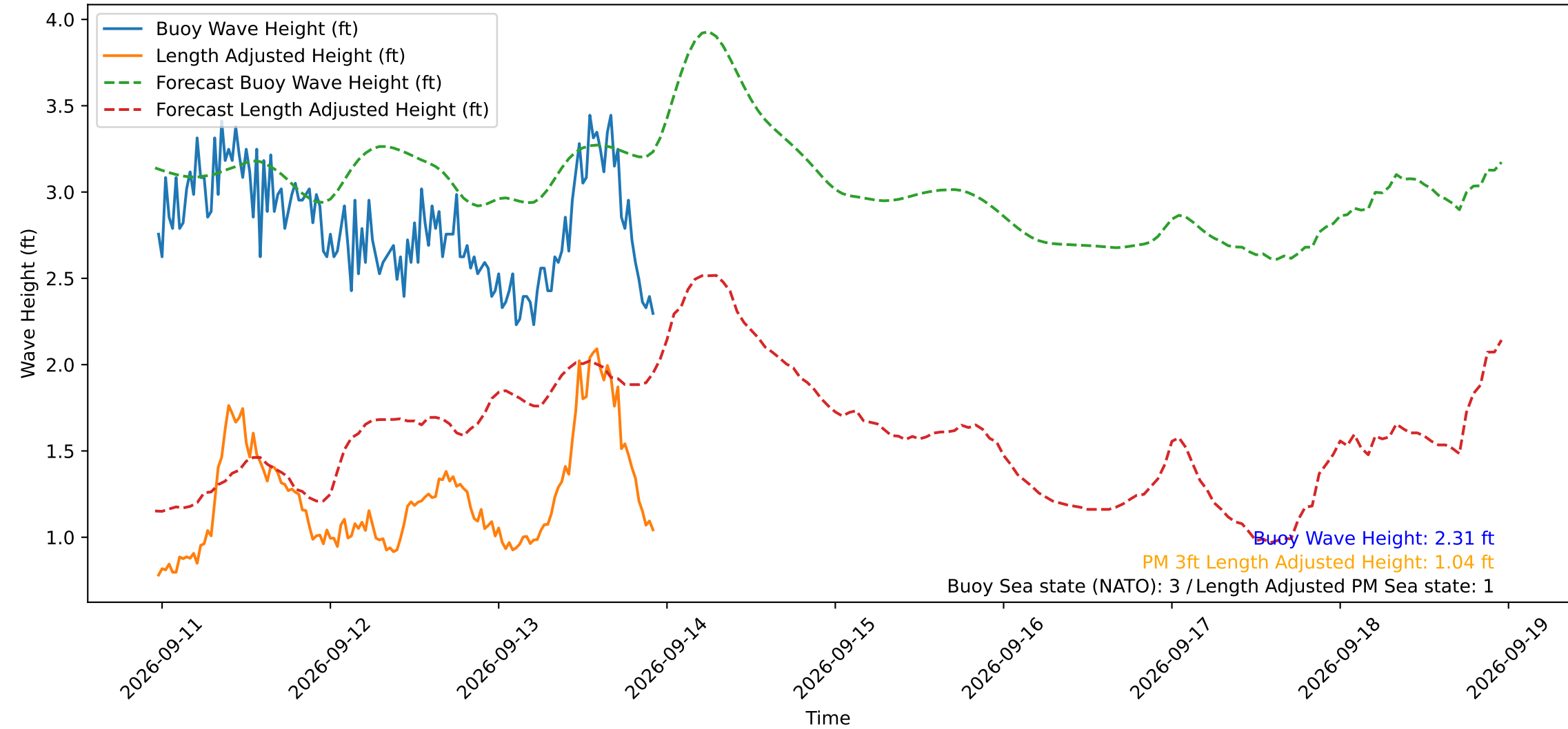
Wave Heights over Time for Red Beach at 2026-09-13 23:00:49
