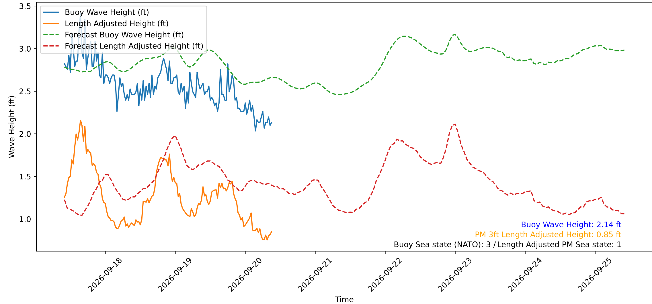
Wave Heights over Time for Red Beach at 2026-09-20 09:50:50
