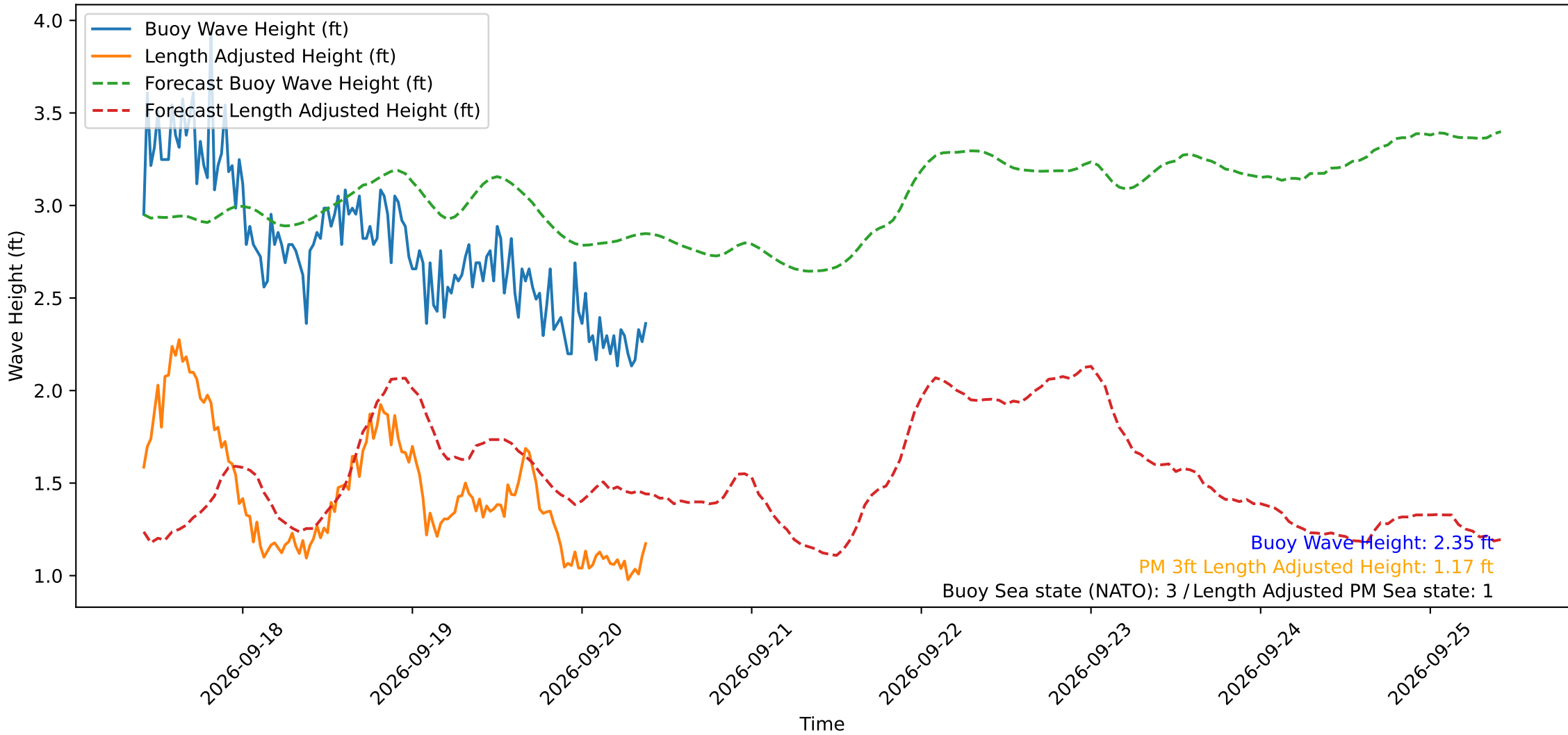
Wave Heights over Time for Oceanside Harbor at 2026-09-20 09:50:30
