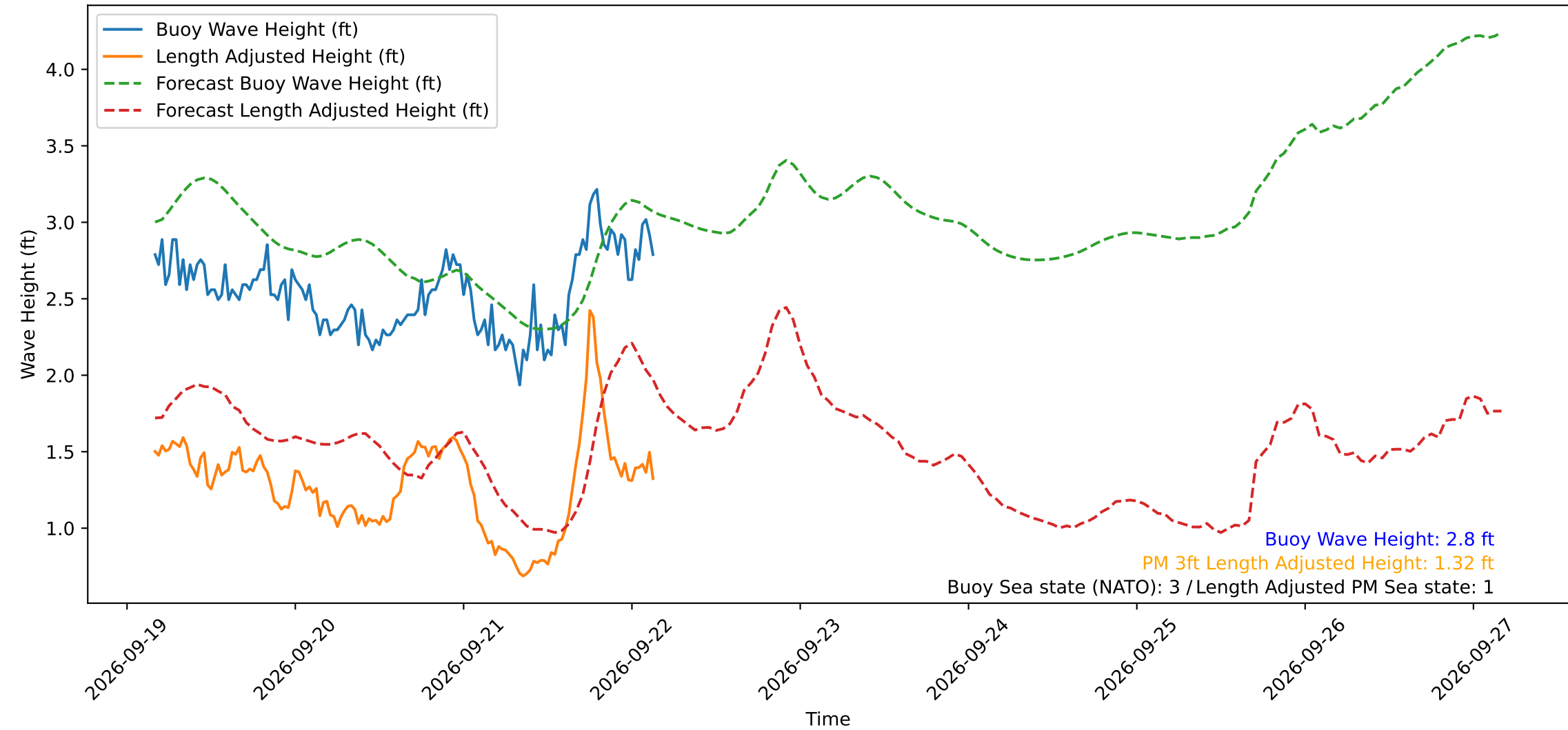
Wave Heights over Time for Green Beach at 2026-09-22 03:41:12
