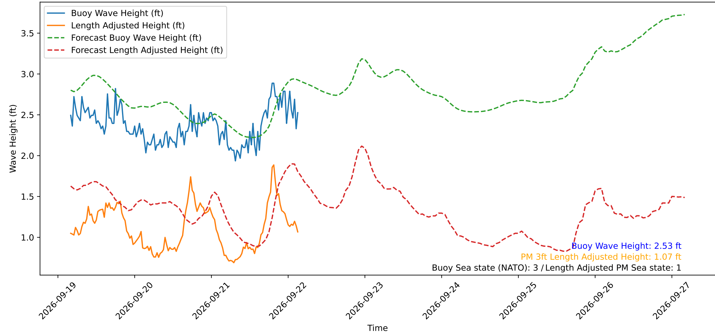
Wave Heights over Time for Red Beach at 2026-09-22 03:40:50
