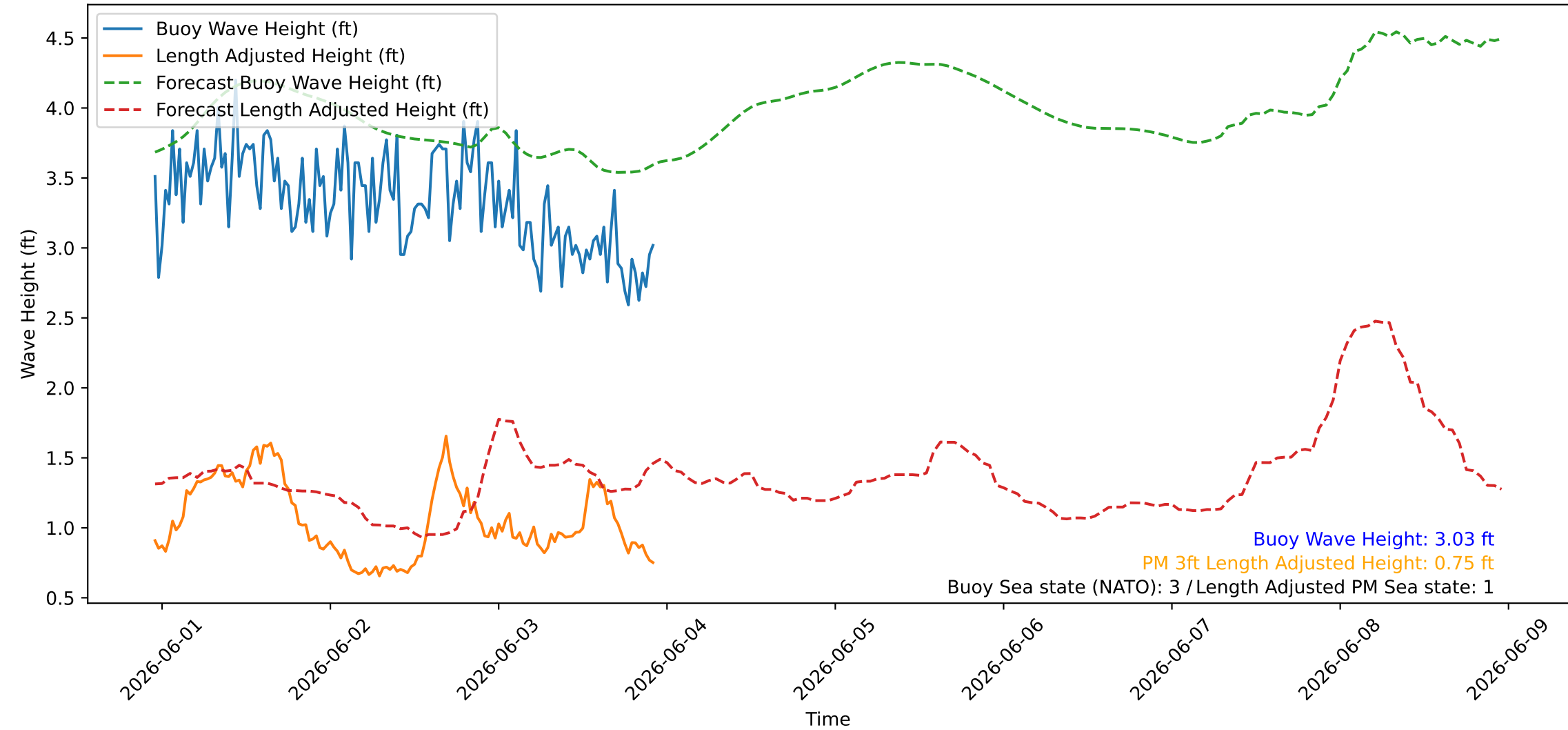
Wave Heights over Time for Red Beach at 2026-06-03 22:50:47
