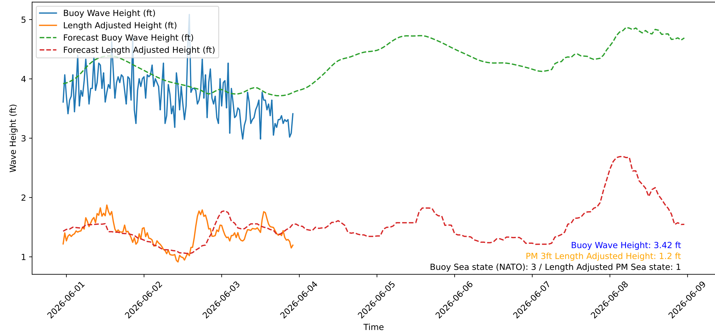
Wave Heights over Time for Oceanside Harbor at 2026-06-03 22:50:26
