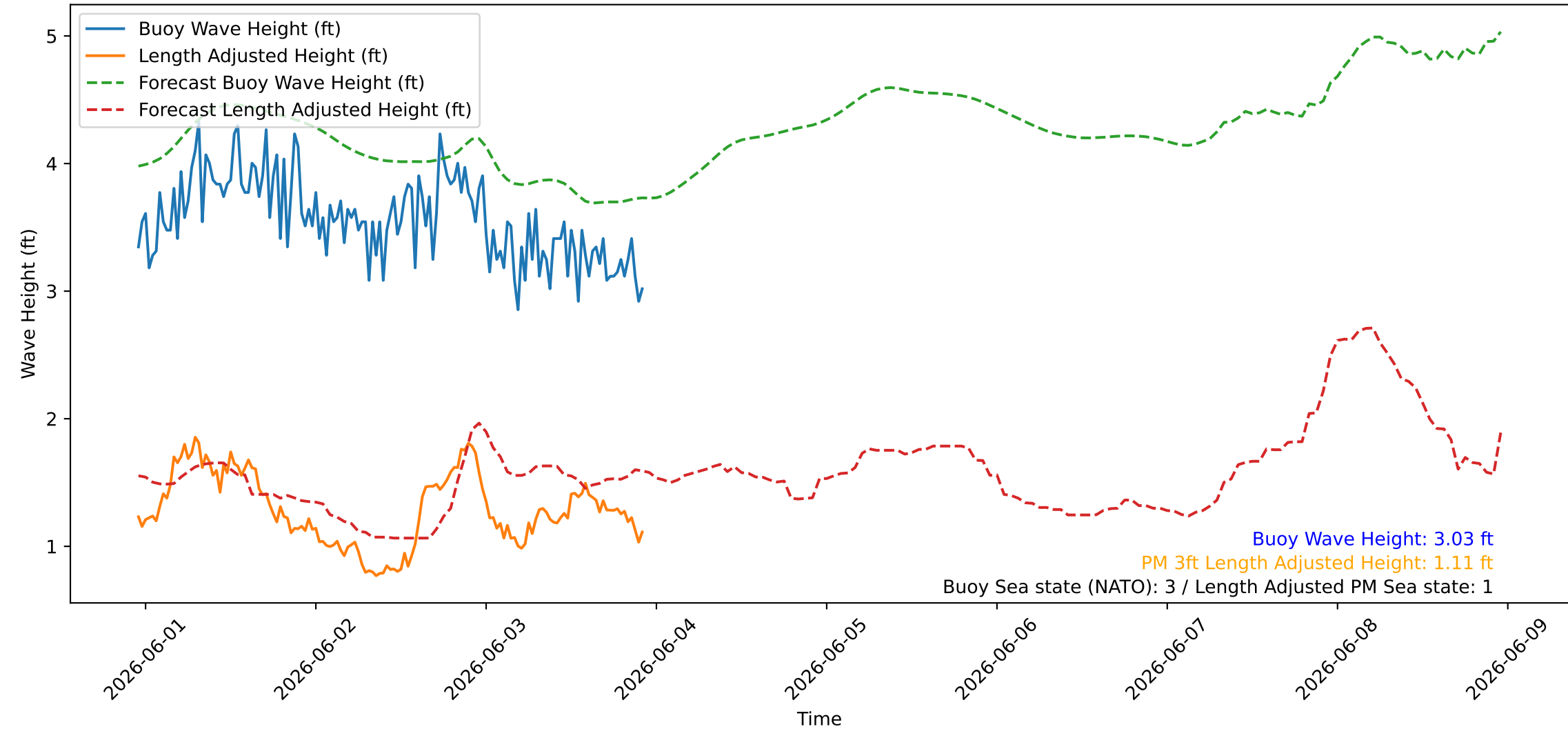
Wave Heights over Time for Green Beach at 2026-06-03 22:51:09
