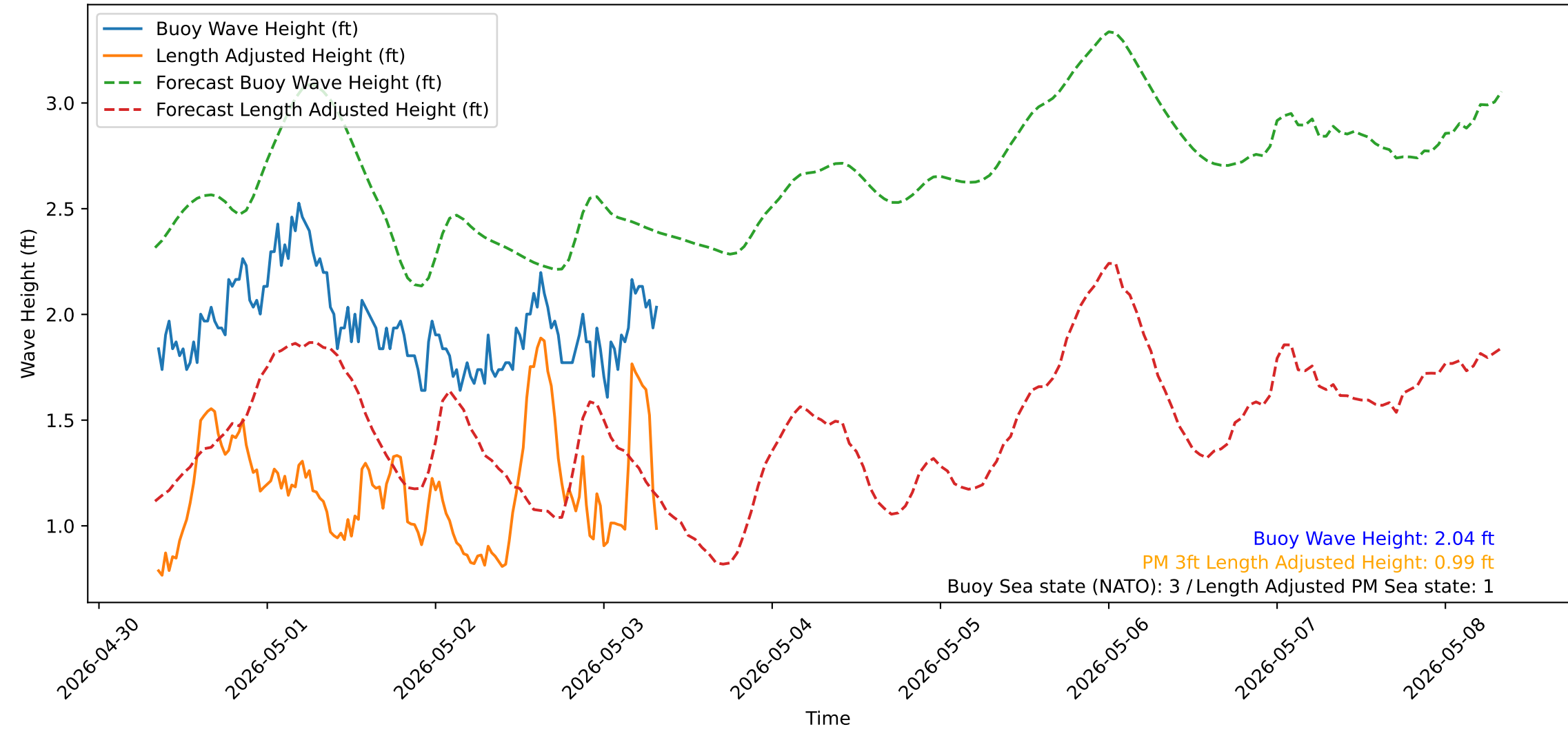
Wave Heights over Time for Red Beach at 2026-05-03 08:20:51
