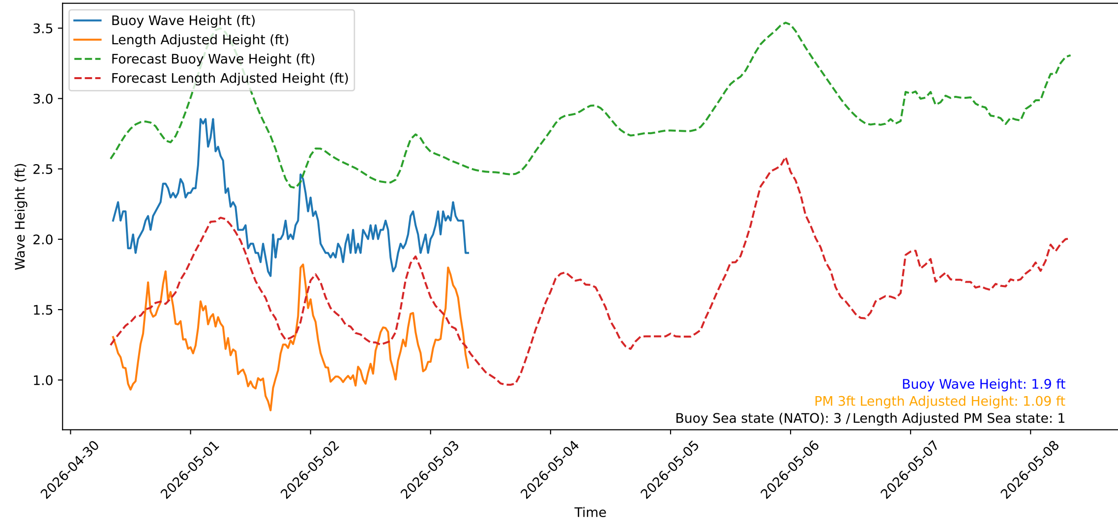
Wave Heights over Time for Green Beach at 2026-05-03 08:21:13
