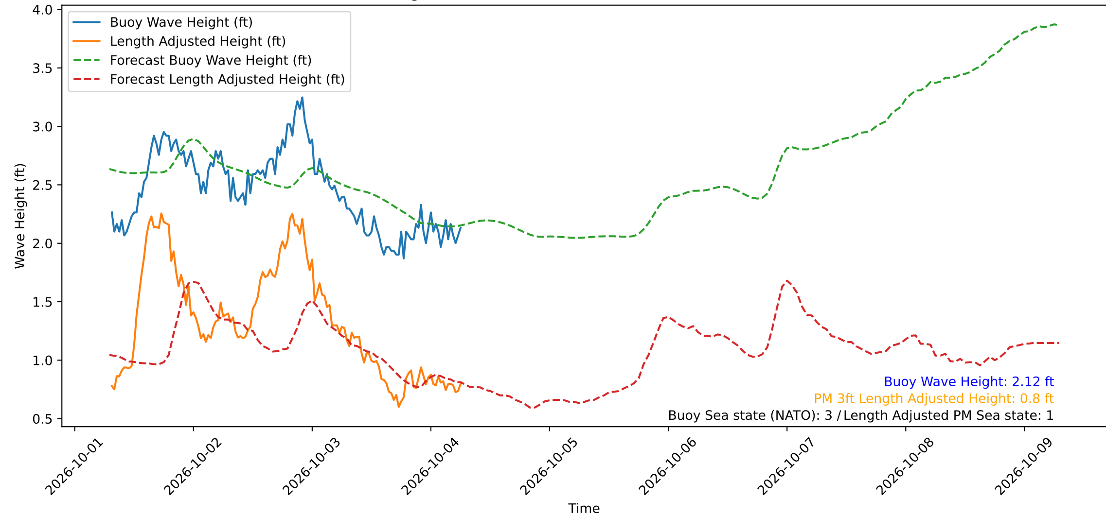
Wave Heights over Time for Red Beach at 2026-10-04 07:00:48
