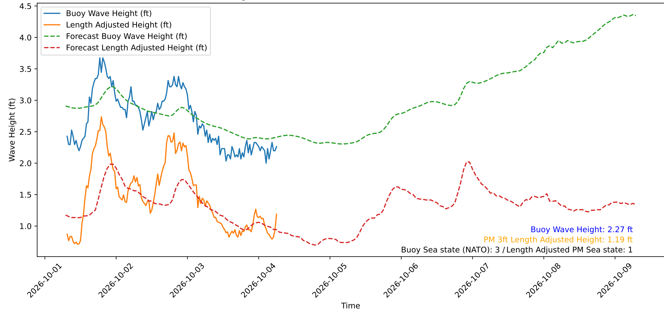
Wave Heights over Time for Green Beach at 2026-10-04 07:01:10
