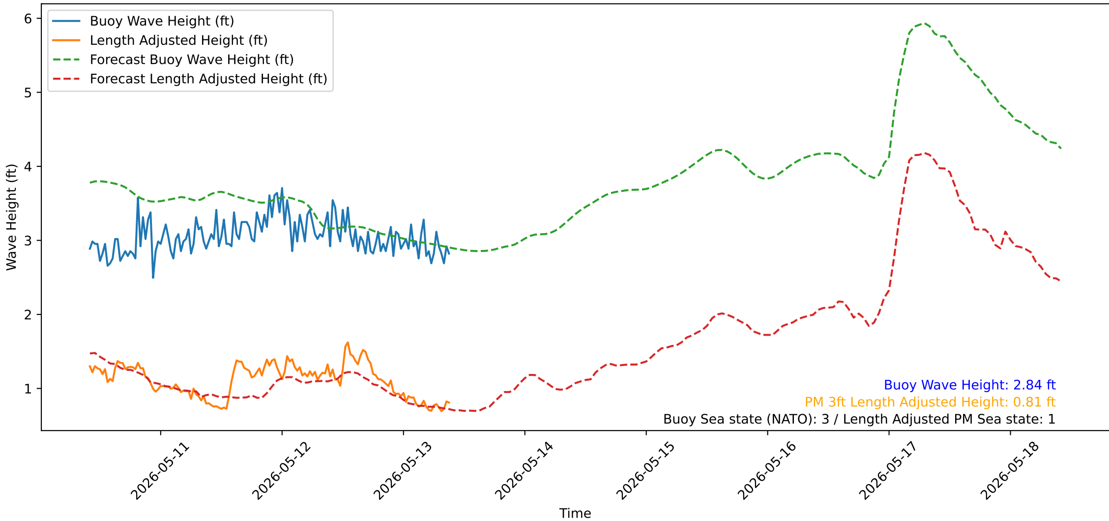
Wave Heights over Time for Oceanside Harbor at 2026-05-13 09:50:31
