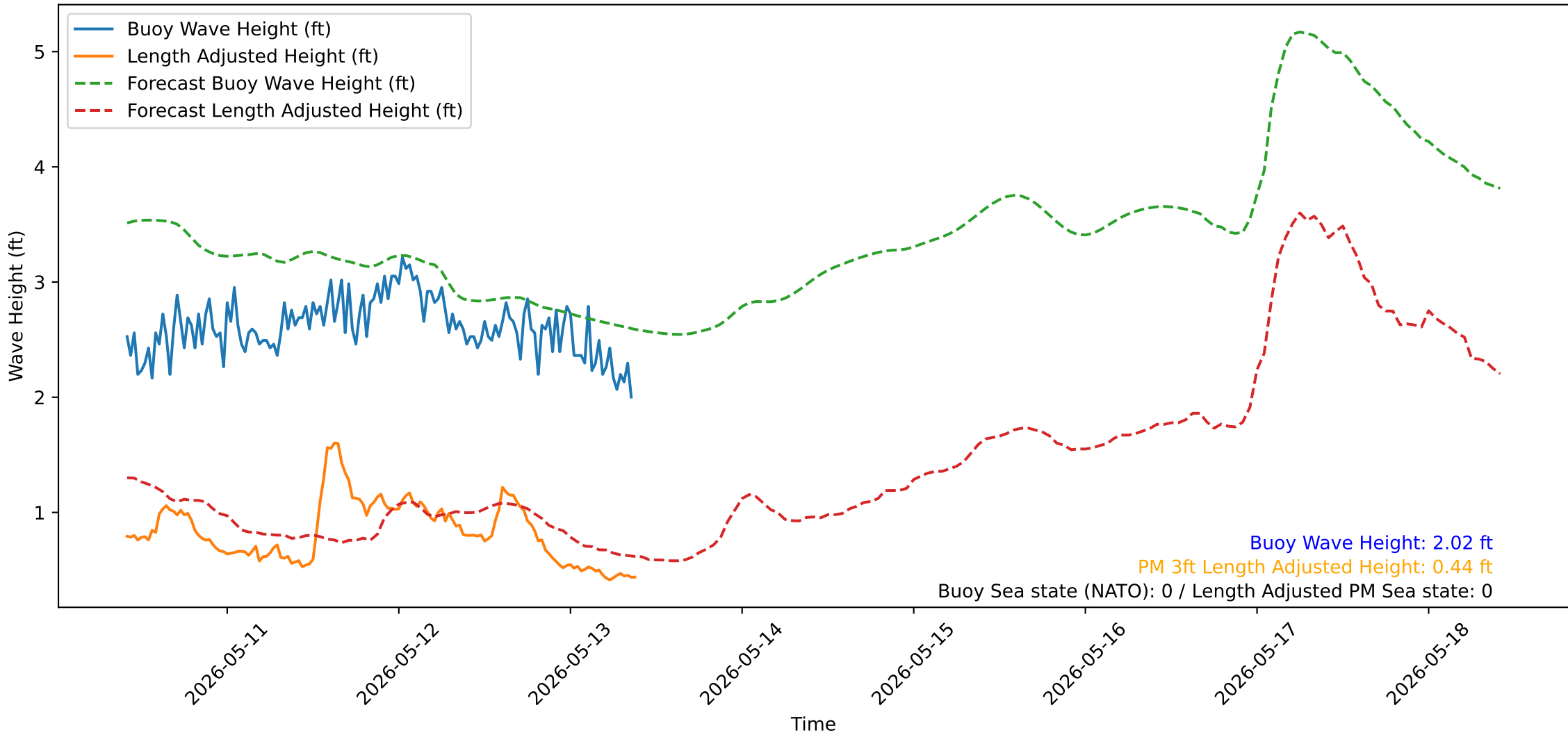
Wave Heights over Time for Red Beach at 2026-05-13 09:50:52
