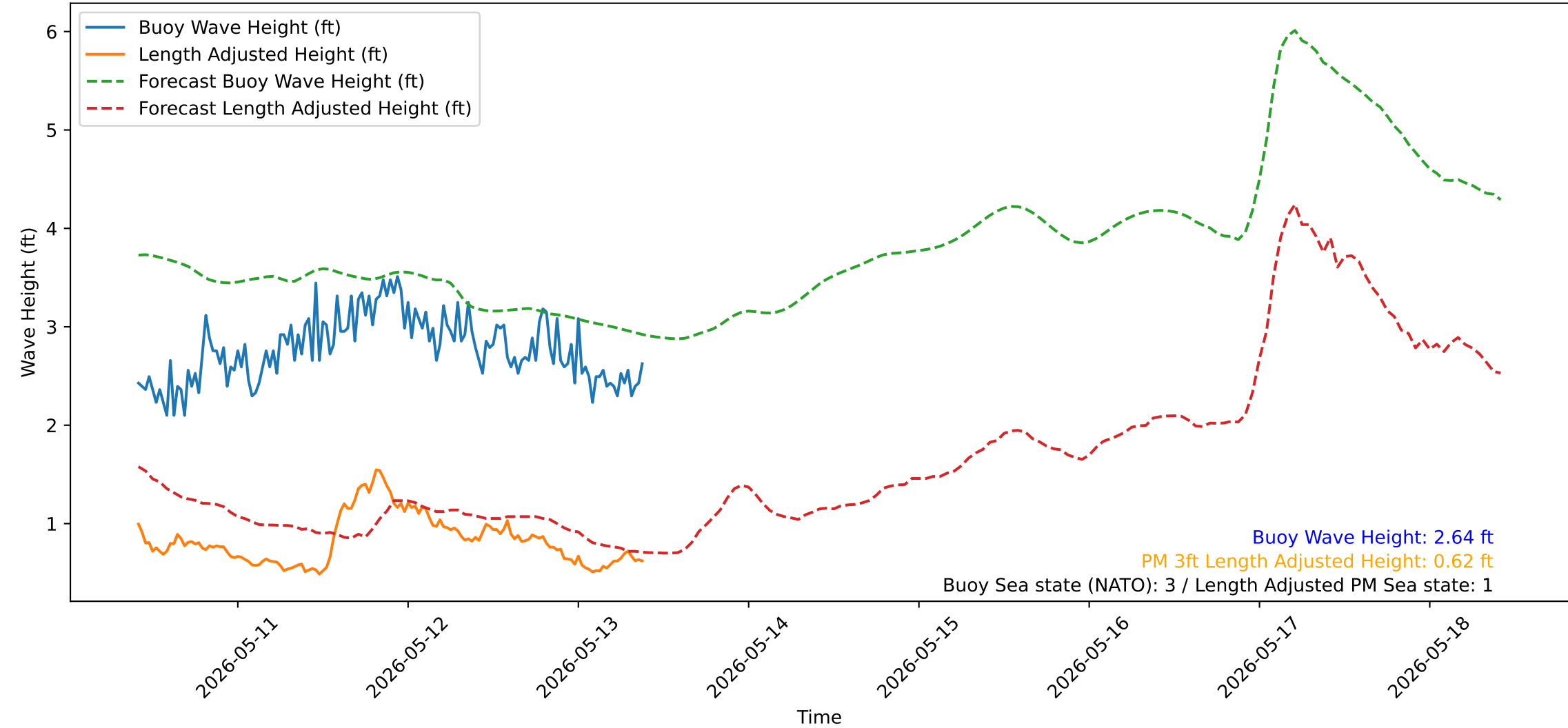
Wave Heights over Time for Green Beach at 2026-05-13 09:51:14
