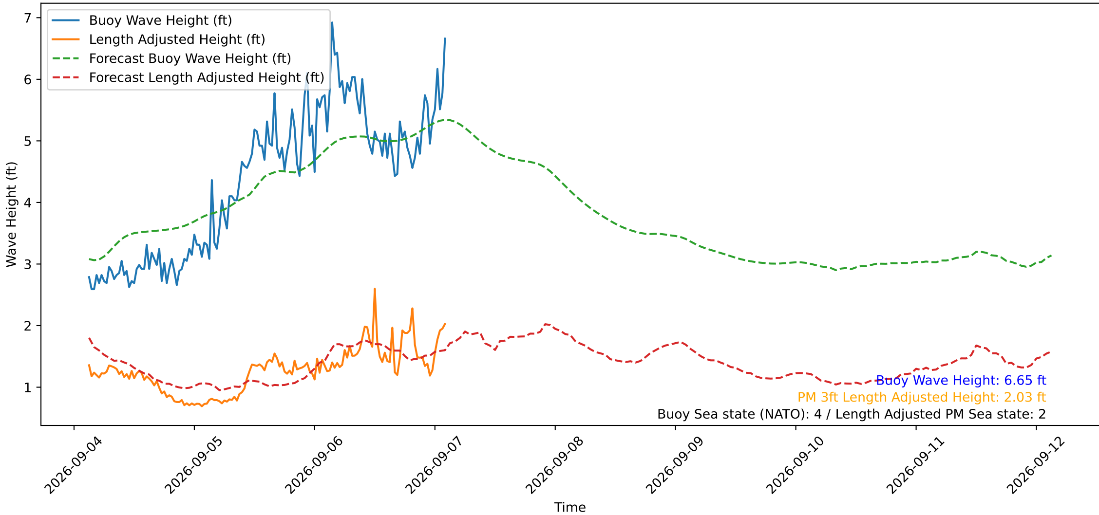
Wave Heights over Time for Red Beach at 2026-09-07 02:40:49
