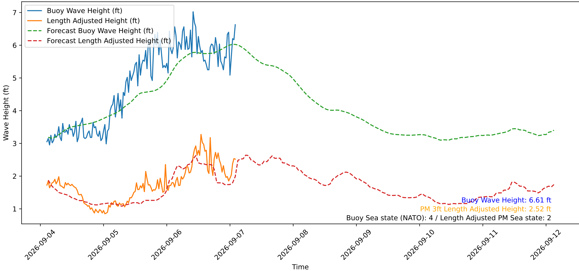
Wave Heights over Time for Oceanside Harbor at 2026-09-07 02:40:30
