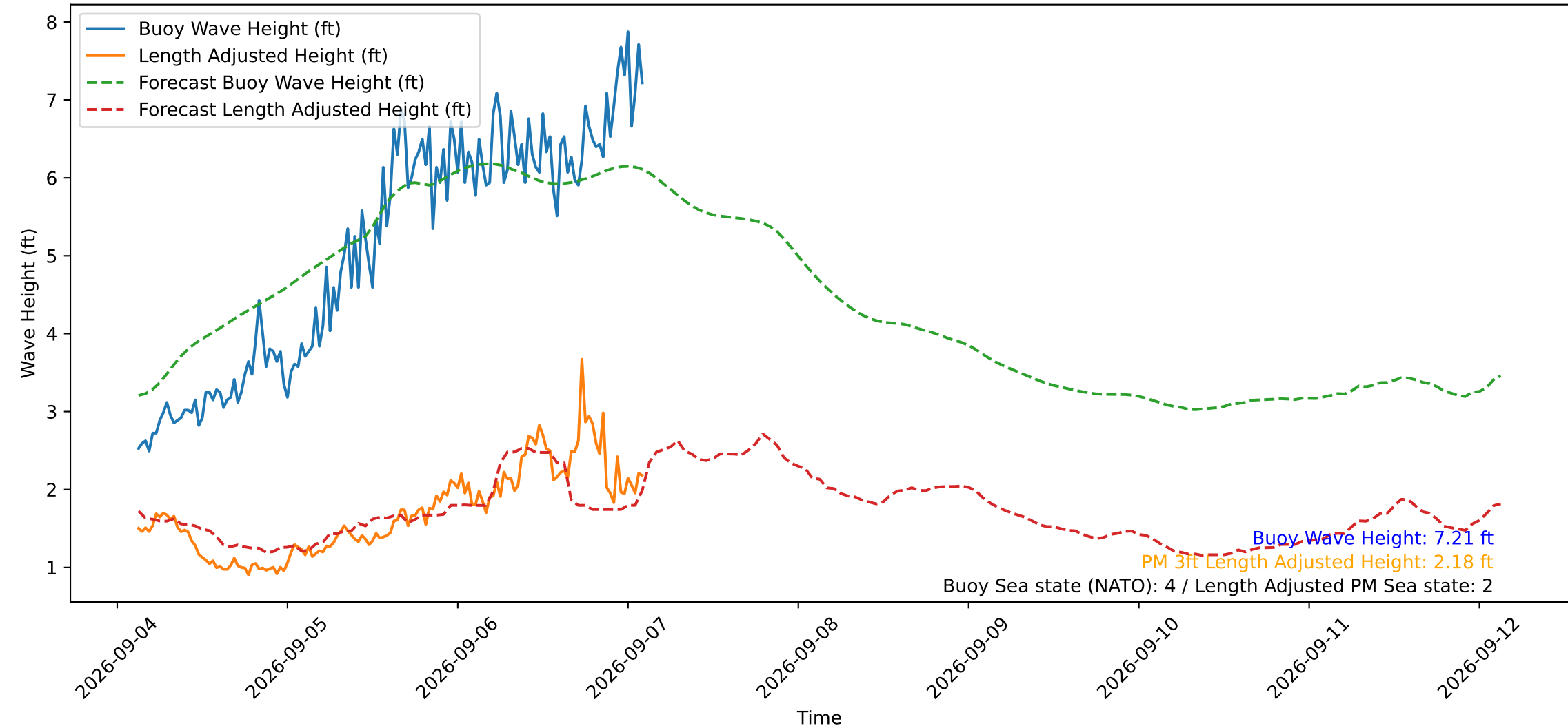
Wave Heights over Time for Green Beach at 2026-09-07 02:41:12
