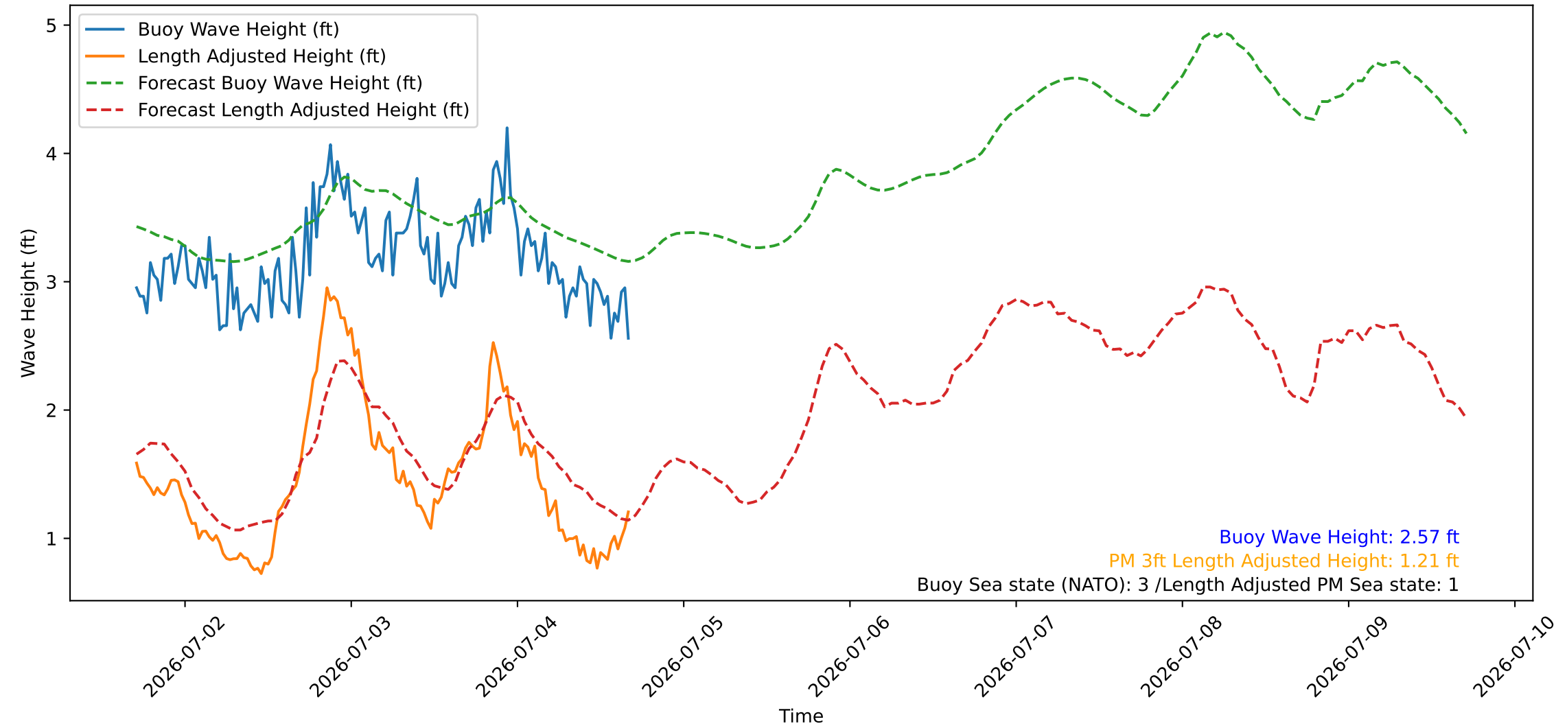
Wave Heights over Time for Green Beach at 2026-07-04 17:01:09
