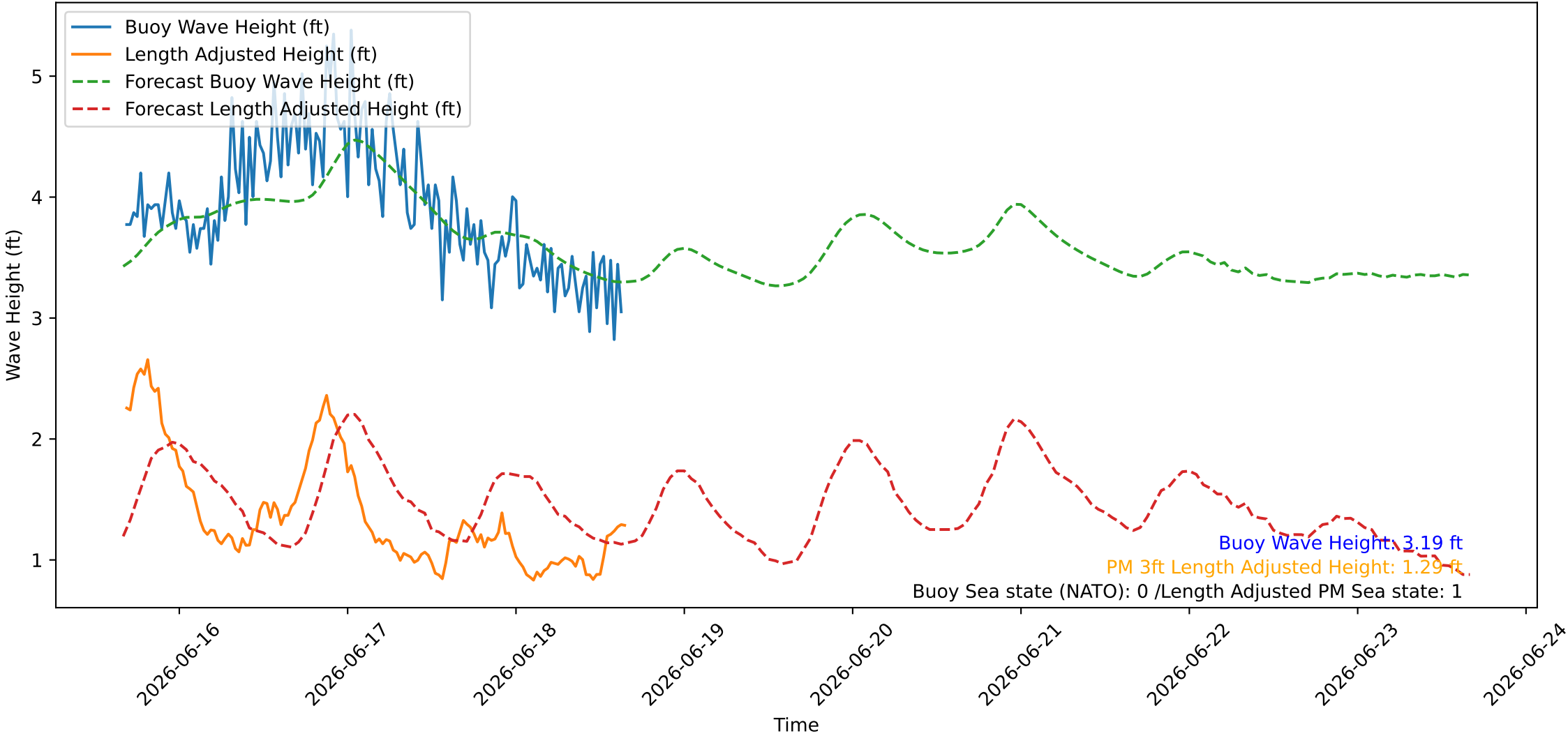
Wave Heights over Time for Red Beach at 2026-06-18 16:20:47
