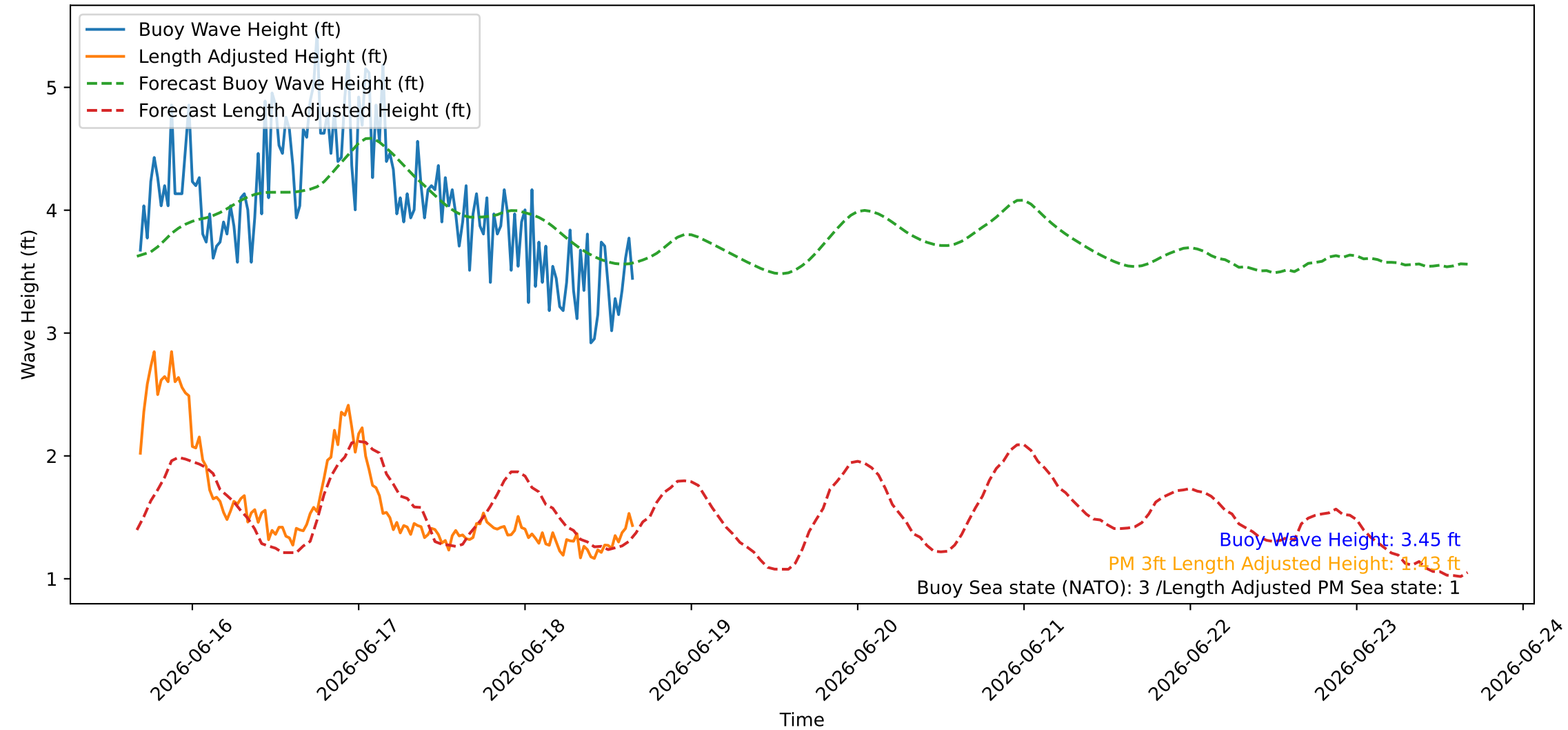
Wave Heights over Time for Oceanside Harbor at 2026-06-18 16:20:27
