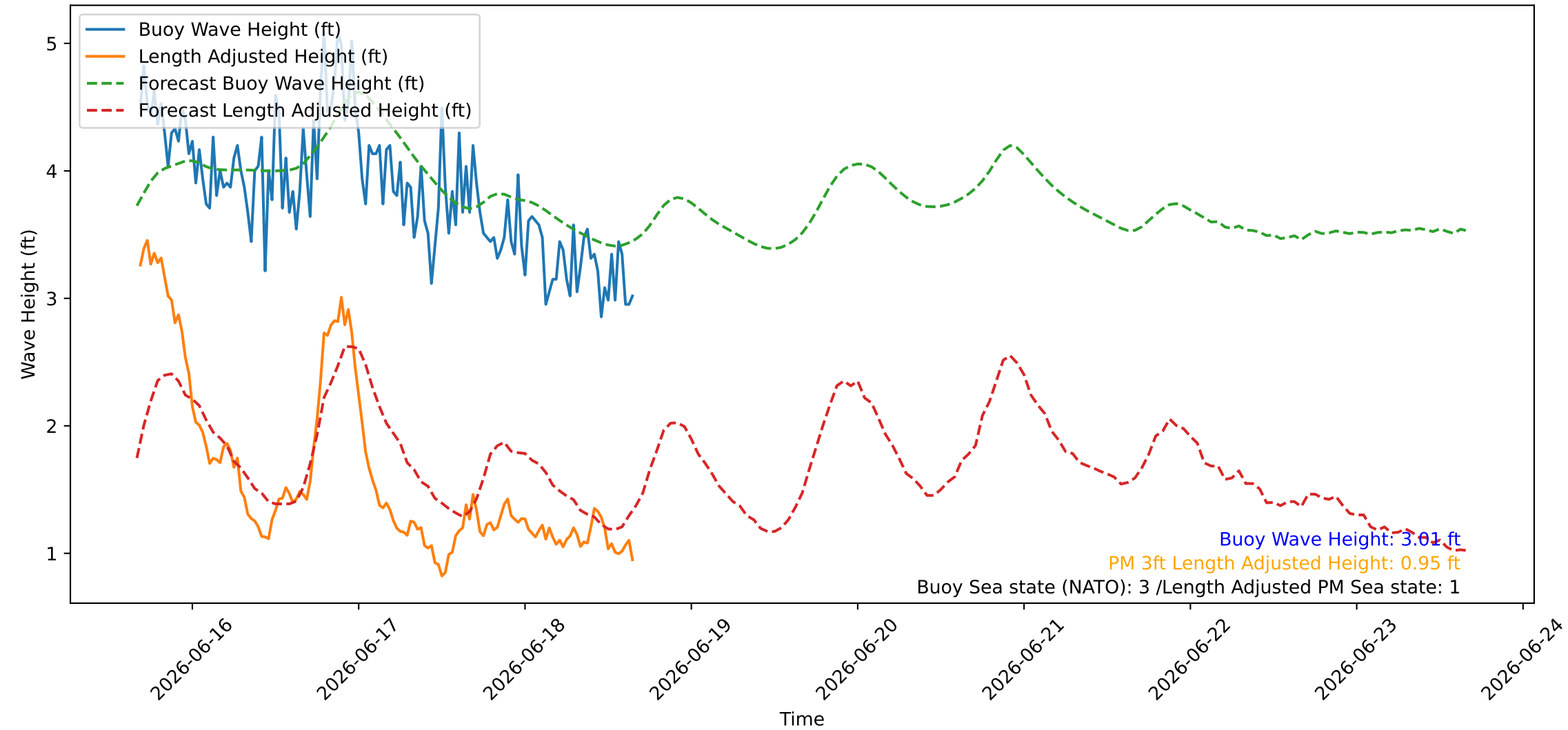
Wave Heights over Time for Green Beach at 2026-06-18 16:21:10
