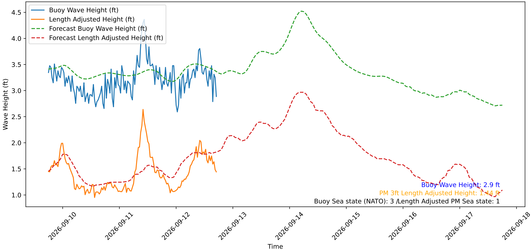
Wave Heights over Time for Oceanside Harbor at 2026-09-12 18:00:30
