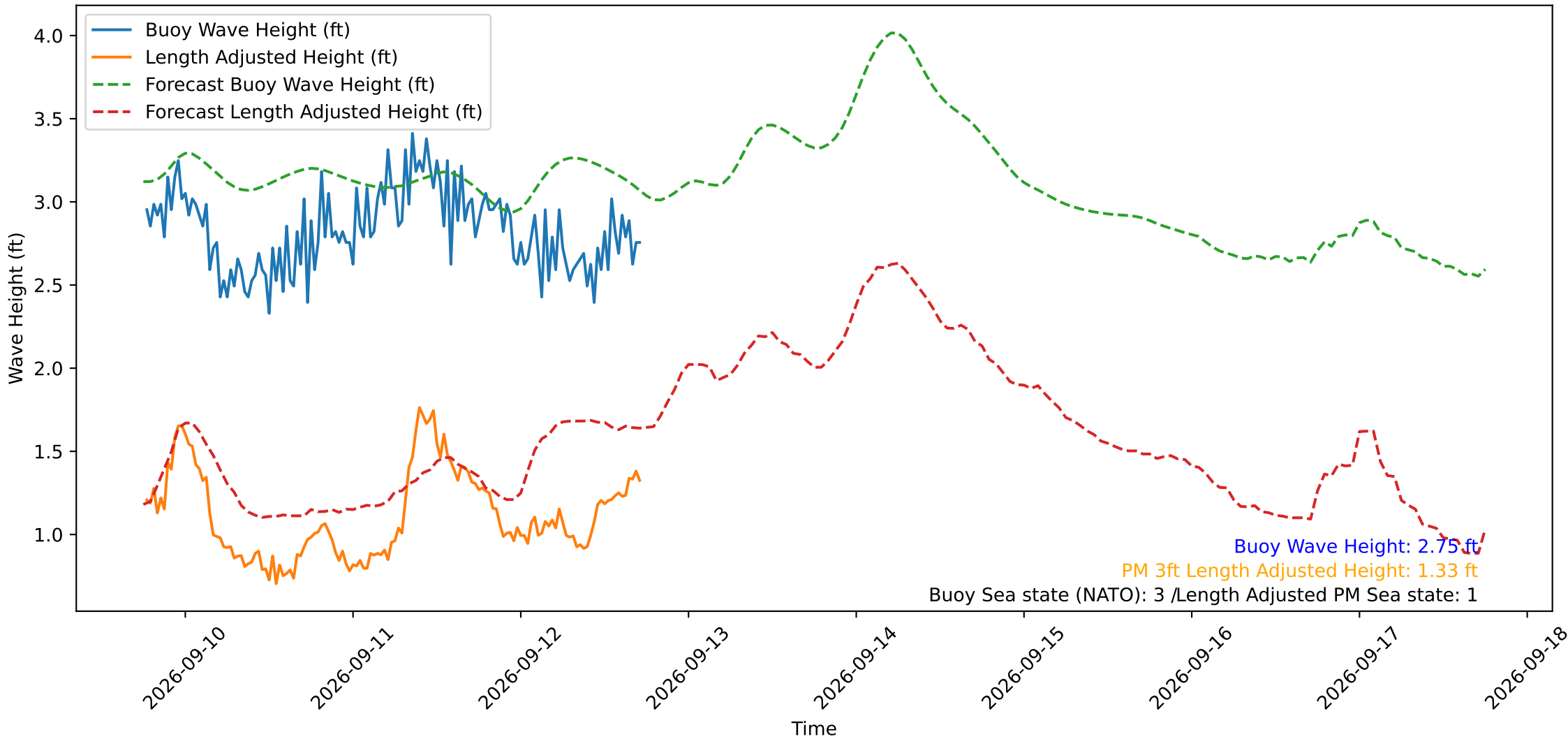
Wave Heights over Time for Red Beach at 2026-09-12 18:00:52
