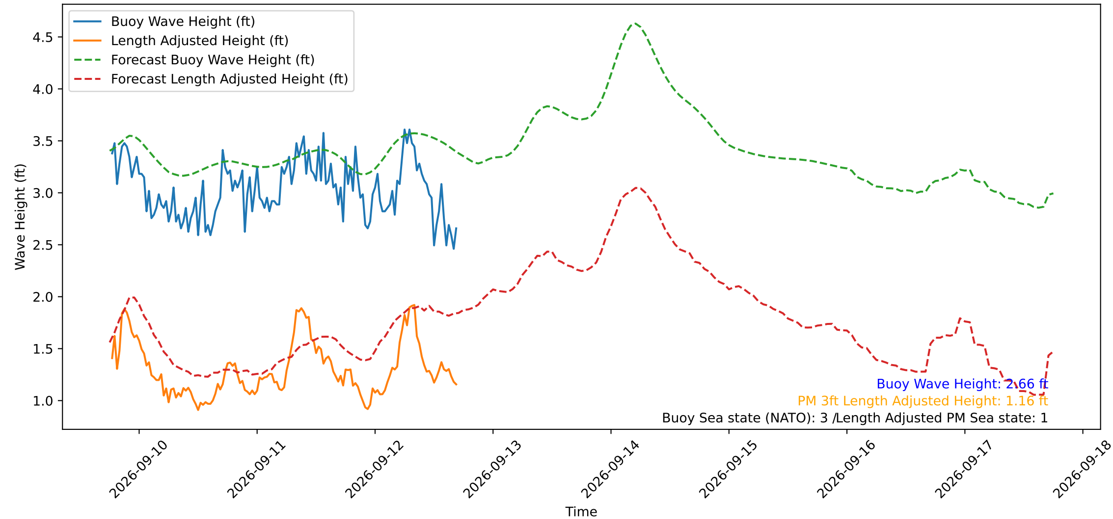
Wave Heights over Time for Green Beach at 2026-09-12 18:01:15
