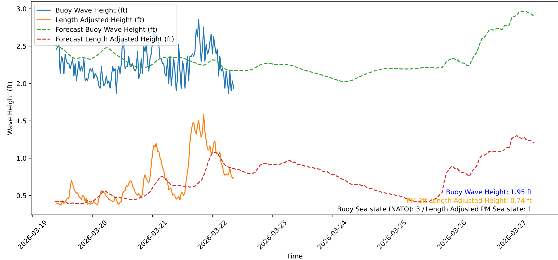
Wave Heights over Time for Red Beach at 2026-03-22 09:20:47
