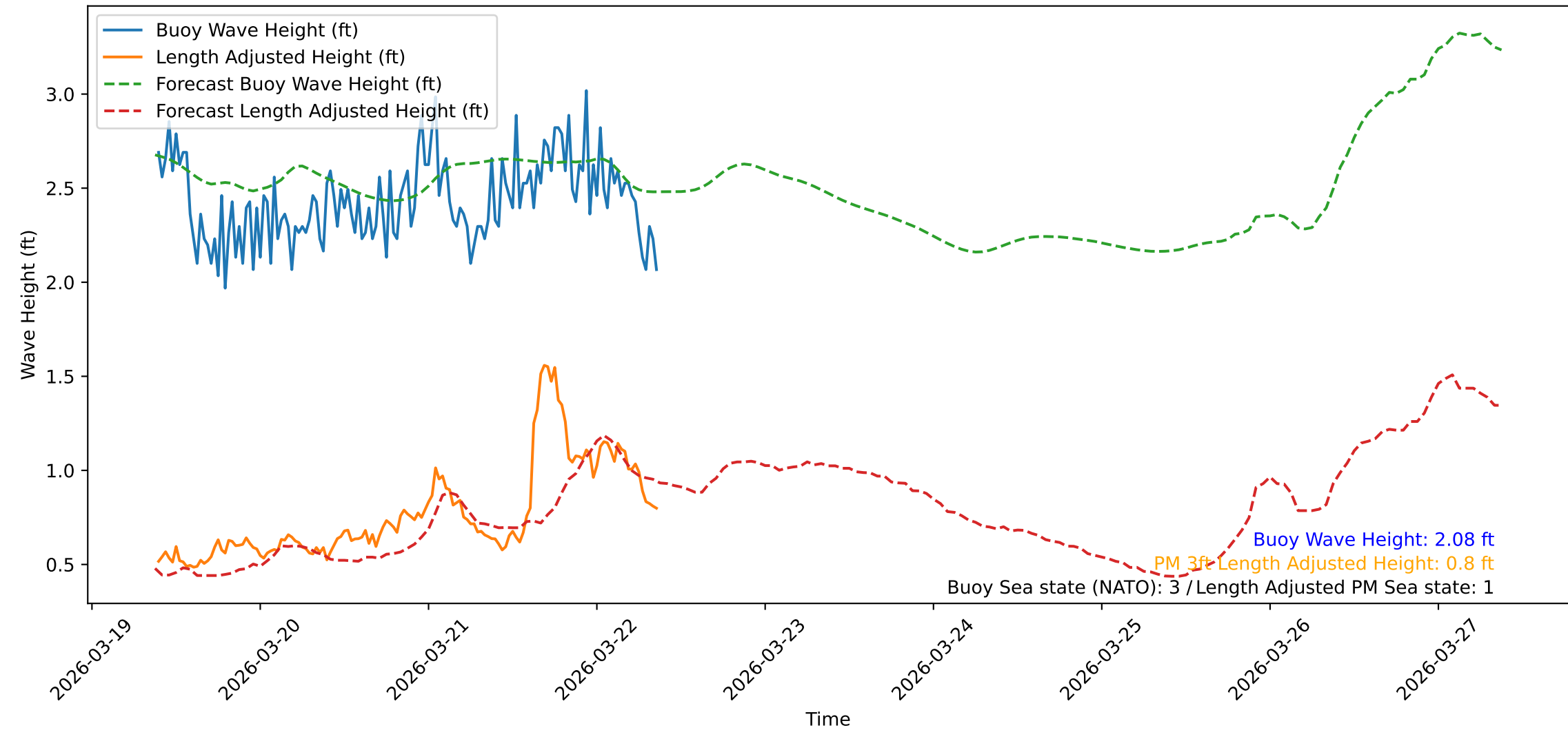
Wave Heights over Time for Oceanside Harbor at 2026-03-22 09:20:31
