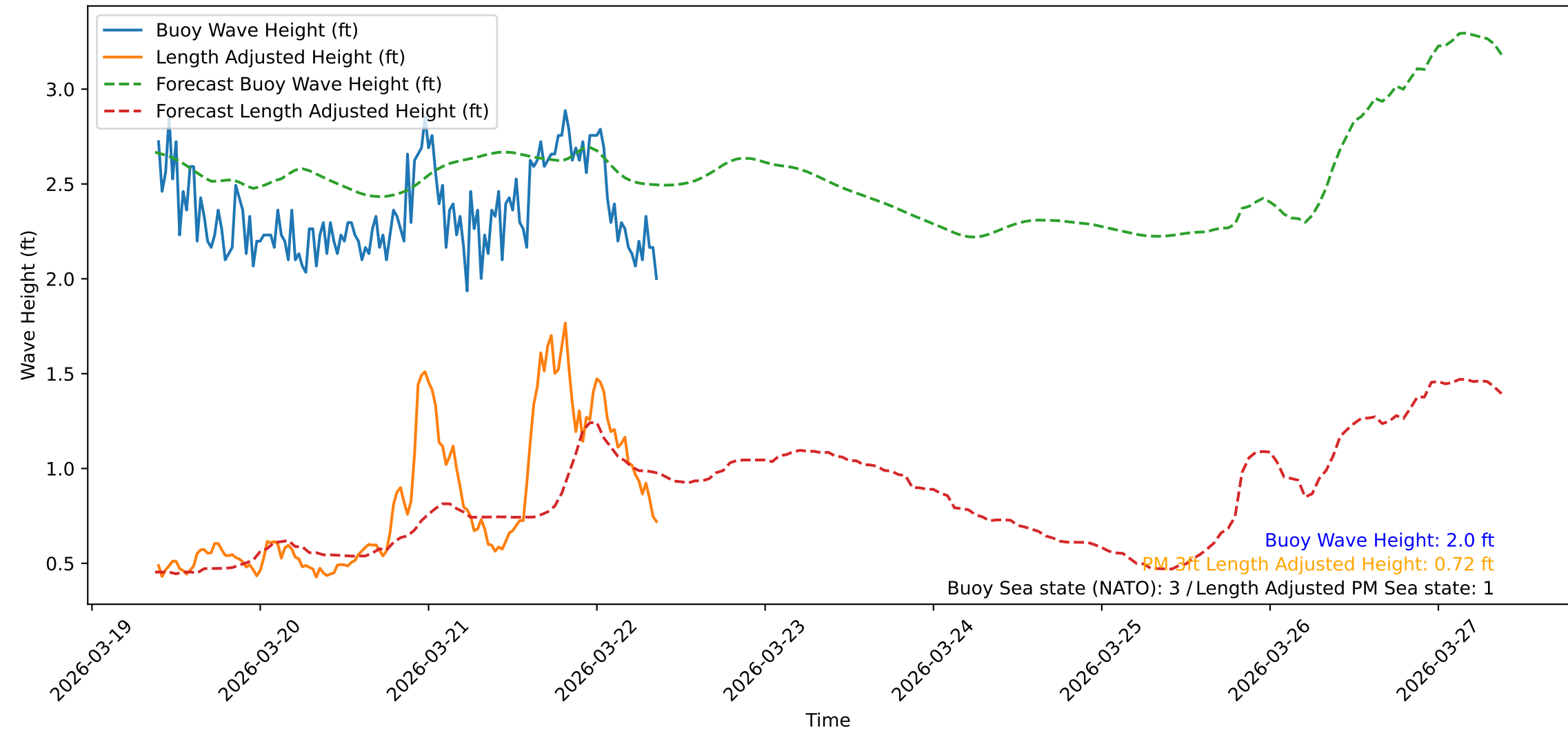
Wave Heights over Time for Green Beach at 2026-03-22 09:21:09
