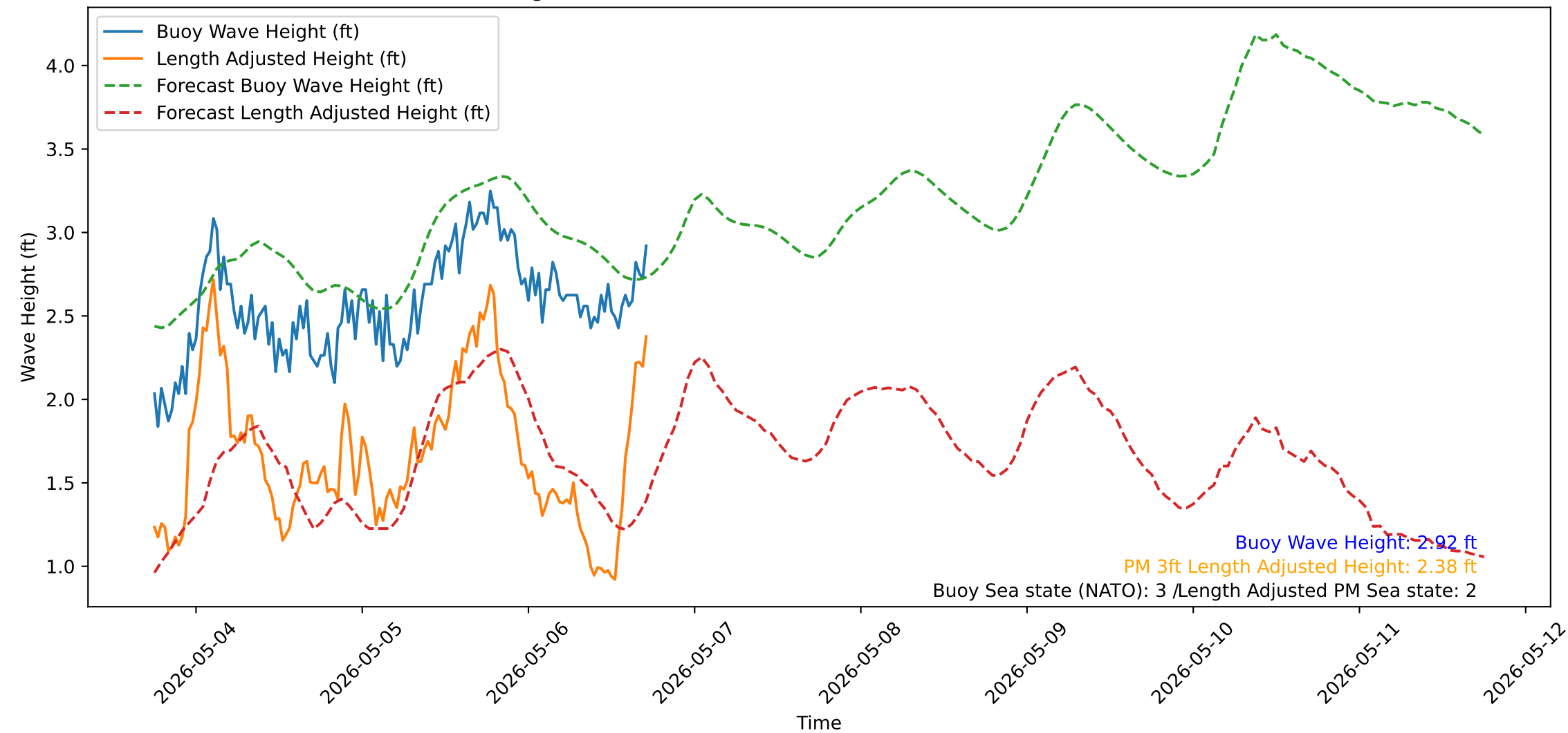
Wave Heights over Time for Oceanside Harbor at 2026-05-06 18:00:31
