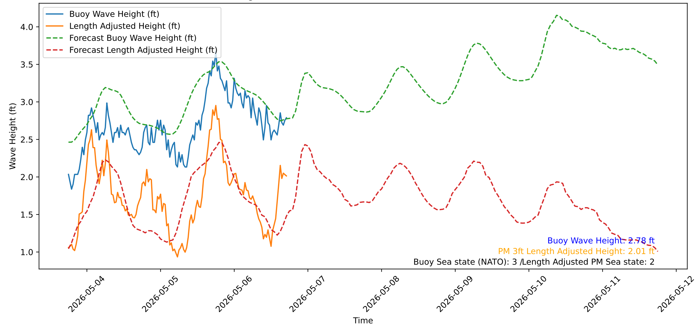
Wave Heights over Time for Green Beach at 2026-05-06 18:01:13
