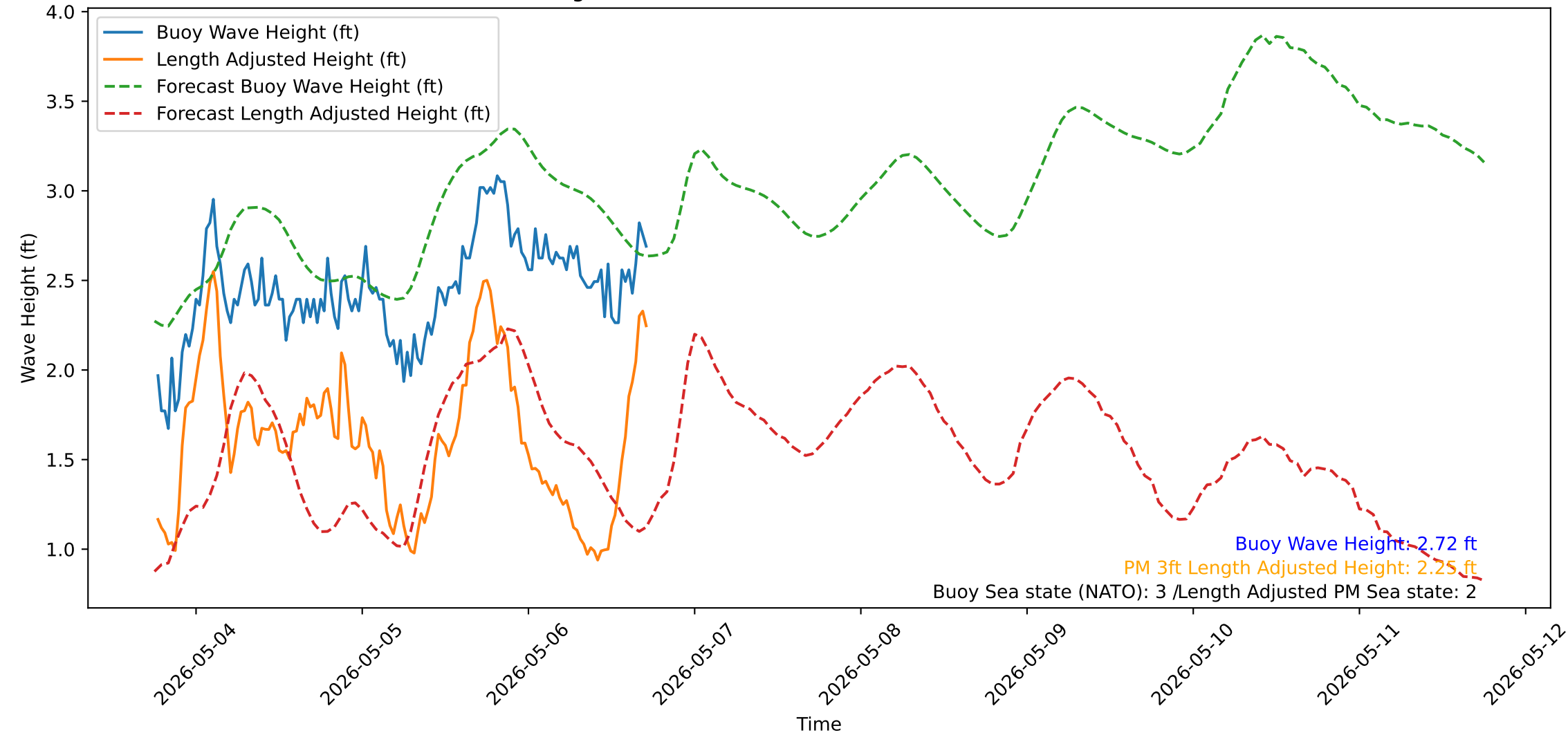
Wave Heights over Time for Red Beach at 2026-05-06 18:00:50
