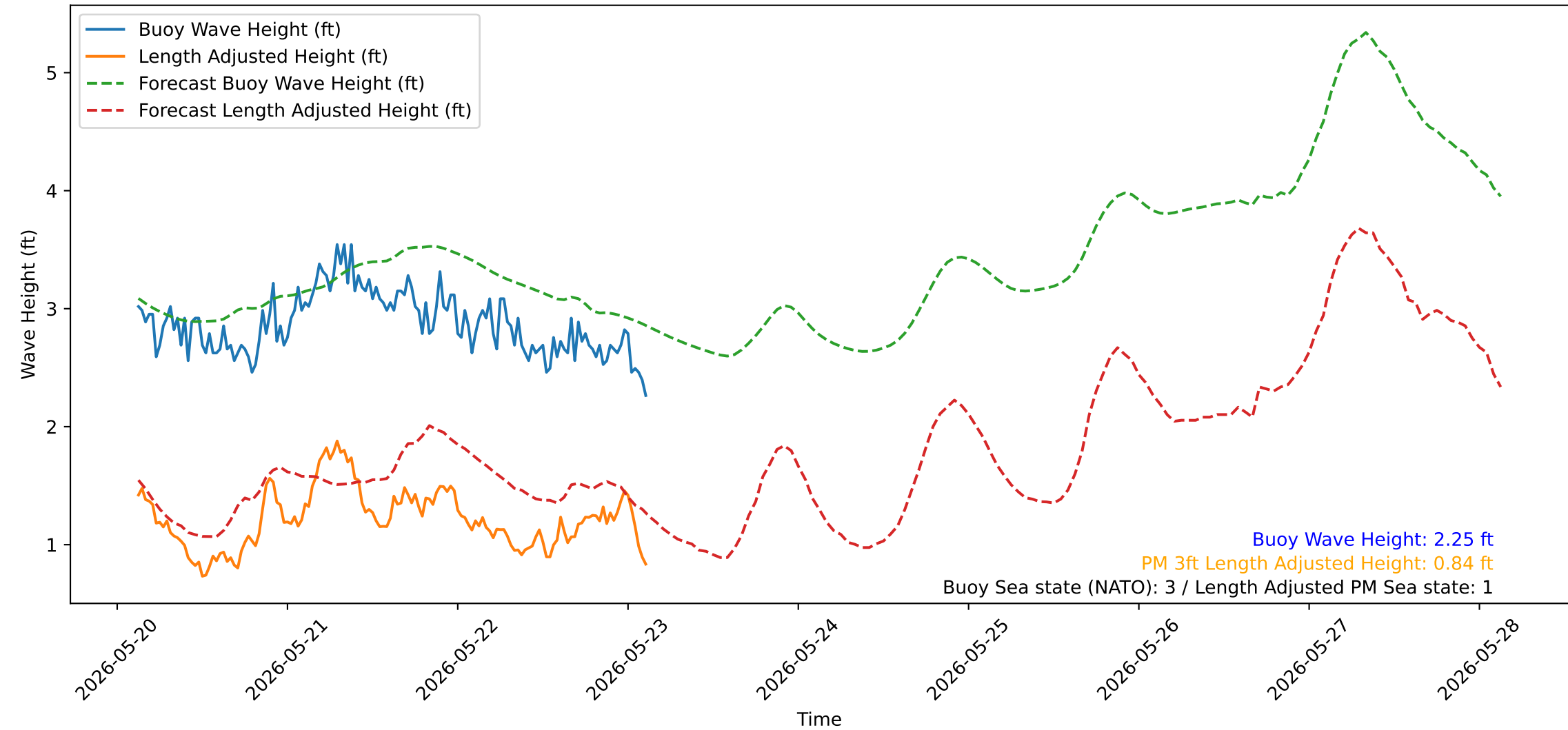
Wave Heights over Time for Green Beach at 2026-05-23 03:11:13
