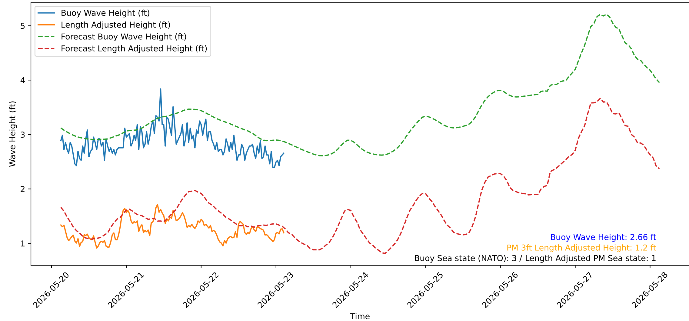
Wave Heights over Time for Oceanside Harbor at 2026-05-23 03:10:32
