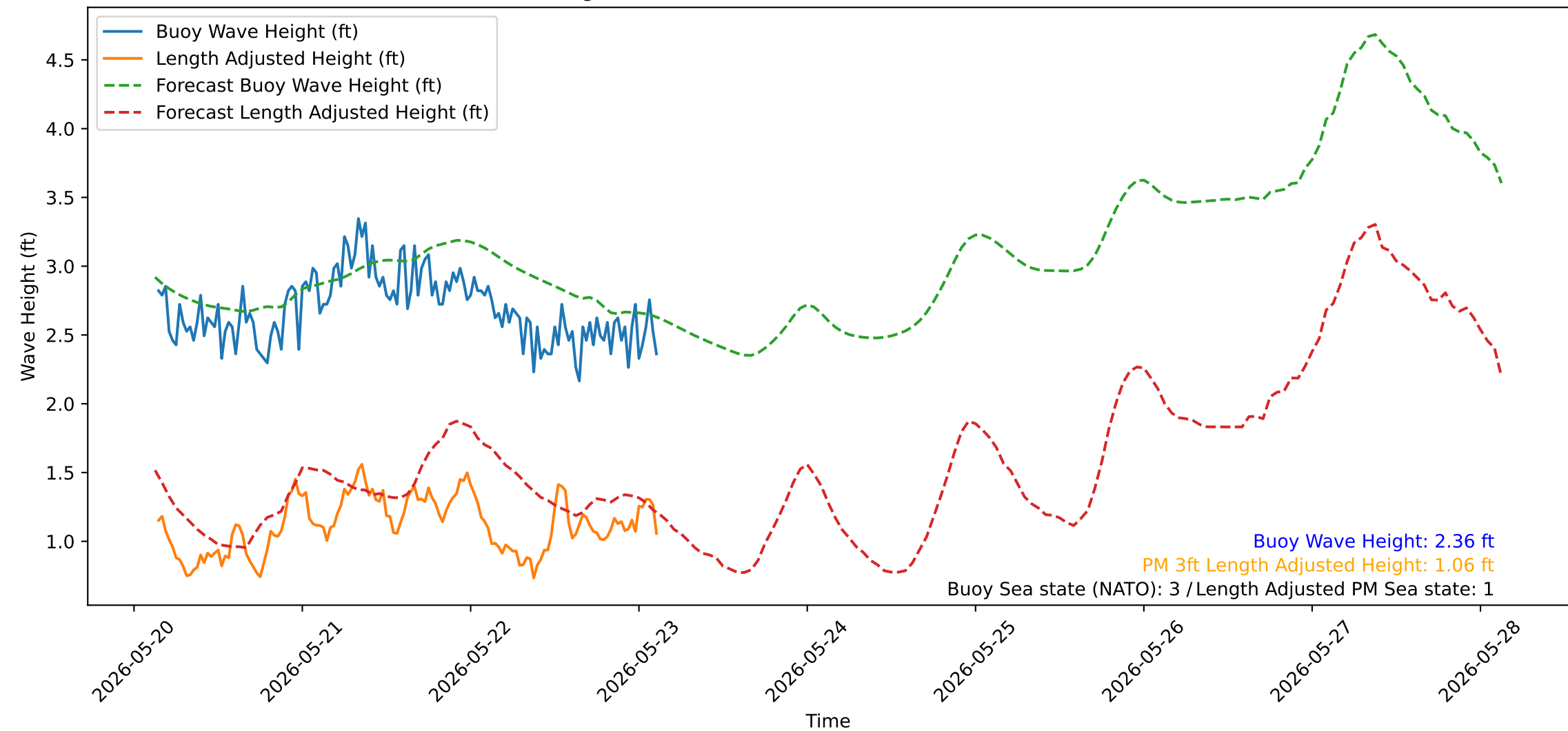
Wave Heights over Time for Red Beach at 2026-05-23 03:10:51
