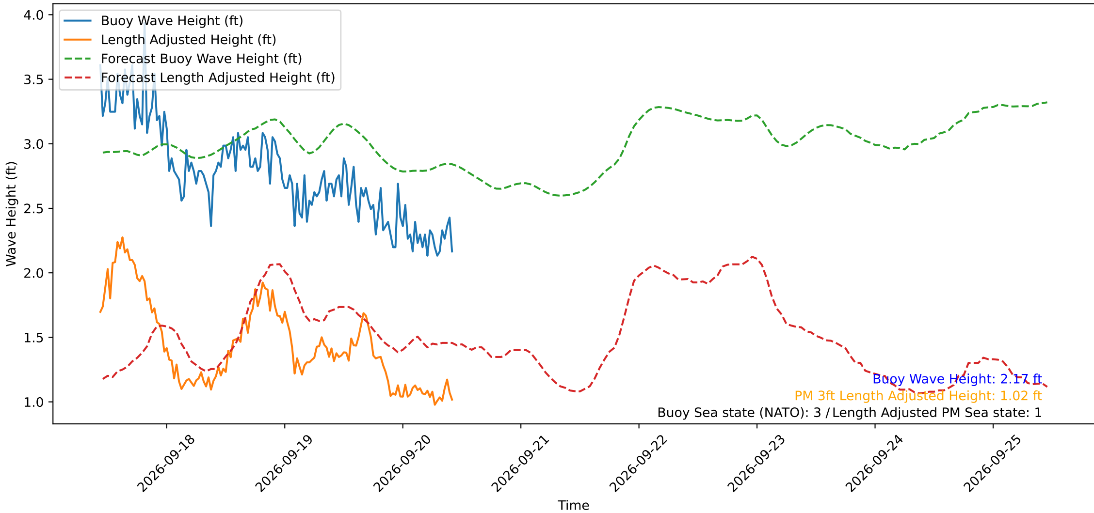
Wave Heights over Time for Oceanside Harbor at 2026-09-20 10:40:29
