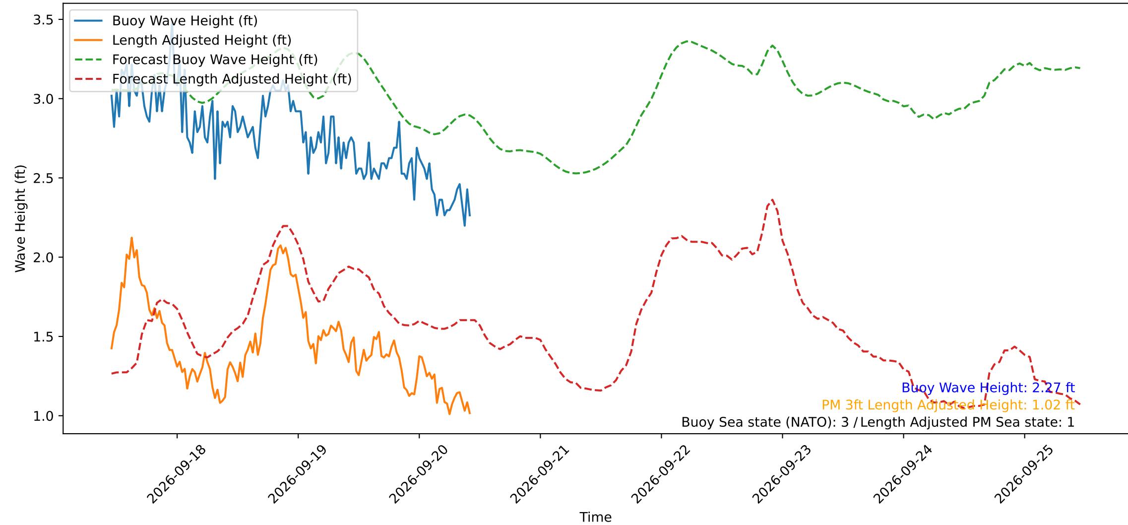
Wave Heights over Time for Green Beach at 2026-09-20 10:41:10
