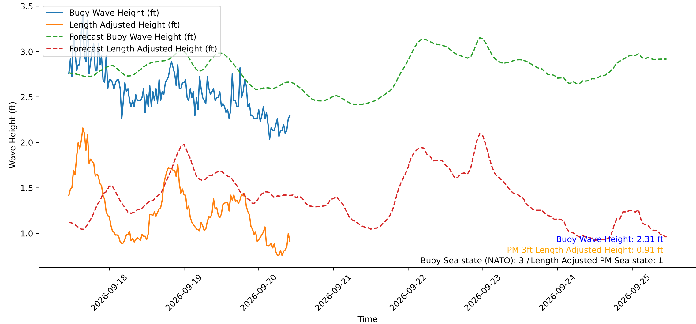
Wave Heights over Time for Red Beach at 2026-09-20 10:40:48
