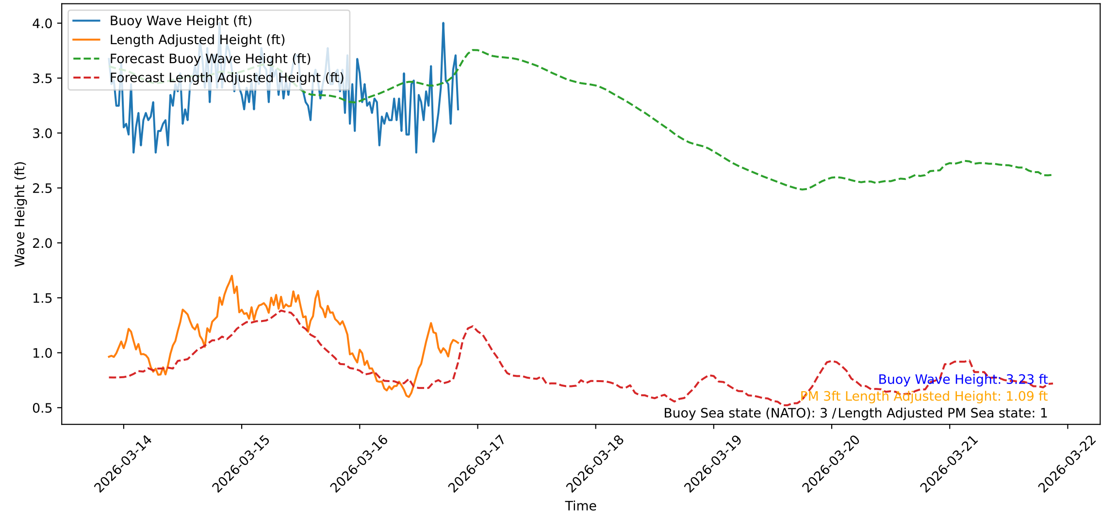
Wave Heights over Time for Green Beach at 2026-03-16 20:51:41
