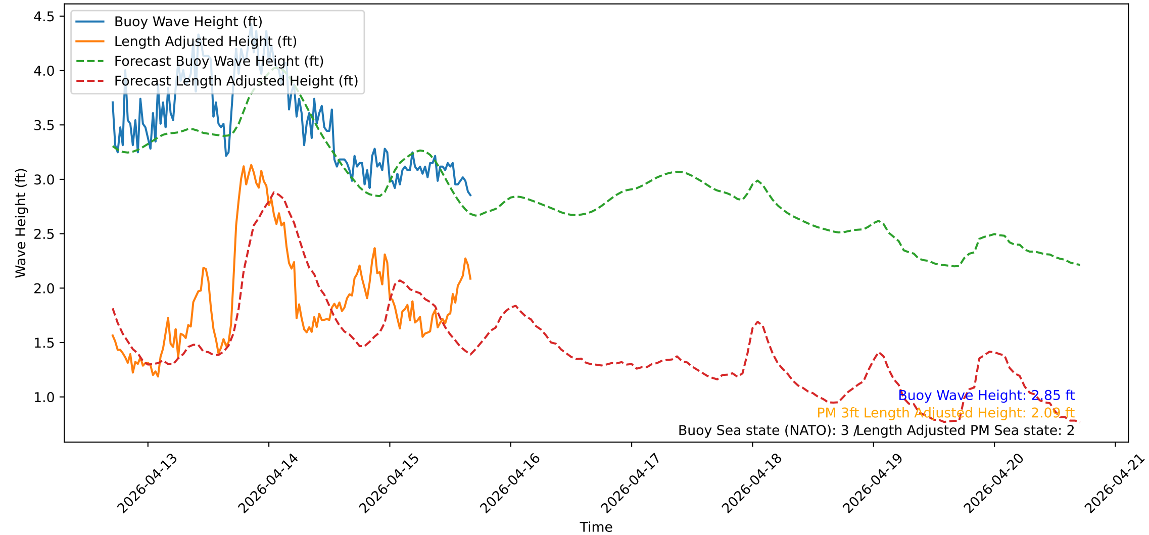
Wave Heights over Time for Red Beach at 2026-04-15 16:50:52
