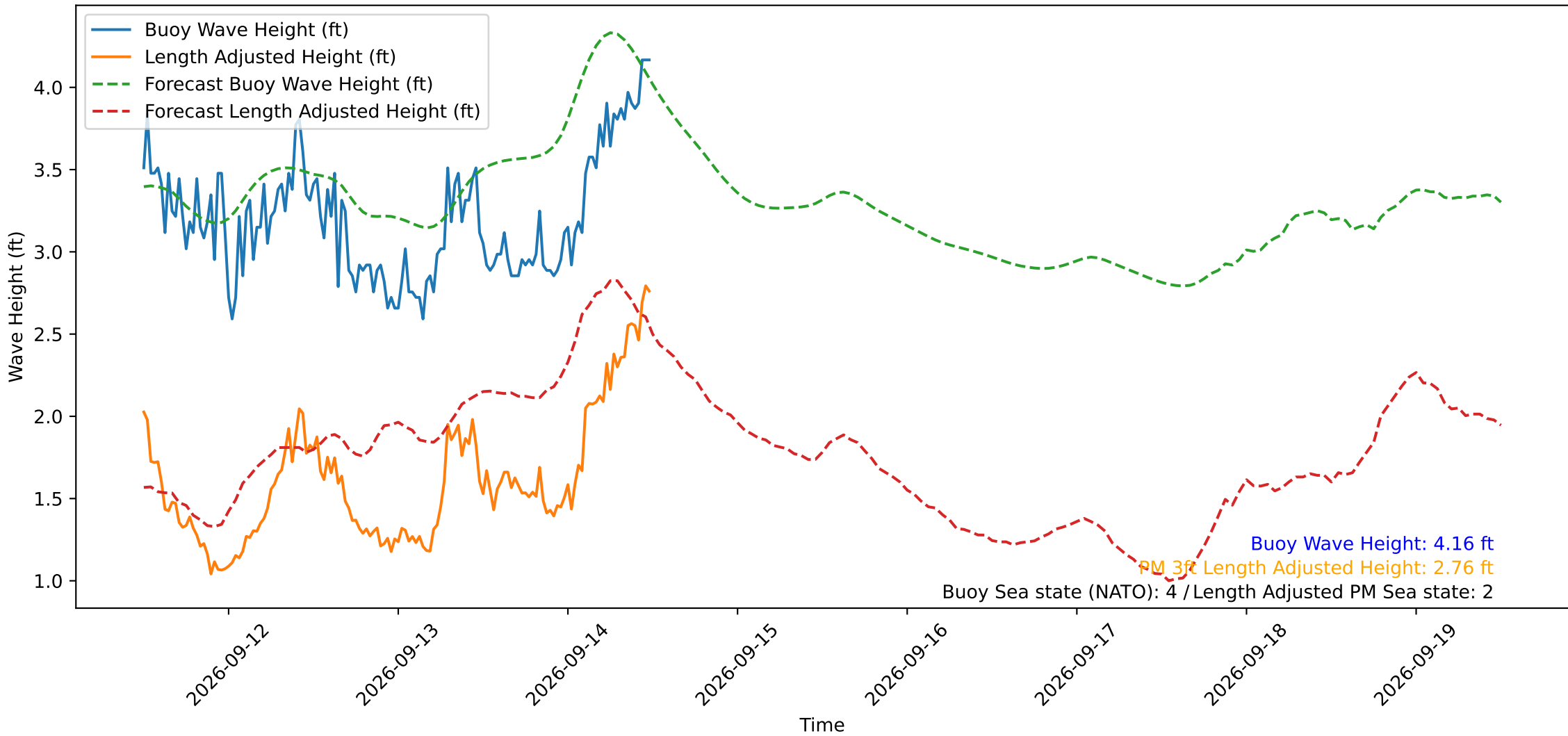
Wave Heights over Time for Oceanside Harbor at 2026-09-14 12:10:30
