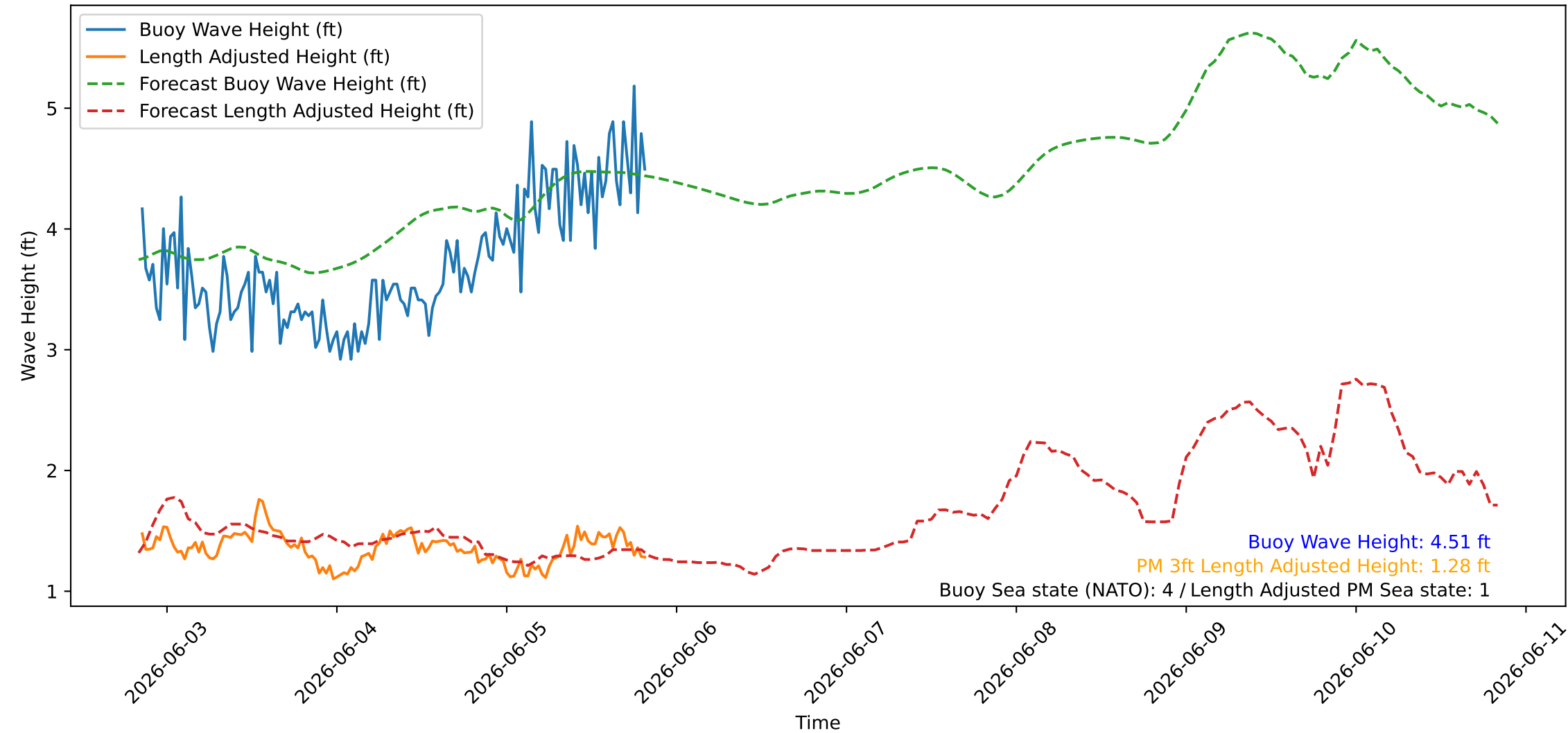
Wave Heights over Time for Oceanside Harbor at 2026-06-05 20:20:25
