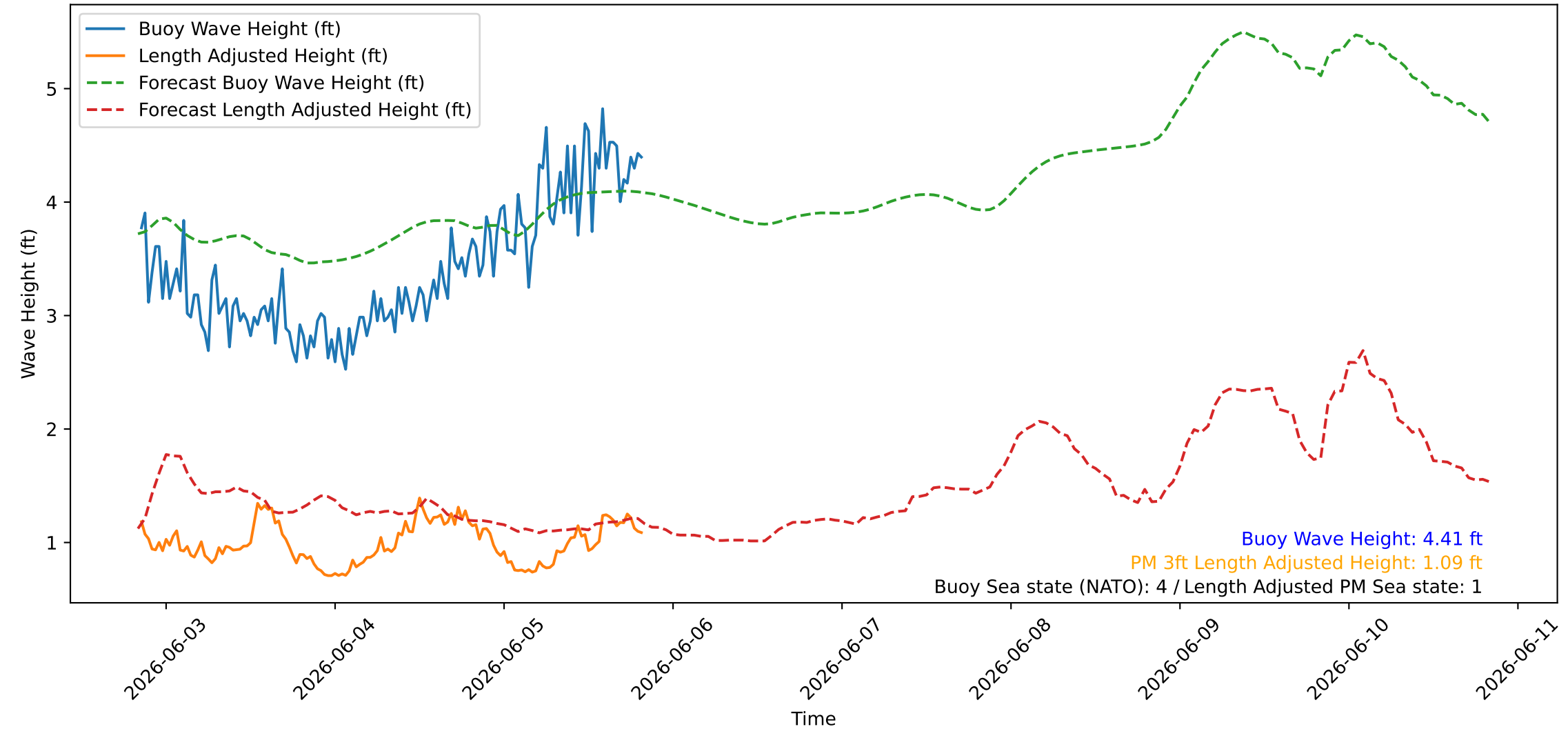
Wave Heights over Time for Red Beach at 2026-06-05 20:20:46
