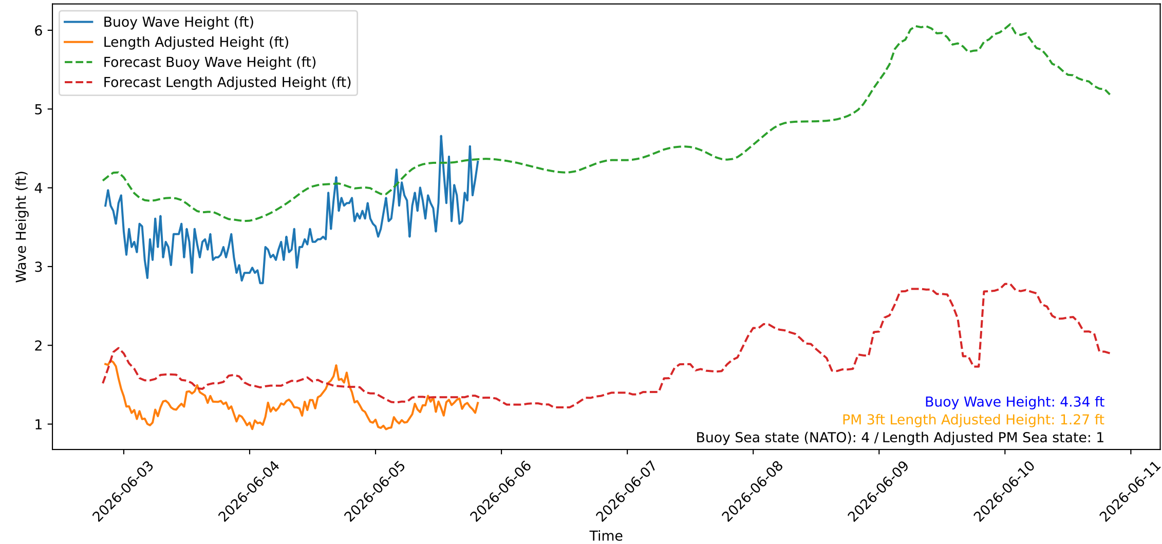
Wave Heights over Time for Green Beach at 2026-06-05 20:21:08
