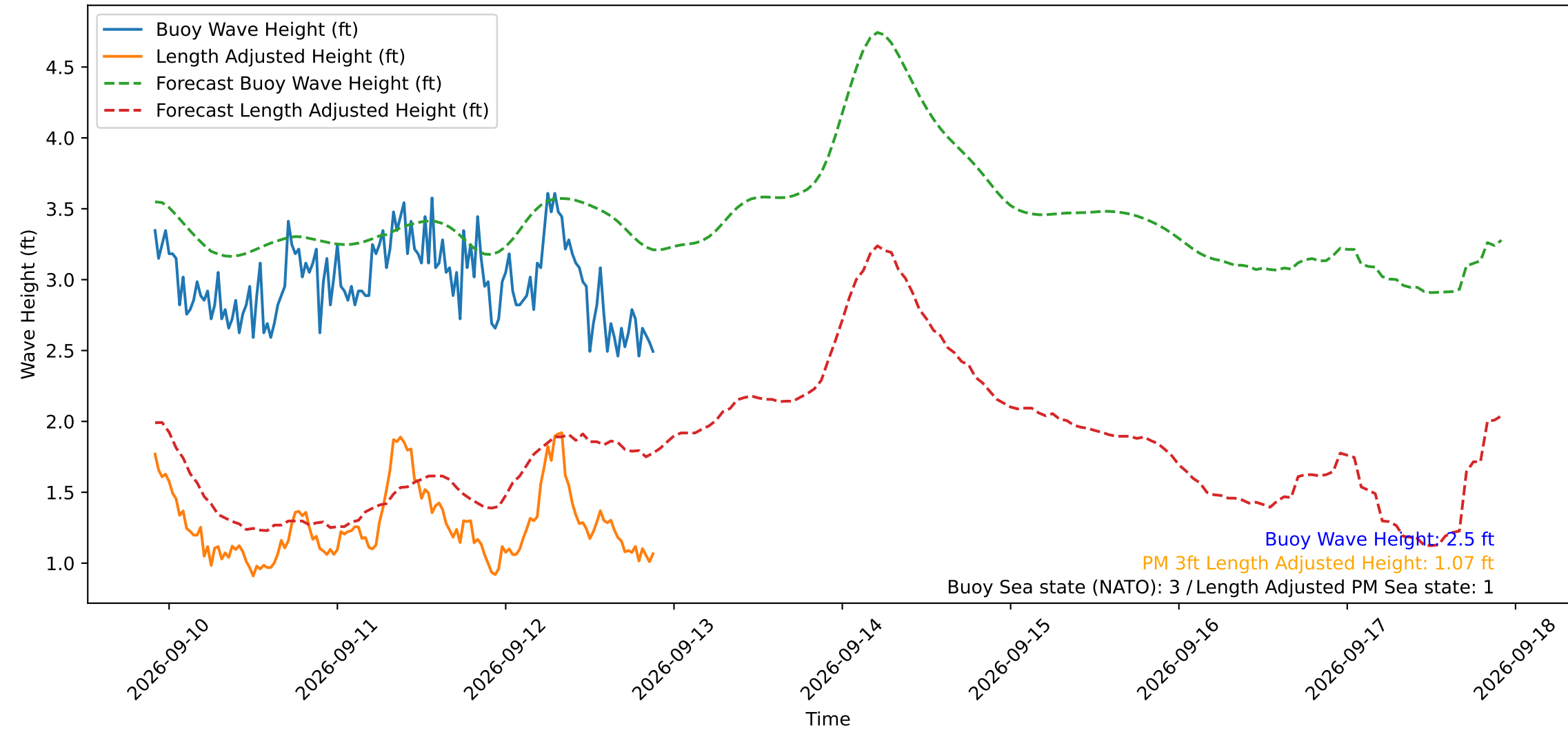
Wave Heights over Time for Green Beach at 2026-09-12 21:41:12
