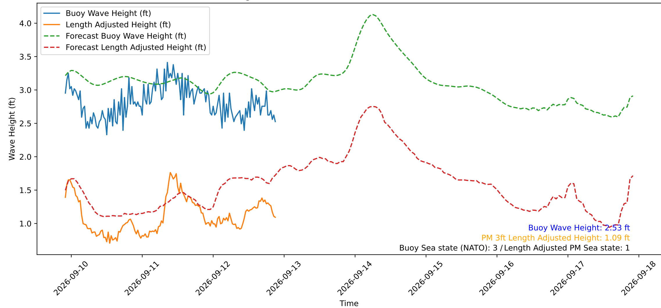
Wave Heights over Time for Red Beach at 2026-09-12 21:40:49
