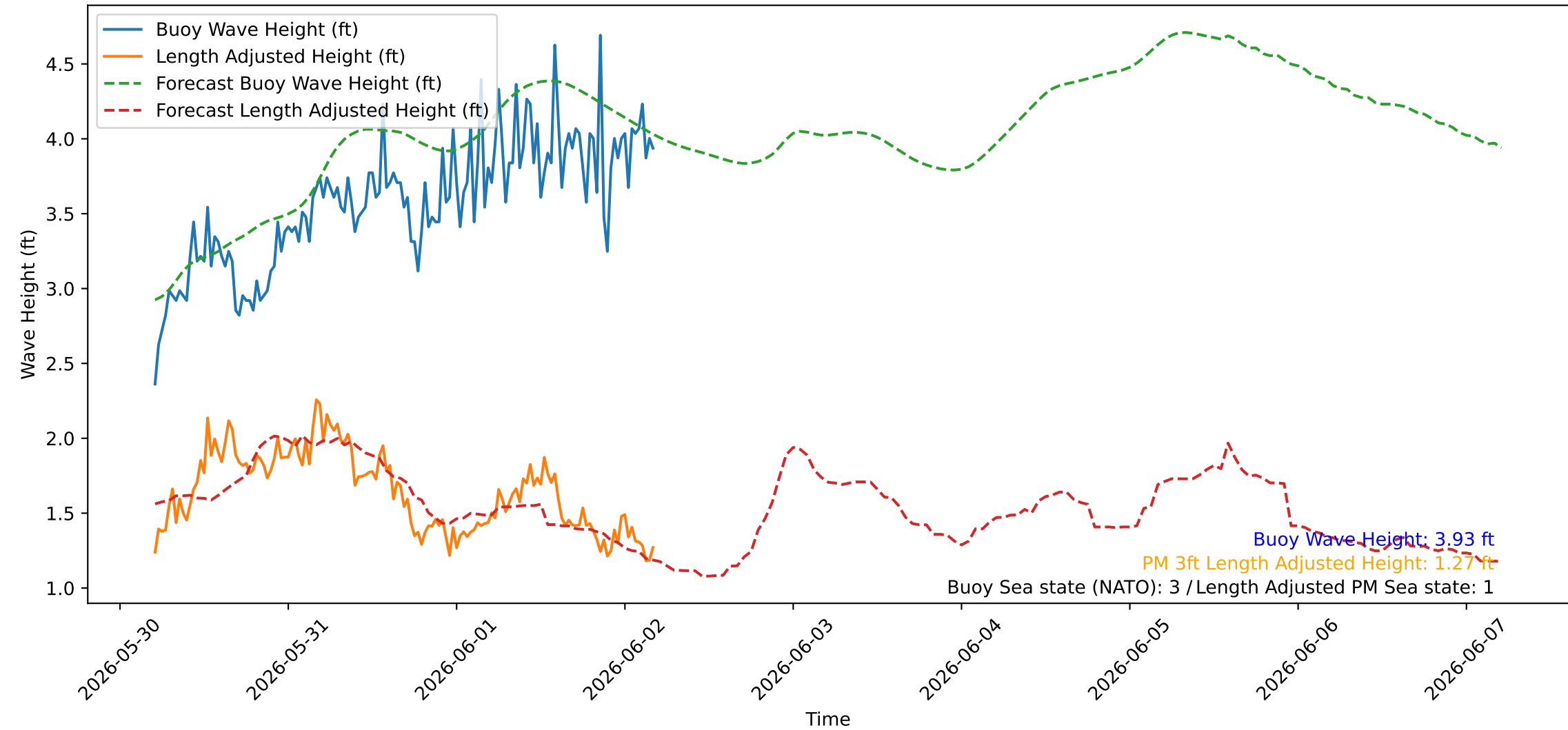
Wave Heights over Time for Oceanside Harbor at 2026-06-02 04:50:26
