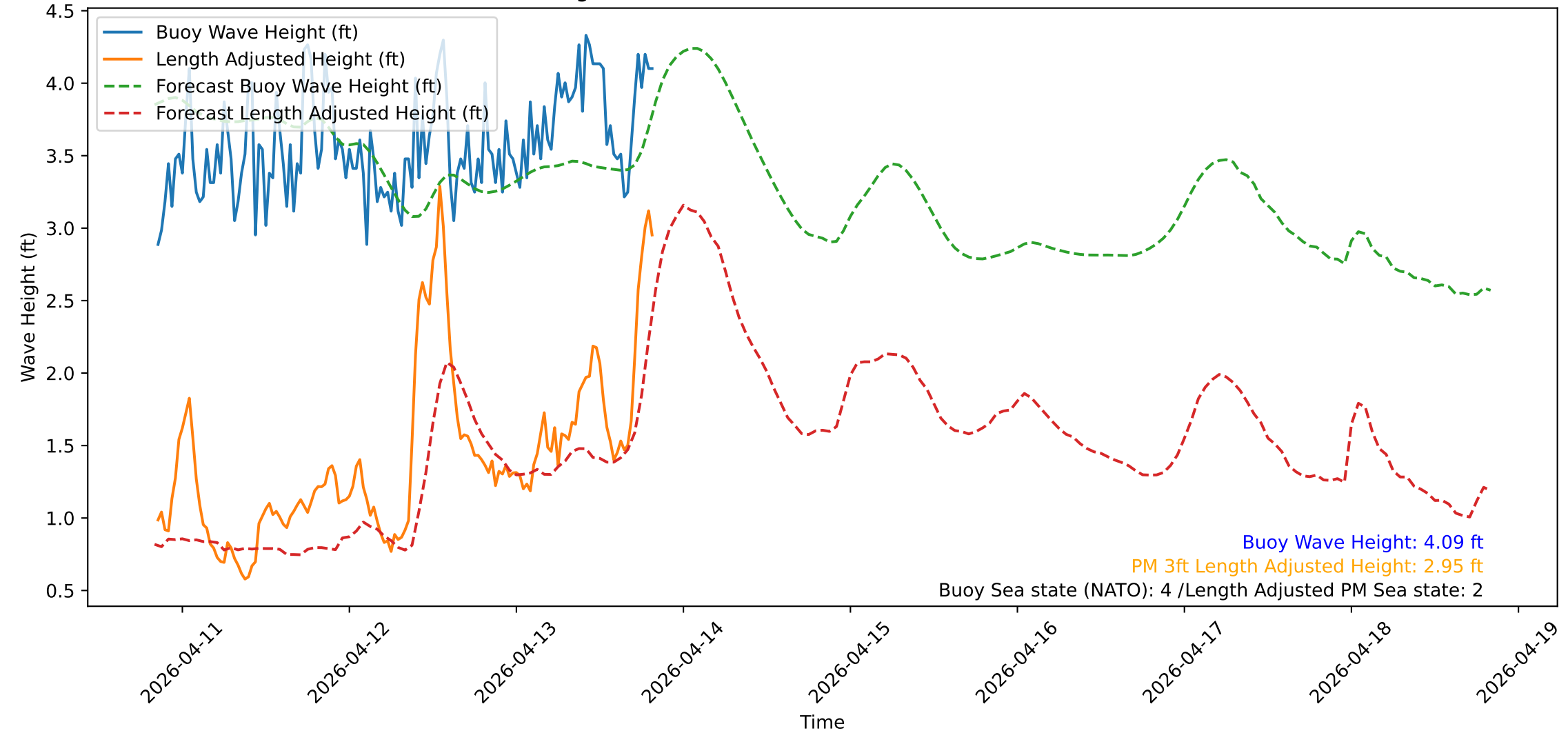
Wave Heights over Time for Red Beach at 2026-04-13 20:20:52
