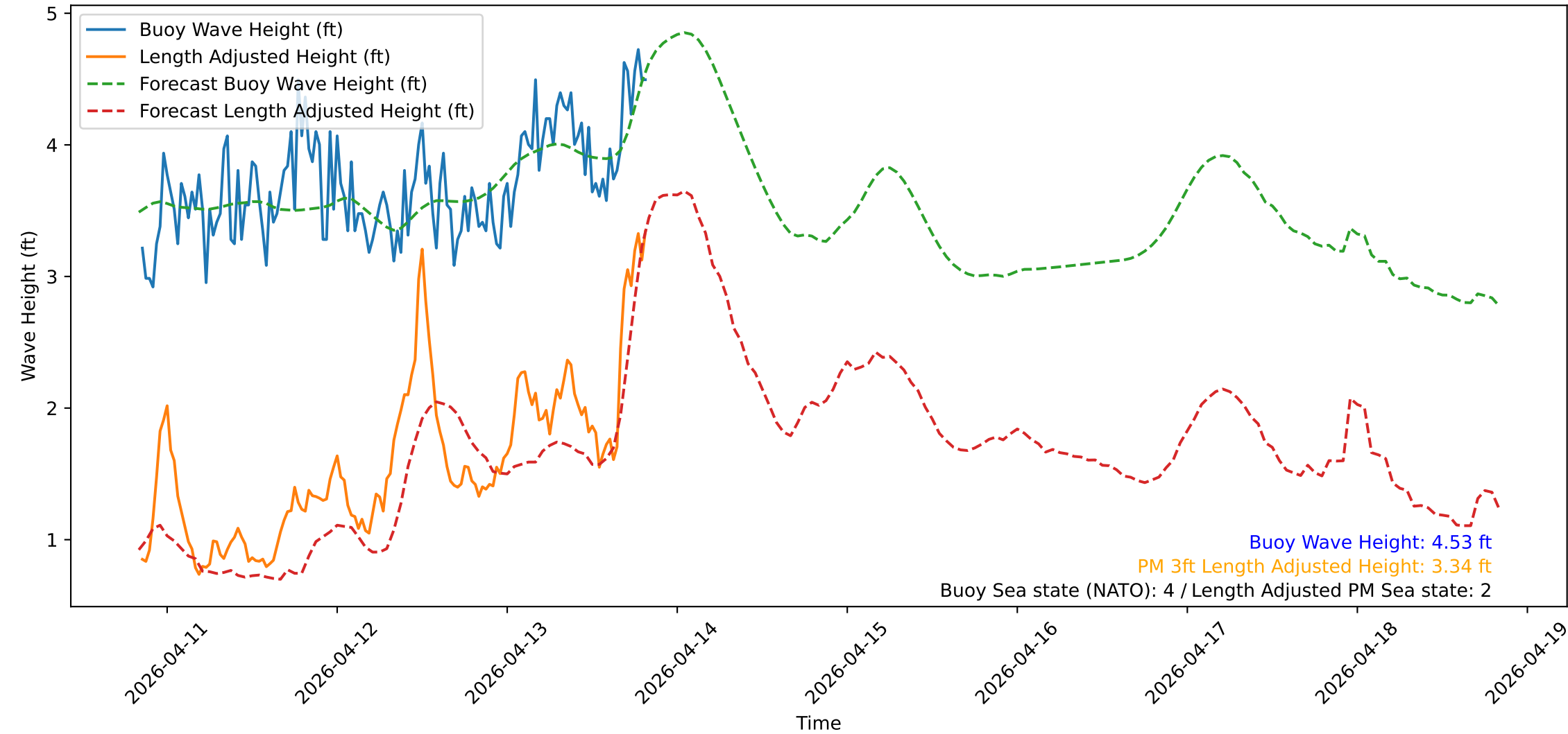
Wave Heights over Time for Green Beach at 2026-04-13 20:21:15
