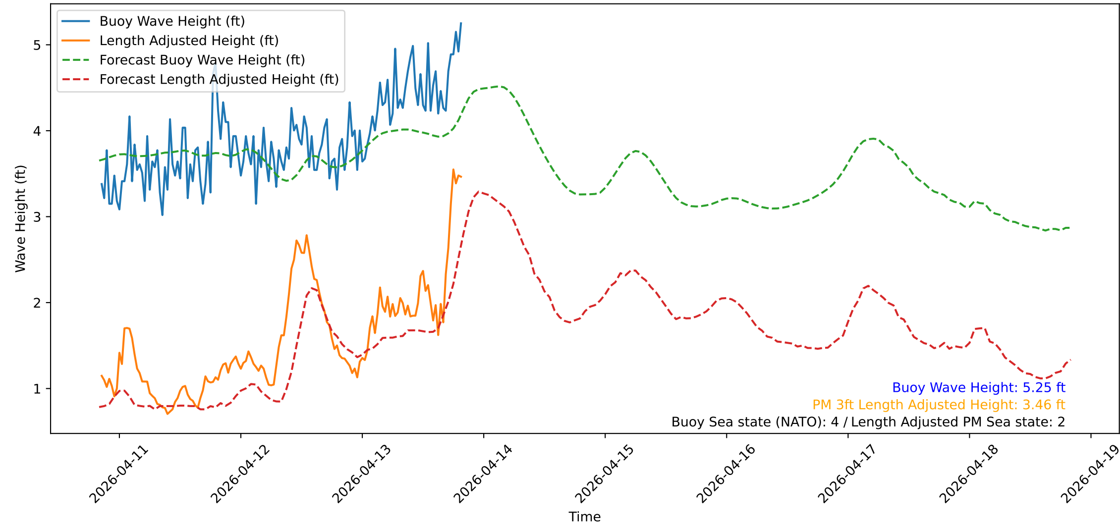
Wave Heights over Time for Oceanside Harbor at 2026-04-13 20:20:32
