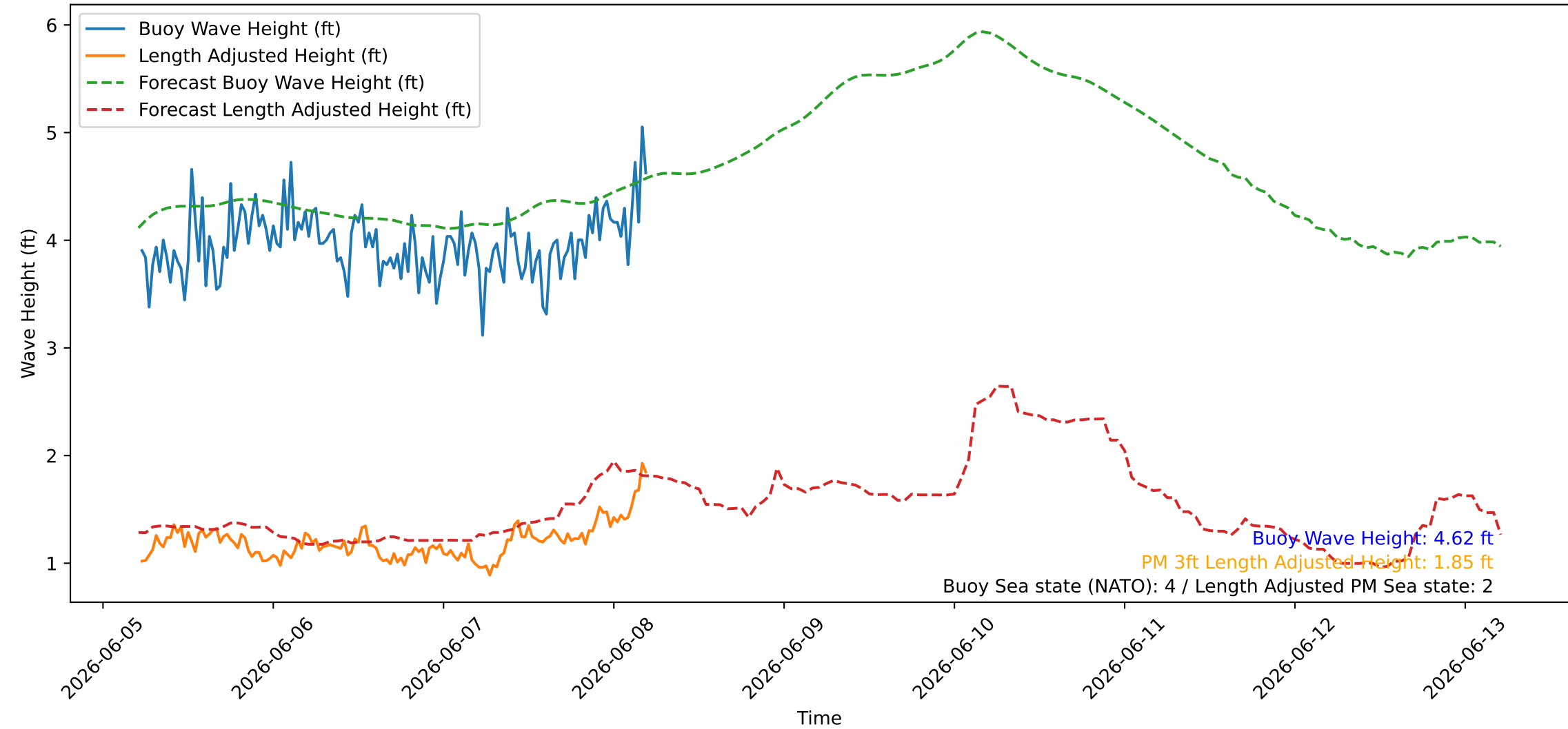
Wave Heights over Time for Green Beach at 2026-06-08 05:21:09
