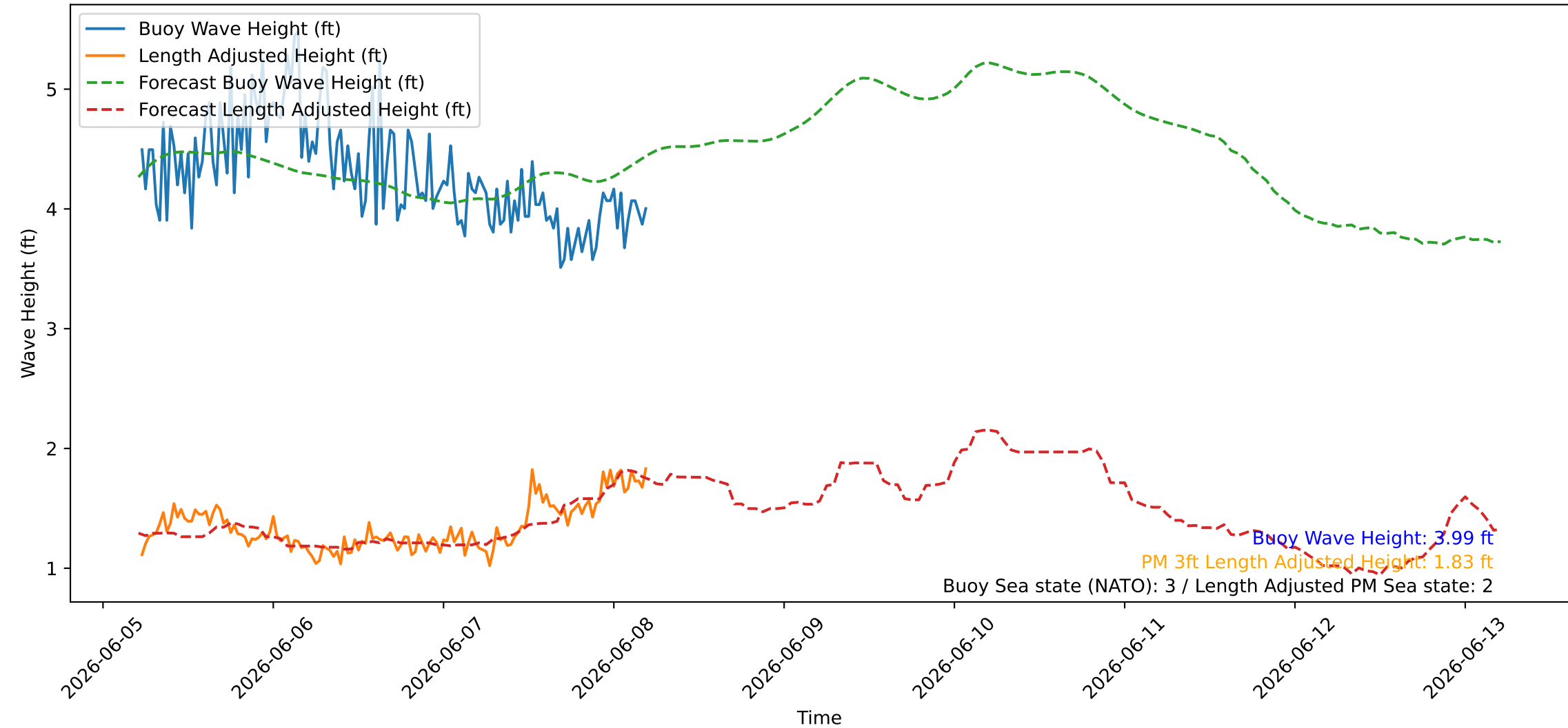
Wave Heights over Time for Oceanside Harbor at 2026-06-08 05:20:26
