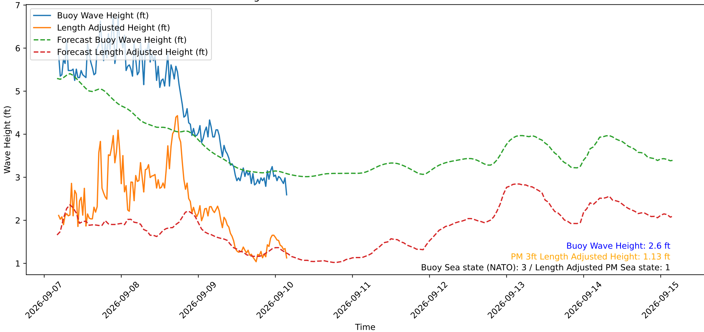
Wave Heights over Time for Red Beach at 2026-09-10 04:20:51
