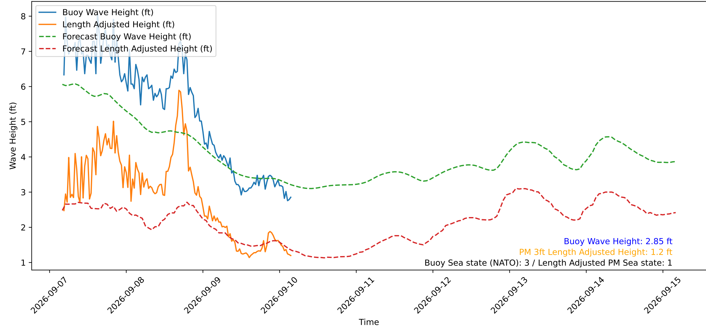
Wave Heights over Time for Green Beach at 2026-09-10 04:21:14
