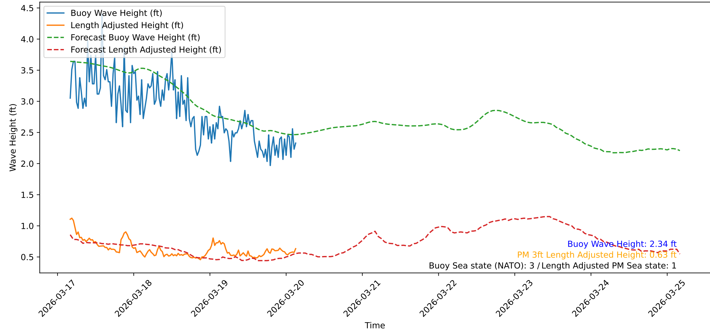
Wave Heights over Time for Oceanside Harbor at 2026-03-20 03:50:31
