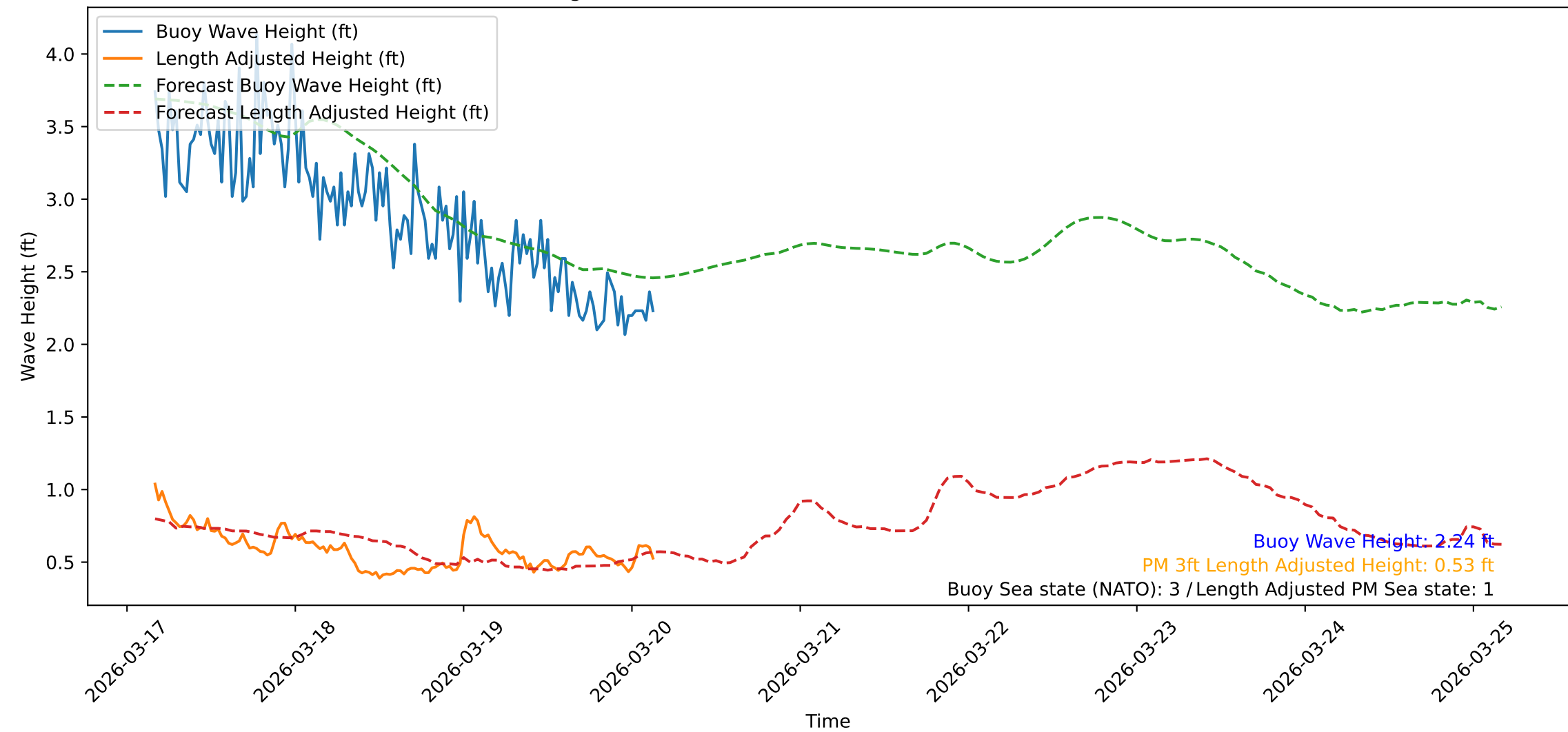
Wave Heights over Time for Green Beach at 2026-03-20 03:51:10
