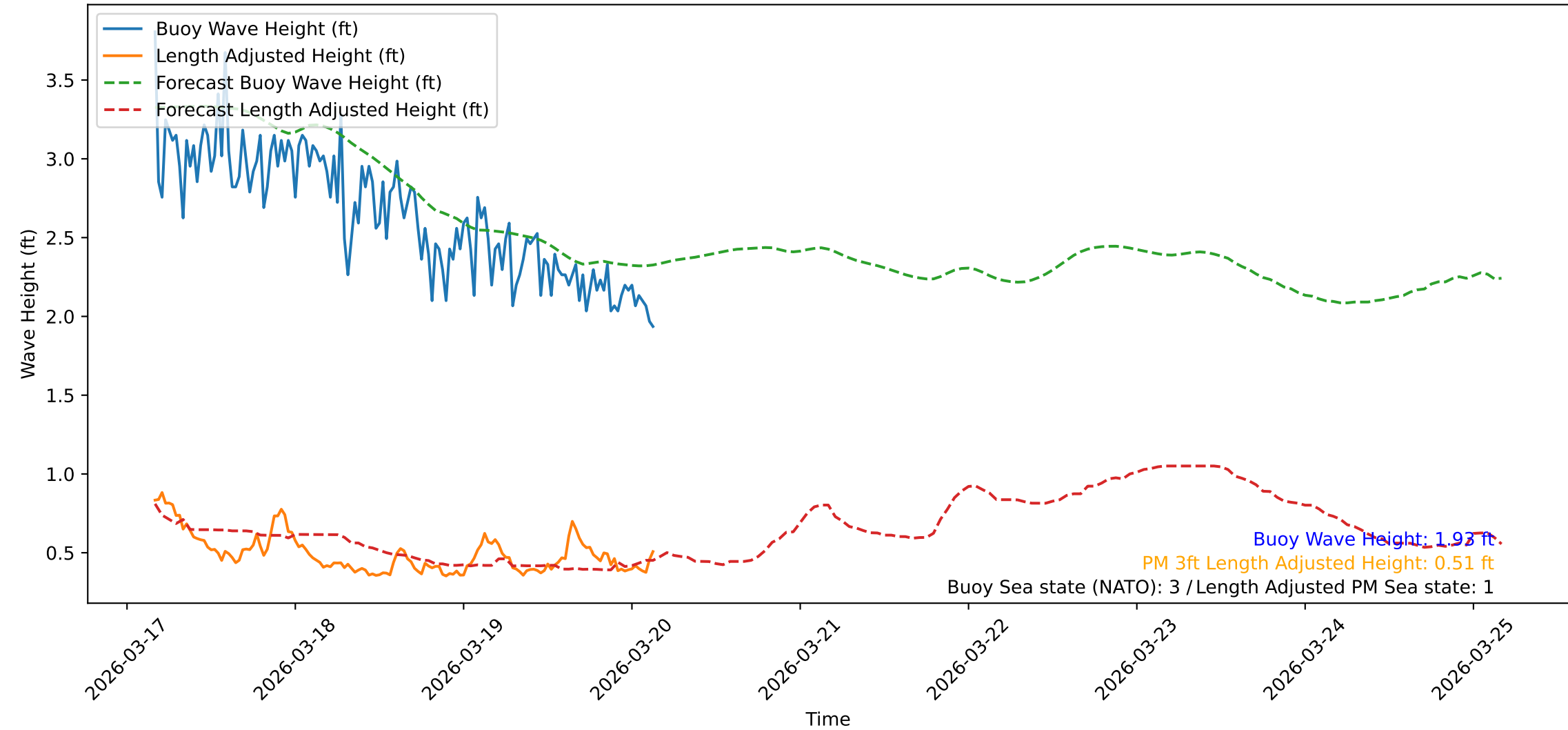
Wave Heights over Time for Red Beach at 2026-03-20 03:50:47
