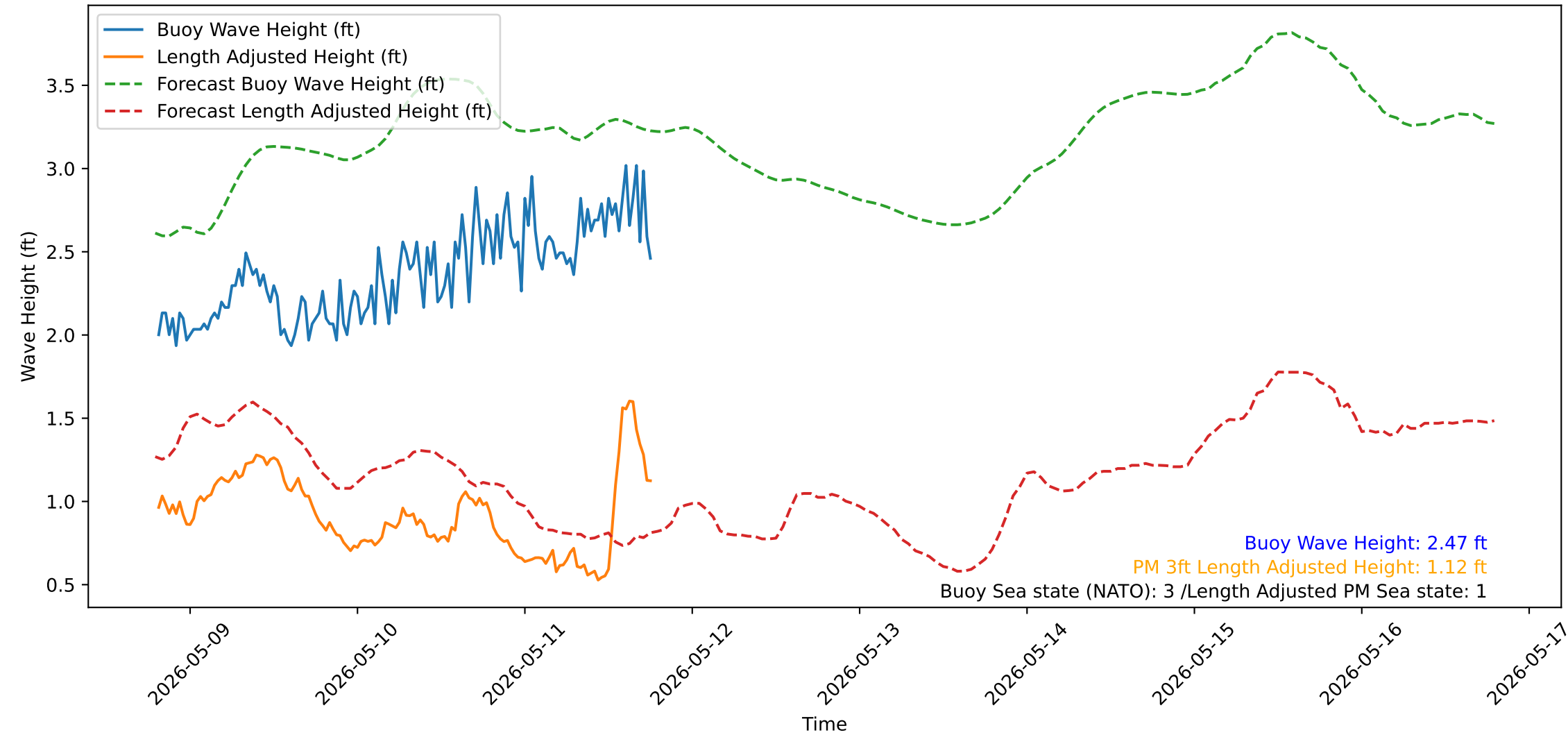
Wave Heights over Time for Red Beach at 2026-05-11 19:00:51
