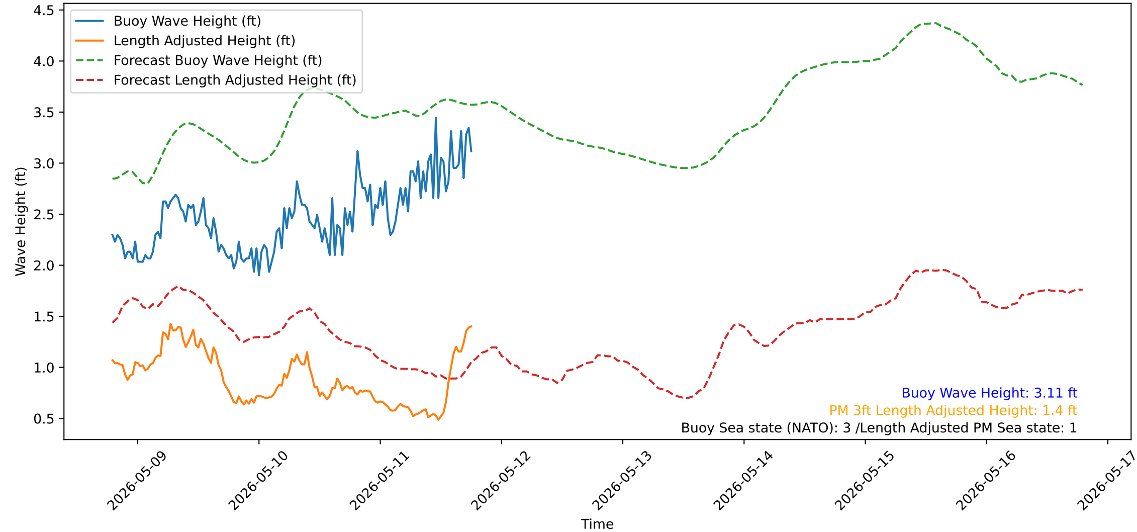
Wave Heights over Time for Green Beach at 2026-05-11 19:01:13
