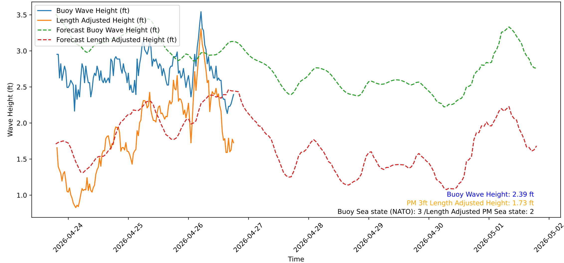
Wave Heights over Time for Red Beach at 2026-04-26 19:00:50
