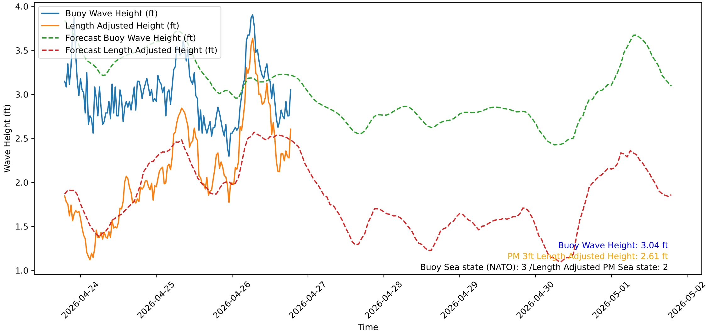
Wave Heights over Time for Oceanside Harbor at 2026-04-26 19:00:31
