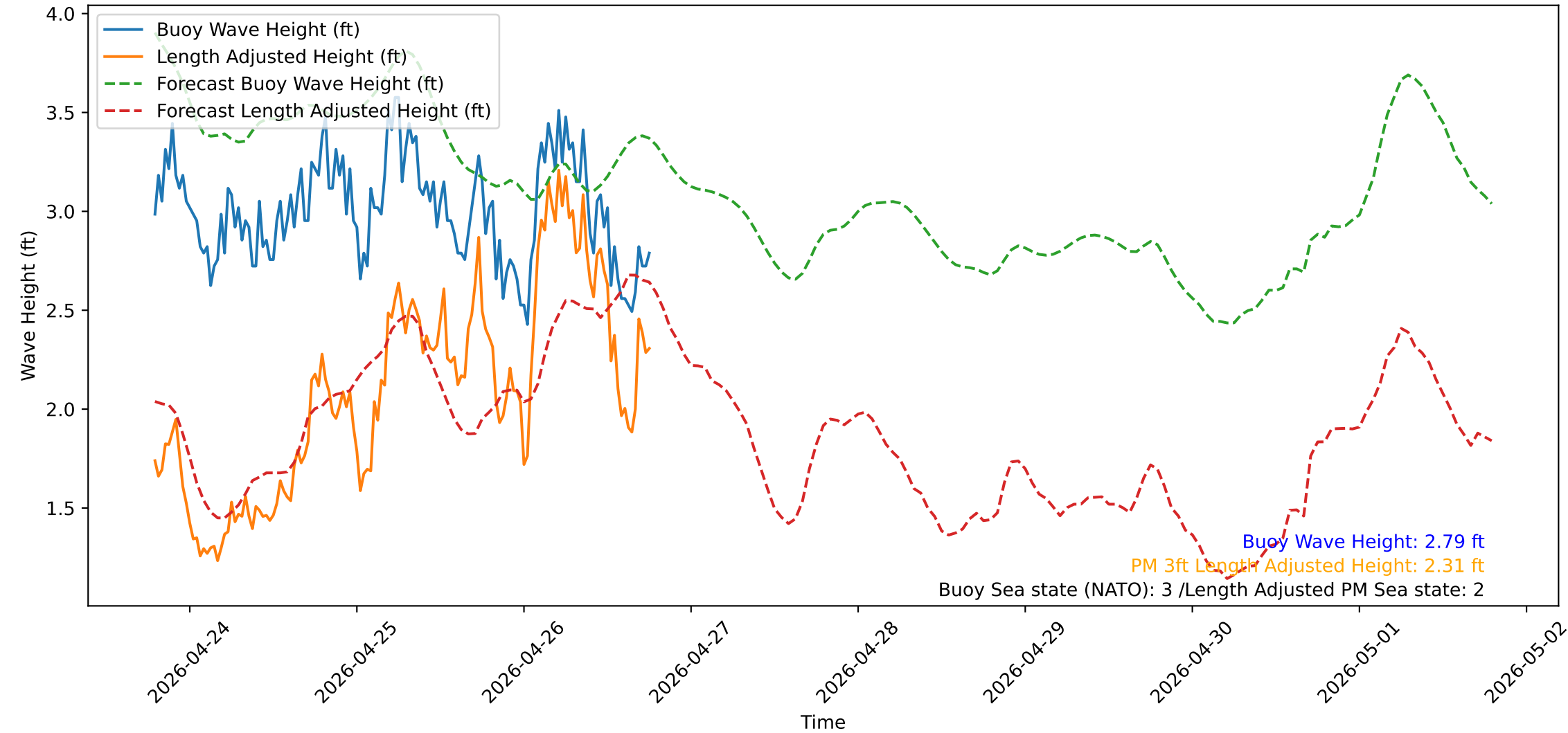
Wave Heights over Time for Green Beach at 2026-04-26 19:01:12
