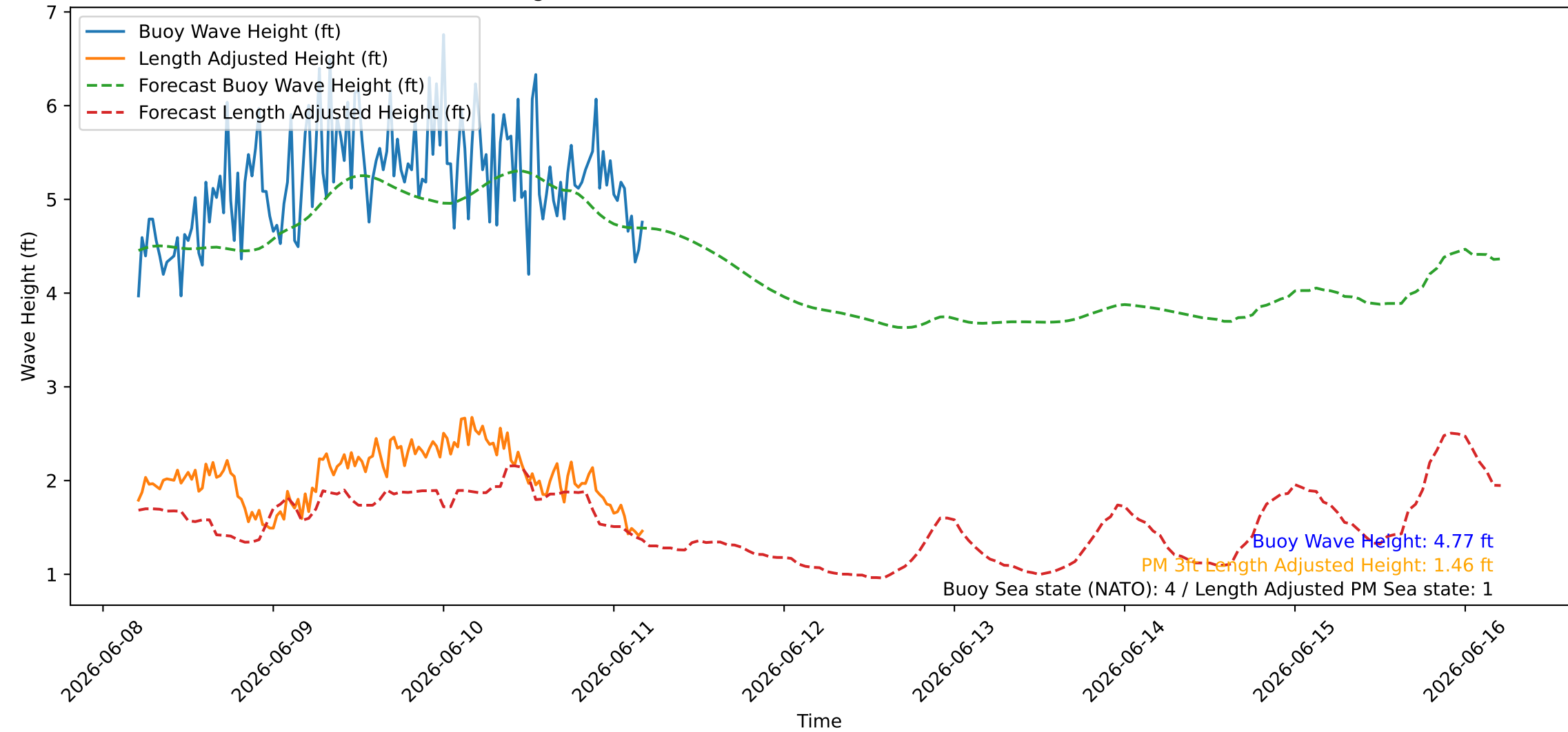
Wave Heights over Time for Oceanside Harbor at 2026-06-11 04:50:26
