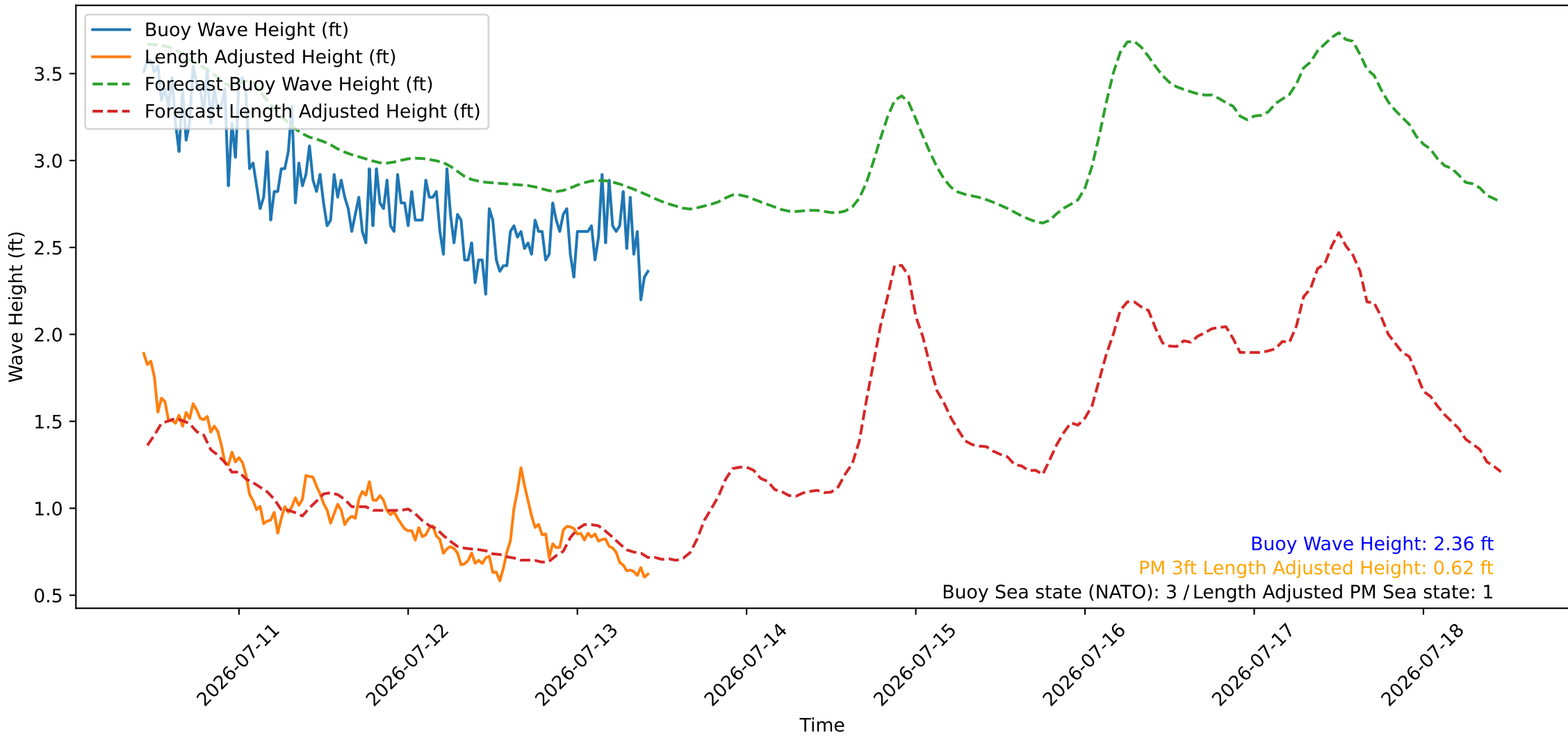
Wave Heights over Time for Green Beach at 2026-07-13 10:41:09
