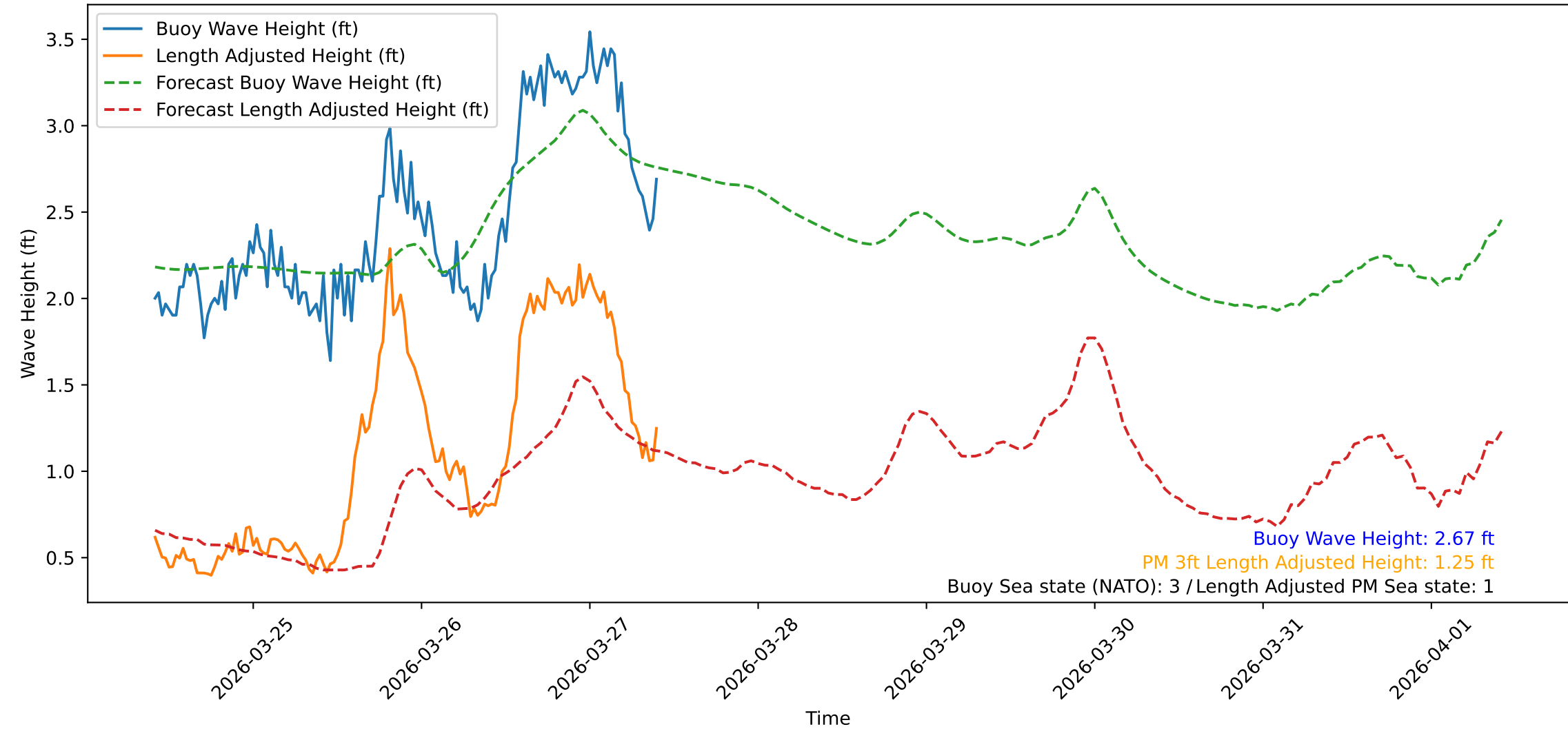
Wave Heights over Time for Green Beach at 2026-03-27 10:11:10
