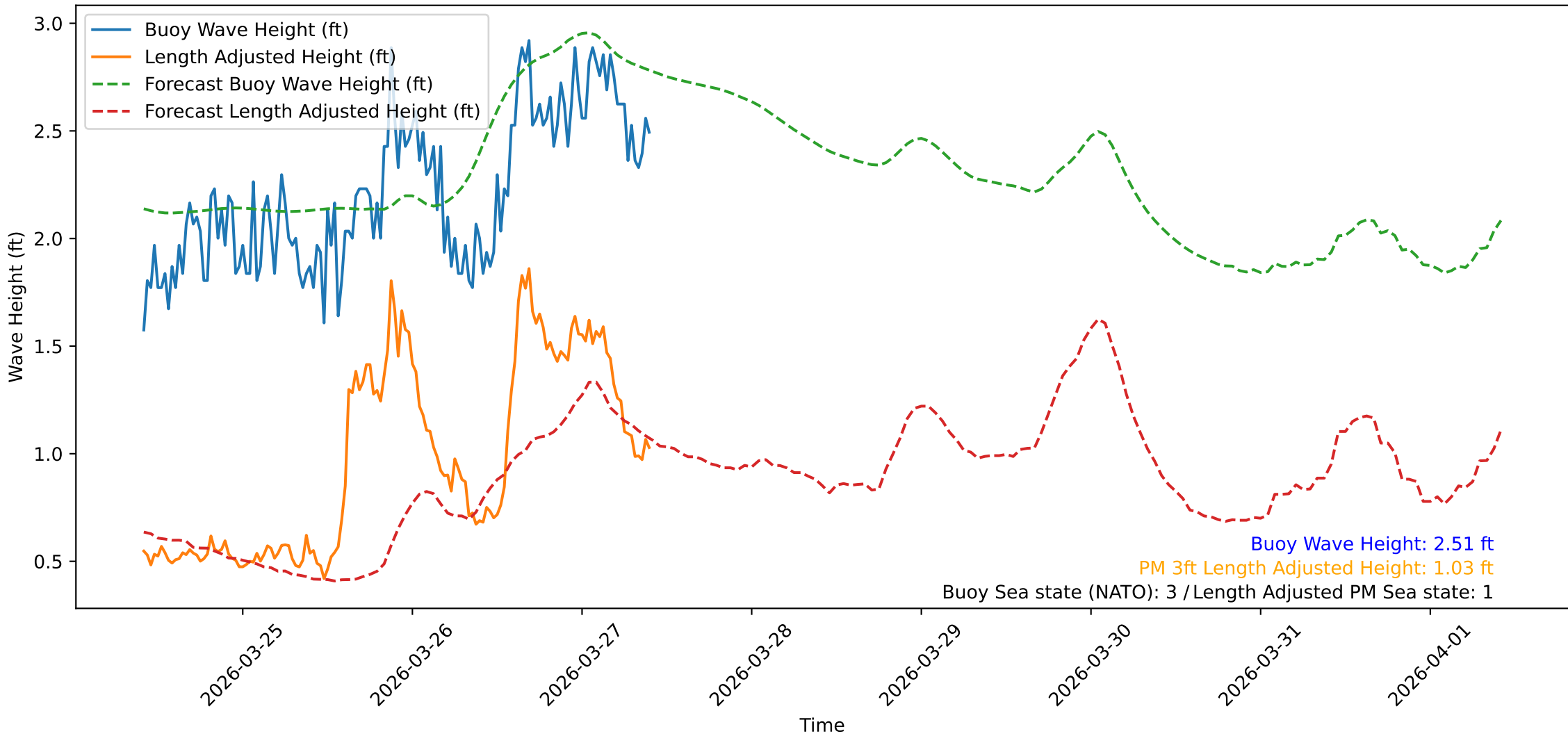
Wave Heights over Time for Oceanside Harbor at 2026-03-27 10:10:31
