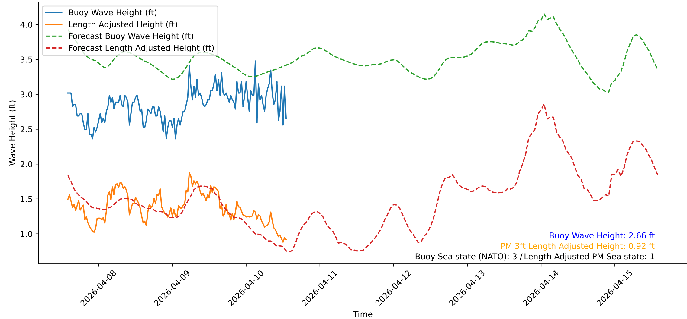
Wave Heights over Time for Green Beach at 2026-04-10 13:51:16
